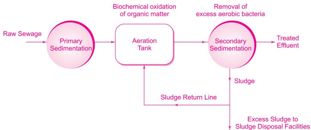
Fig. 3.14 Conventional Activated Sludge Process
