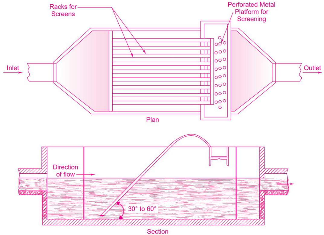
Fig. 3.11 A Typical Bar Screen
