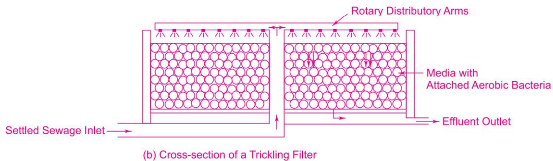
Fig. 3.15 Trickling Filter
