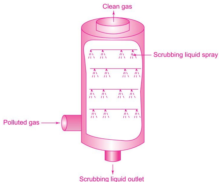
Fig. 3.7 Wet Scrubber
