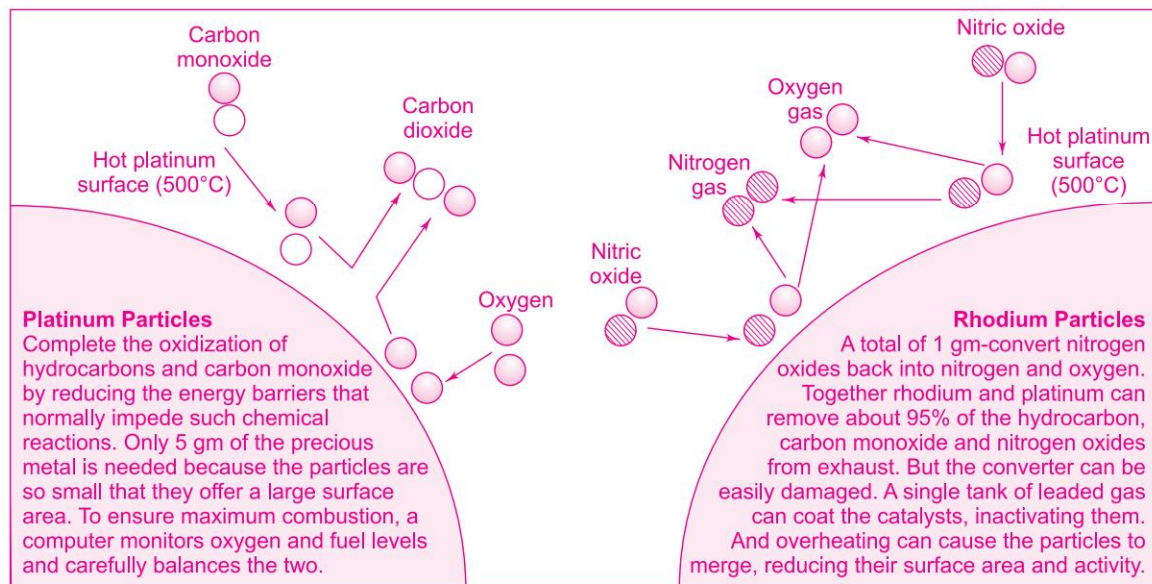
Fig. 3.8 Working of Catalytic Converter
