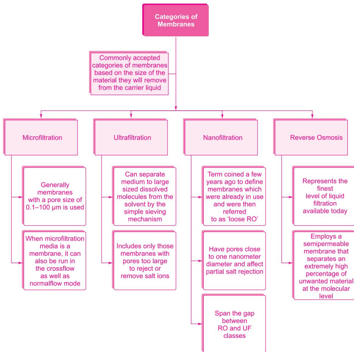
Fig. 3.20 Classification of Membrane Filtration Systems
