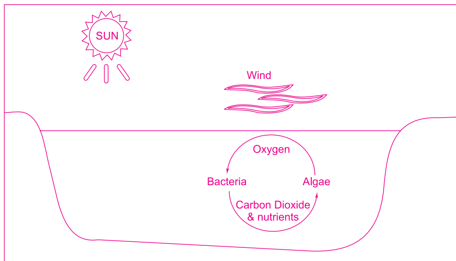
Fig. 3.17 Symbiotic Relation between Algae and Bacteria in Oxidation Pond
