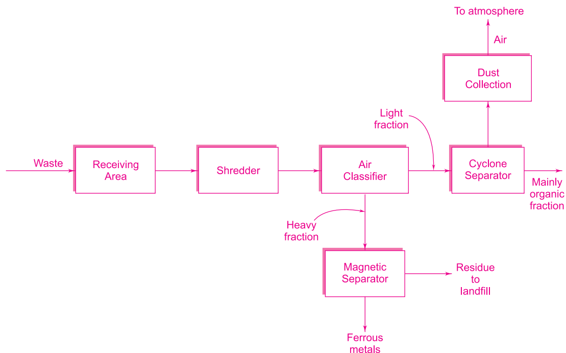
Fig. 3.25 Separation of MSW Components
