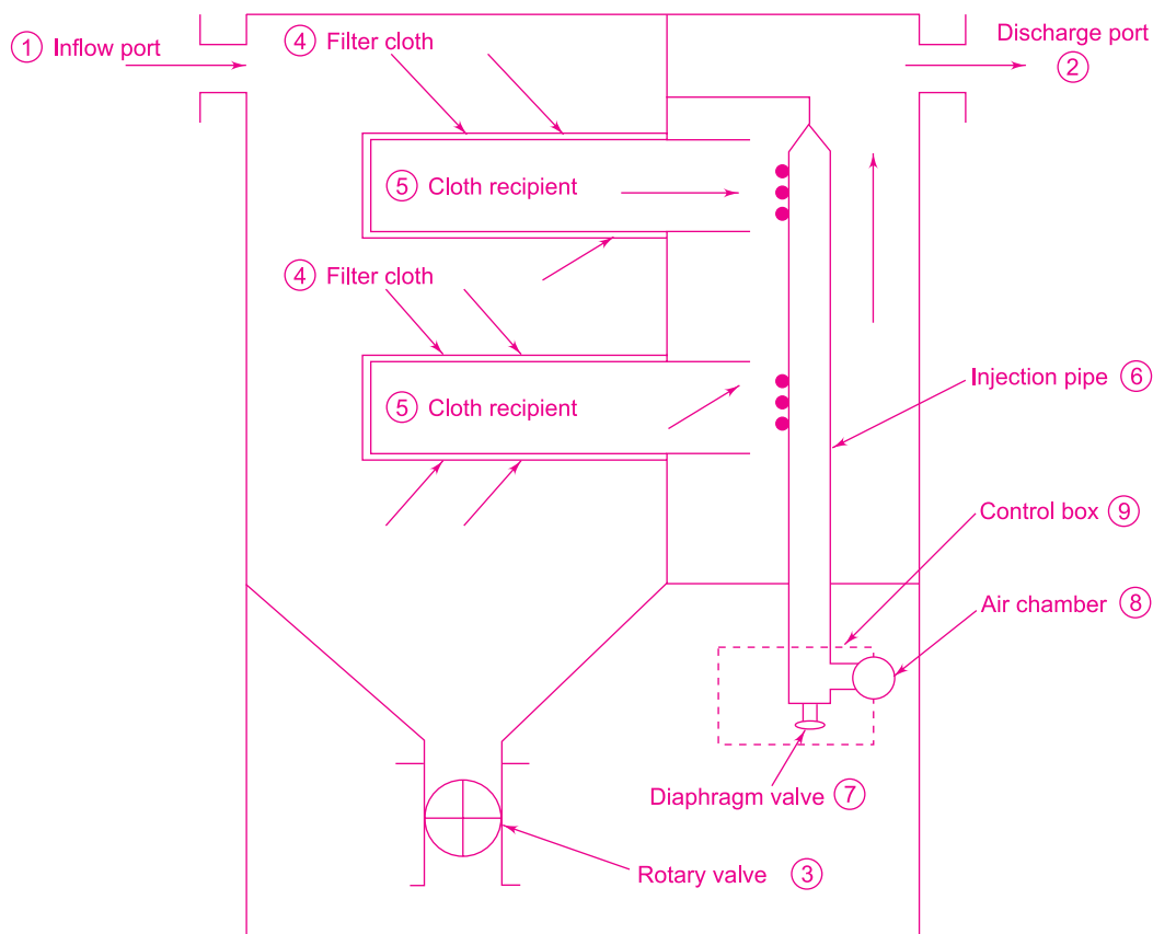
Fig. 3.6 Bag Filter Working
