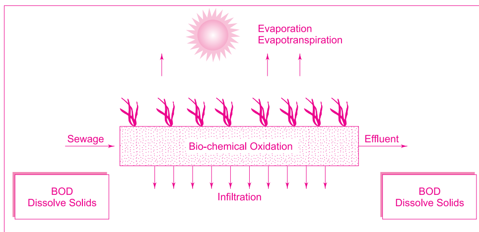
Fig. 3.18 Constructed Wetland
