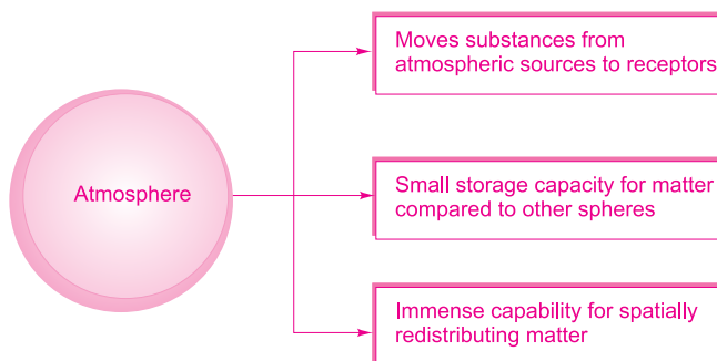
Fig. 1.7(a) Atmosphere
