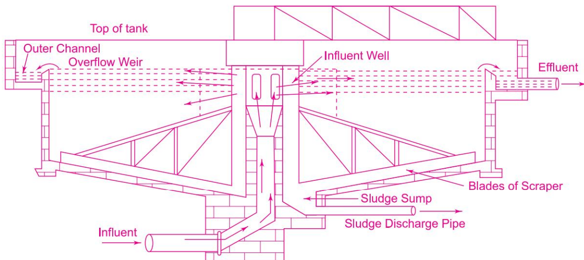
Fig. 3.13 Circular Sedimentation Tank
