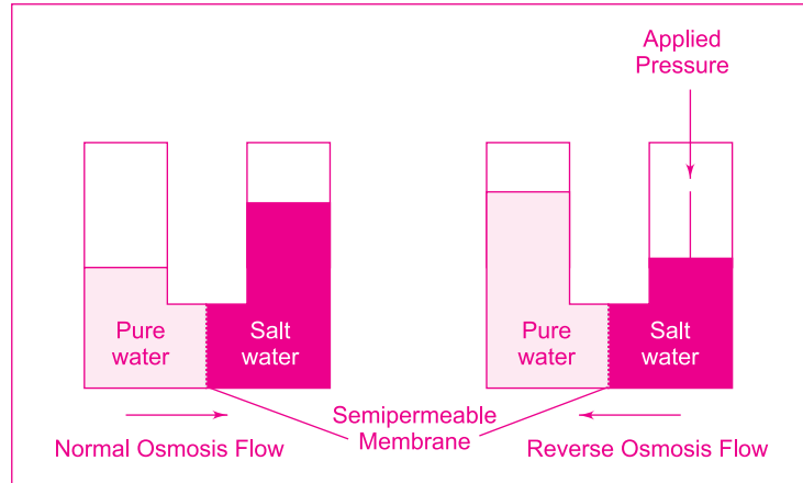
Fig. 3.21 Osmosis Principle
