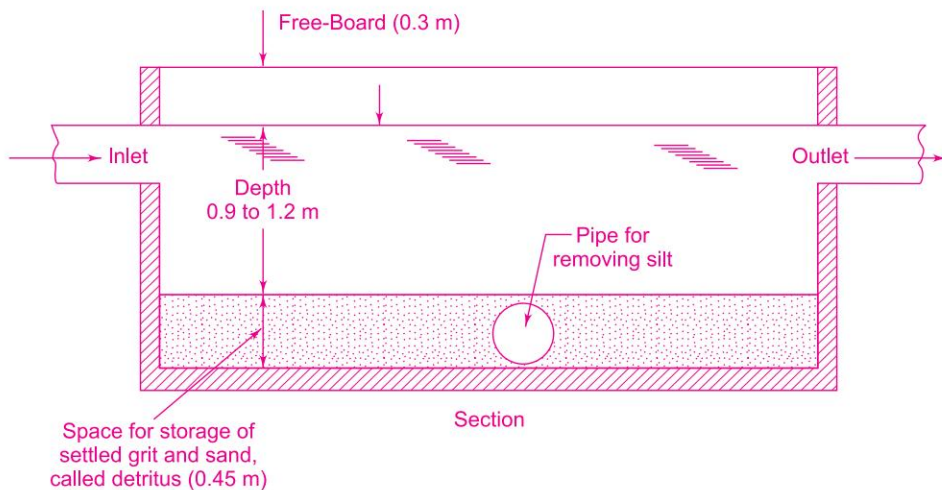
Fig. 3.12 A Typical Grit Chamber used in Sewage Treatment
