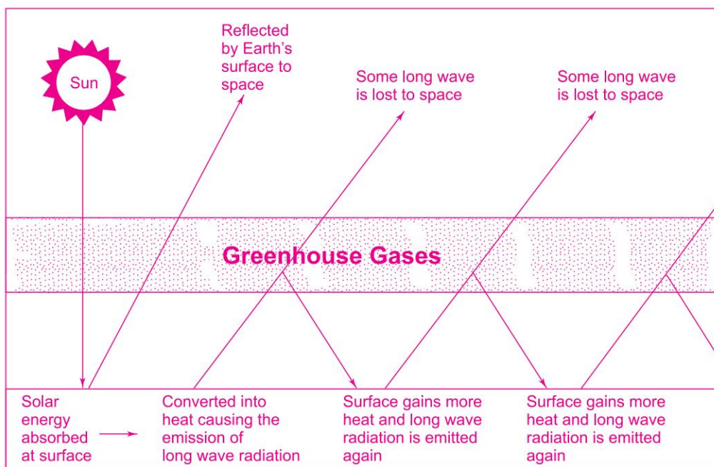
Fig. 5.6 Greenhouse Effect
