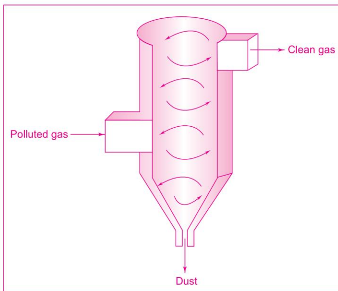
Fig. 3.5 Cyclone Separator
