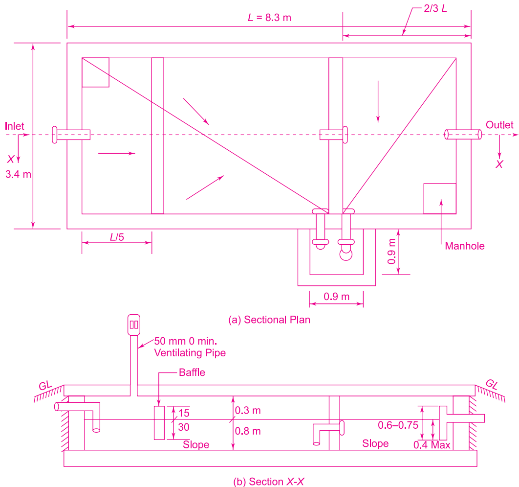
Fig. 3.16 Septic Tank
