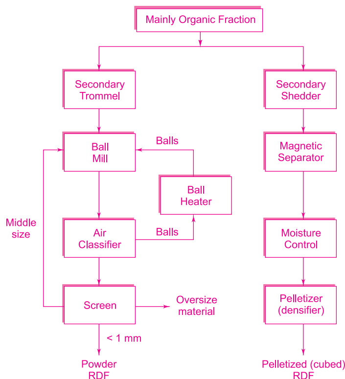
Fig. 3.28 MSW Organic Fraction Processing for Reuse
