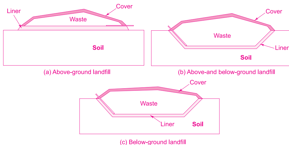
Fig. 3.34 Cross-section of Landfills for Solid Waste Disposal
