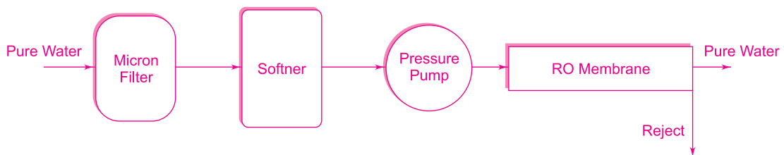
Fig. 3.22 Flow Diagram of Typical Reverse Osmosis Plant for Water Treatment
