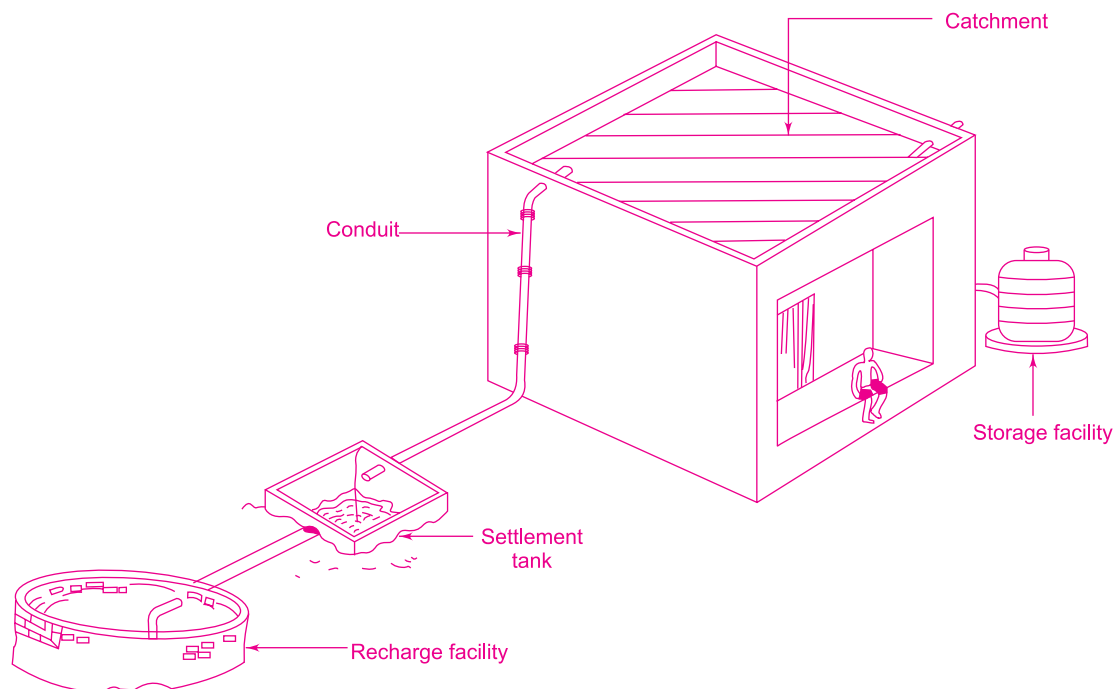
Fig. 5.4 Typical Rainwater Harvesting Facility for a Building
