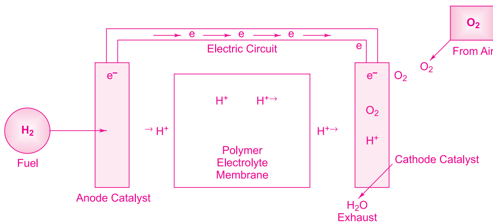
Fig. 4.12 Fuel Cell
