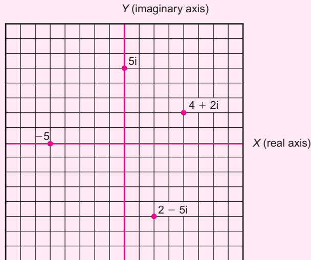
FIGURE 18.48 Four complex numbers shown in the complex plane
