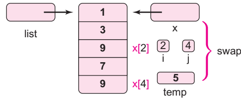
FIGURE 7.18 x[i] = x[j]
