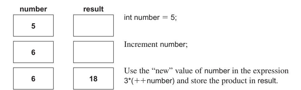
FIGURE 3.6 Prefix operator
