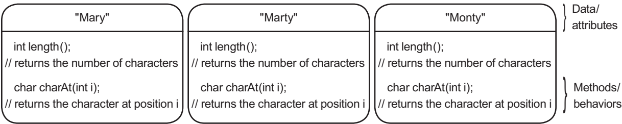
FIGURE 9.4 Three String objects, each with its own data, all with the same methods
