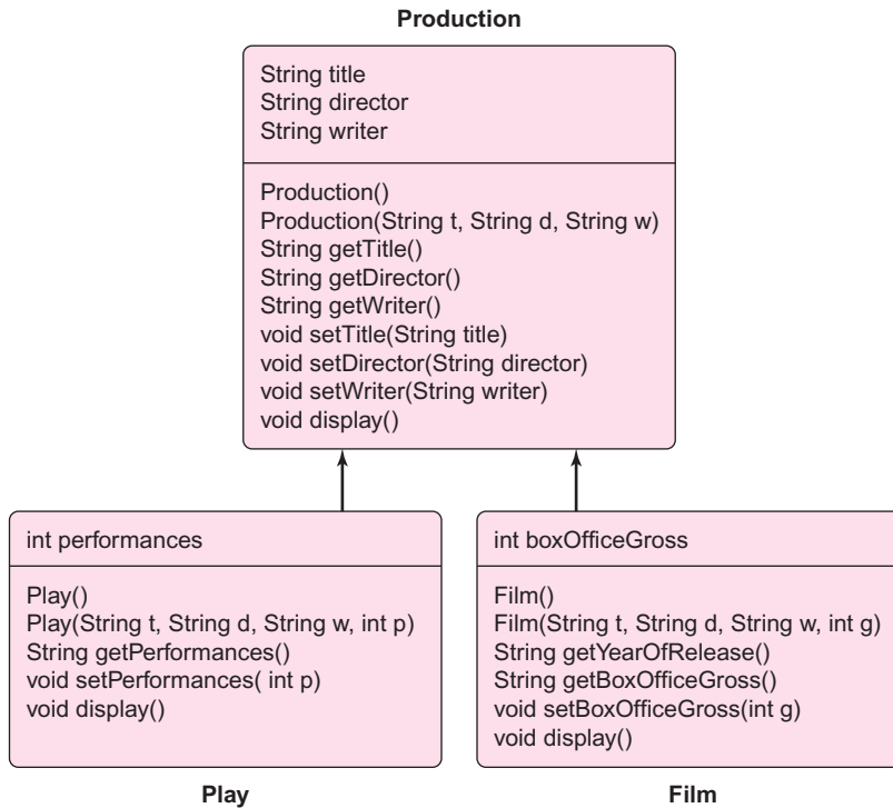
FIGURE 12.5 Play extends Production; Film extends Production
