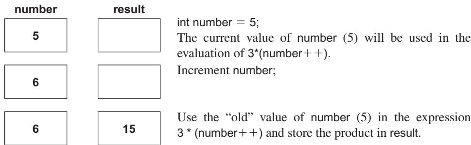
FIGURE 3.7 Postfix operator
