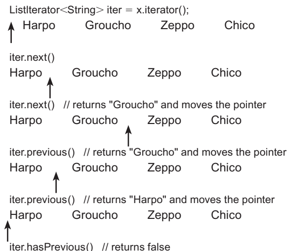
FIGURE 17.10 A ListIterator
