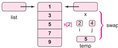
FIGURE 7.17 temp = x[i]
