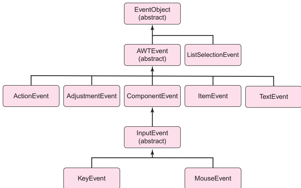
FIGURE 19.2 A partial view of the EventObject hierarchy
