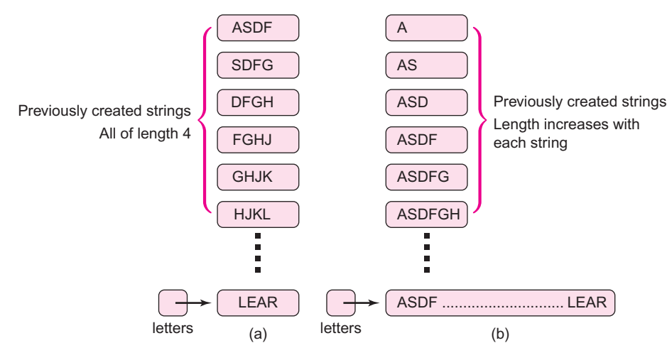
FIGURE 9.20 (a) Strings created with the program of Example 9.3 (b) Strings created using the endsWith() method
