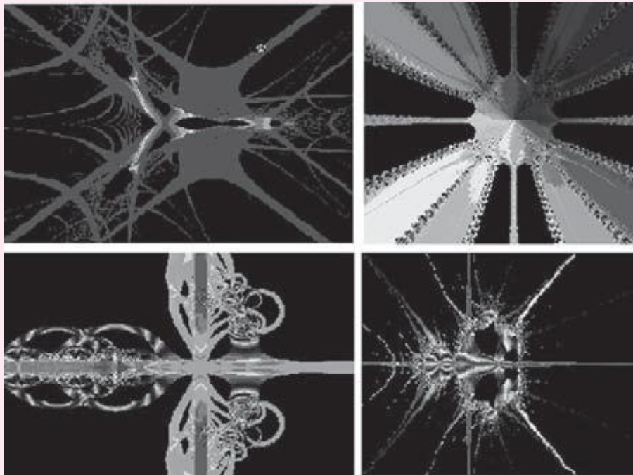
FIGURE 18.44 Some fractals
