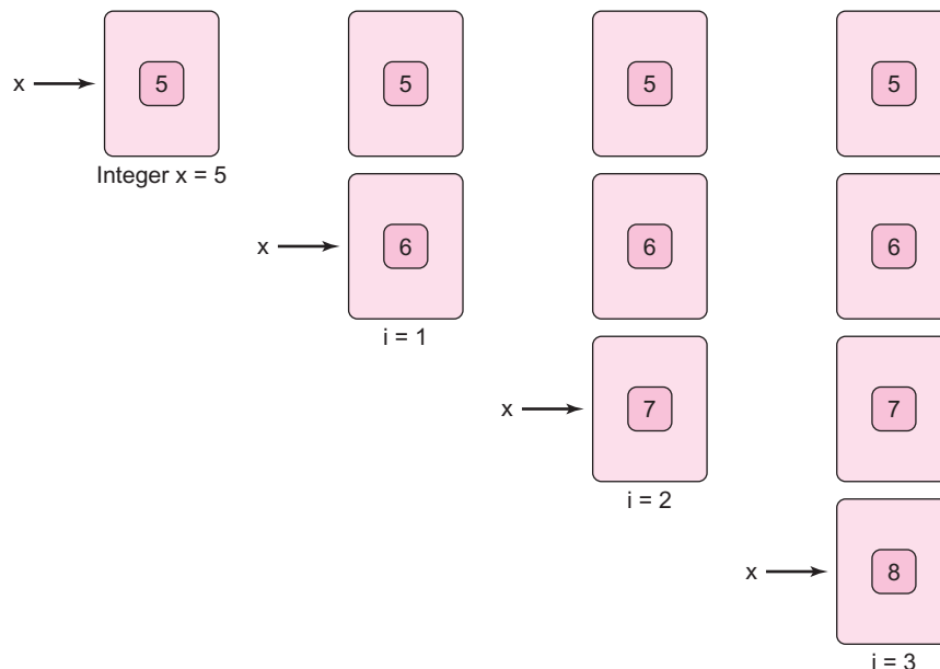
FIGURE 14.5 Wrapper objects are immutable
