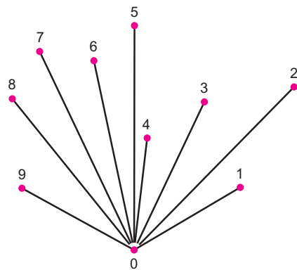
FIGURE 20.16 The points are sorted into counterclockwise order
