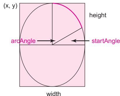
FIGURE 18.22 The arc drawn by the drawArc() method
