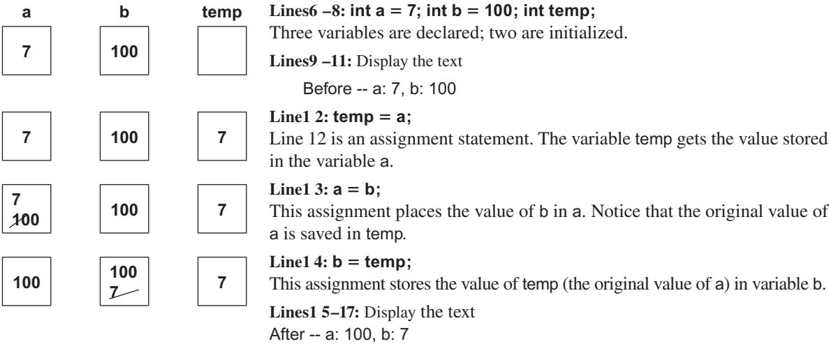
FIGURE 3.4 Swapping the values in two variables
