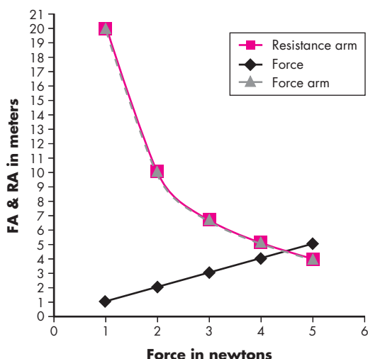
Relationship among Force, Force Arm, and Resistance Arm with Constant Resistance of 20 kilograms
