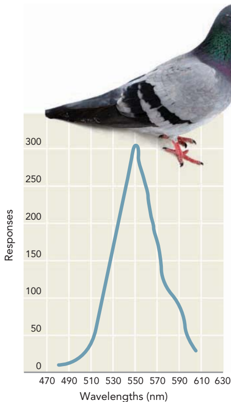
FIGURE 19.5 Stimulus
