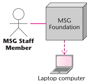
FIGURE 17.26 A deployment diagram.
