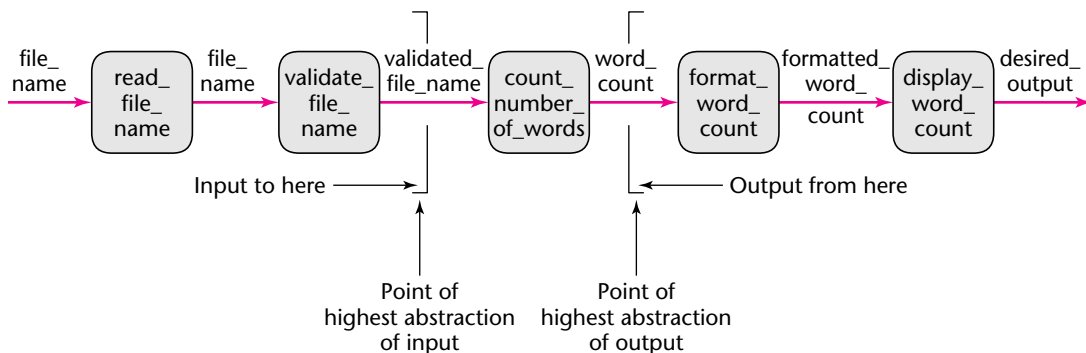
FIGURE 14.3 The first refinement of the data flow diagram.
