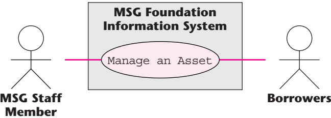
FIGURE 13.39 The Manage an Asset use case.
