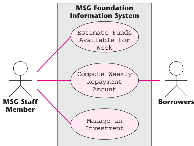
FIGURE 11.13 The use-case diagram of the initial requirements of the MSG Foundation case study.
