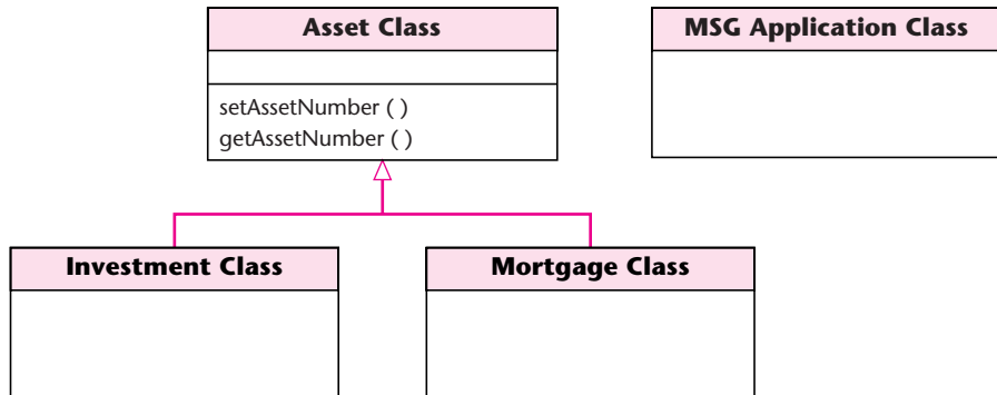
FIGURE 14.15 Part of the class diagram for the MSG Foundation case study with methods setAssetNumber and getAssetNumber assigned to Asset Class .
