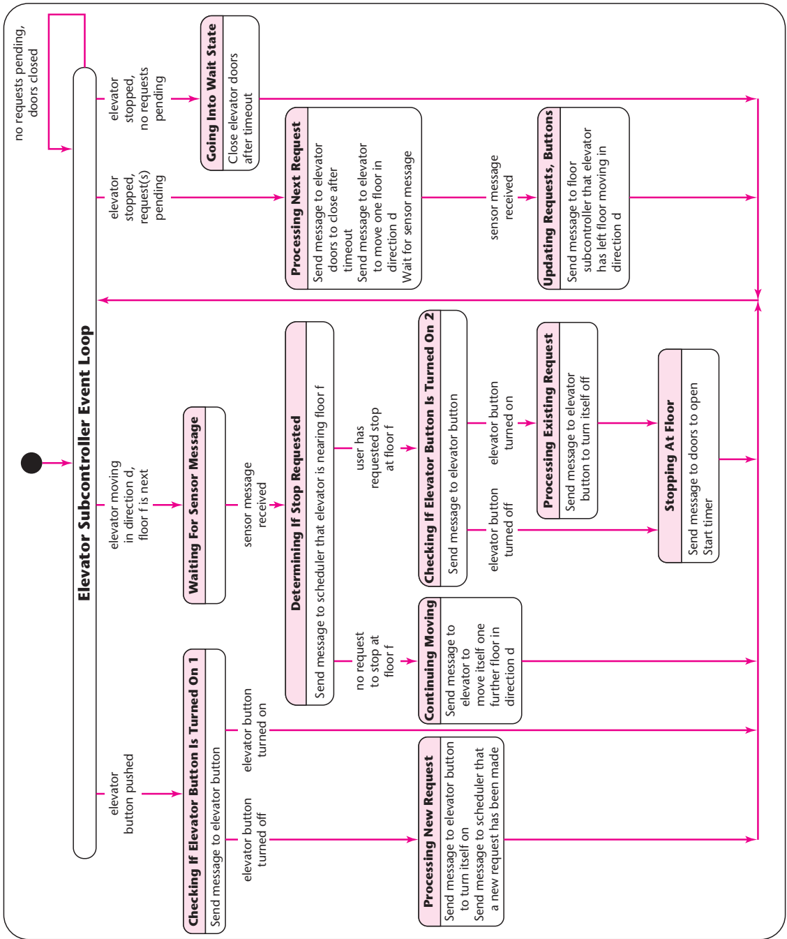
FIGURE 13.13 The first iteration of the statechart for the Elevator Subcontroller Class .
