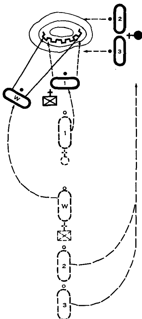
(2) Maneuver right from platoon column (schematic) Figure 76—Continued.
