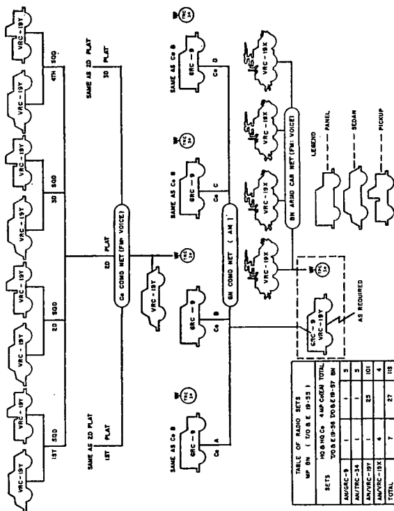
TYPE RADIO NETS MILITARY POLICE BATTALION Figure 6. Radio net diagram, military police battalion (TO/E 19-55A).
