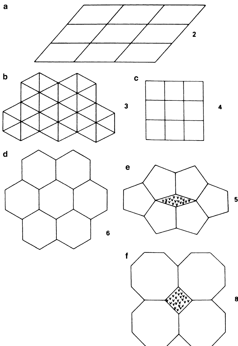
Fig. 1.27 Sections of three-dimensional figures and the rotational symmetries of their smallest structural units; (a–d) Space-filling patterns. In (e) and (f) the v -marks represent voids in the pattern (see also Problem 1.10a)
