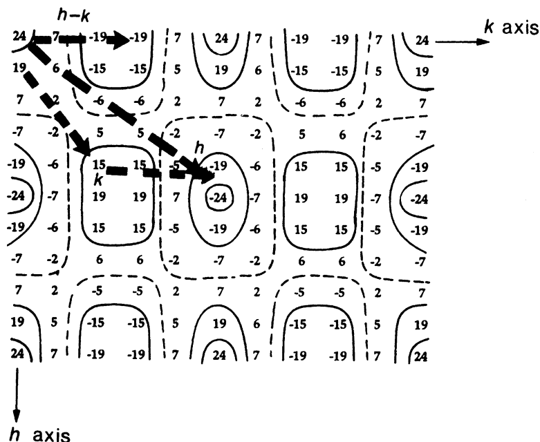
Fig. 6.22 Calculated transform for the four-atom structure (Fig. 6.21a) convolved with its inversion in the origin; contours are shown at -20 , -10 , 10 , and 20 . Fringe systems are apparent, corresponding to the normals to the directions between all pairs of atoms in the four-atom structure (The vectors labeled \mathbf{h} , \mathbf{k} , and \mathbf{h} - \mathbf{k} refer to the discussion in Sect. 6.9.3.)
