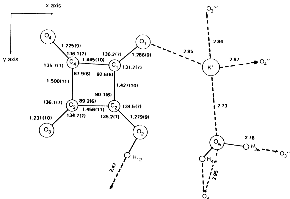
Fig. 9.28 Bond lengths and bond angles in the asymmetric unit of KHSQ; the OH...O distances refer to the overall O...O separations. Primes on atom symbols indicate neighboring asymmetric units; this diagram should be studied in conjunction with Fig. 9.29
