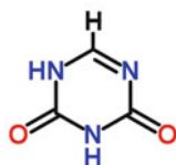
Fig. 8.33 Chemical formula of 5-azauracil, C_4H_4N_4O_2
