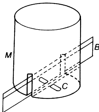
Fig. 5.36 Crystal cutting apparatus: B is a half razor blade, M is a metal or plastic collar and C is the crystal under examination
