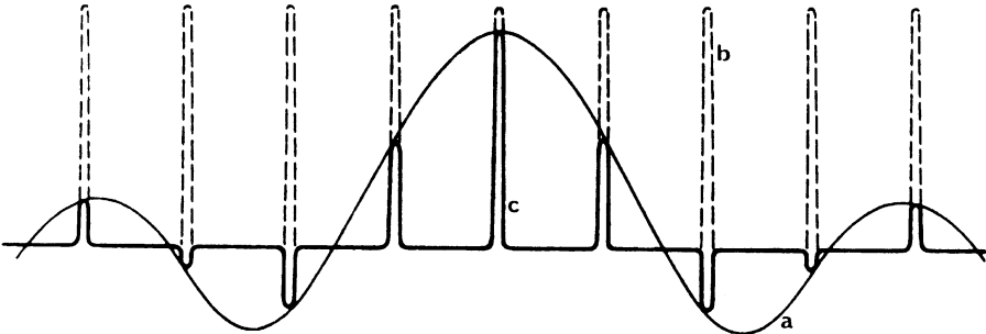
Fig. 6.17 Relationship between amplitudes of diffraction. (a) Single slit of finite width ( thin line ). (b) Ideal slit grating ( dashed line ). (c) Grating of finite-width slits ( bold line ). The transform of the grating of finite-width slits is the convolution of the transforms of the single slit and the ideal grating (reproduced from Taylor and Lipson 1964)
