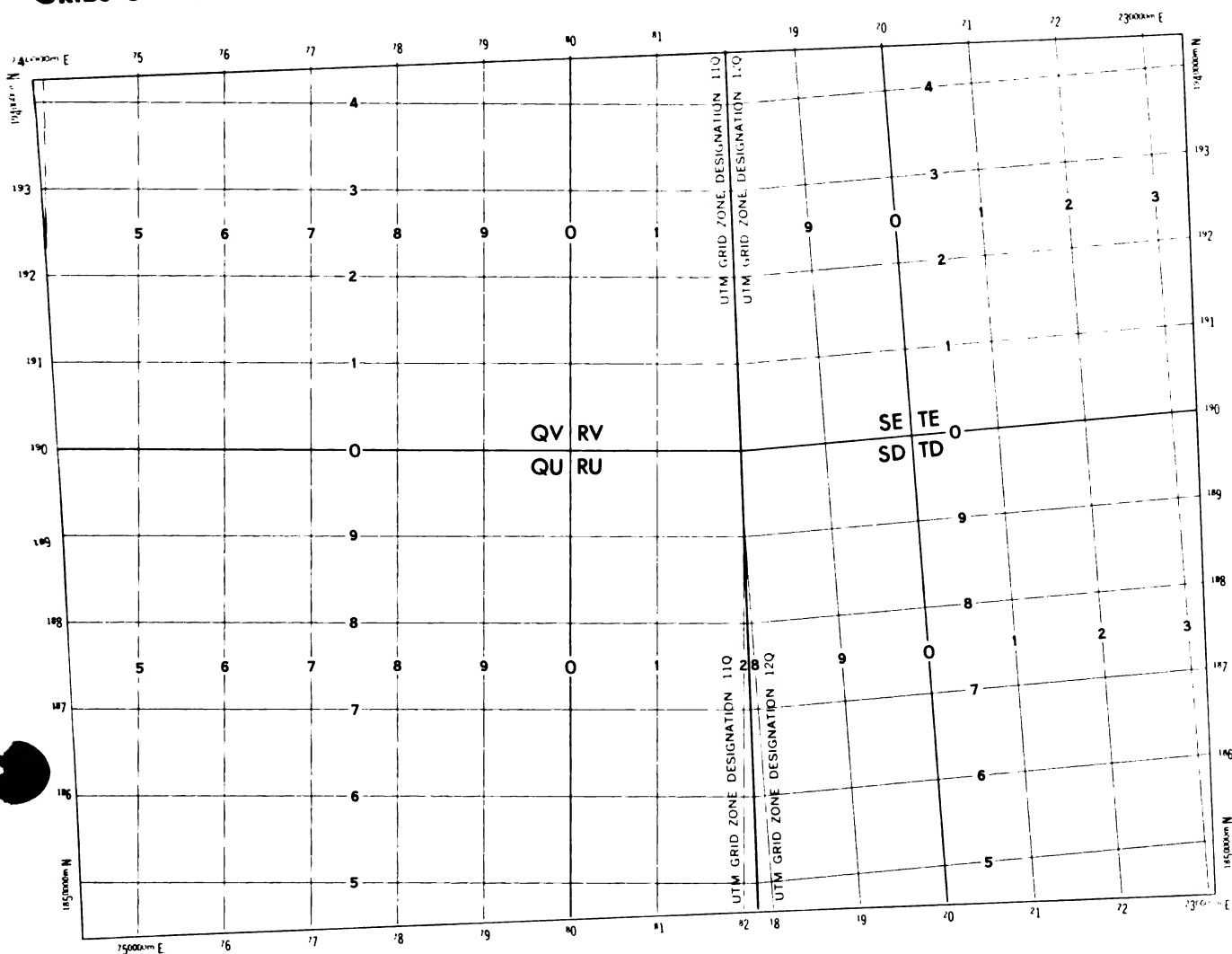
Figure 30. Two major UTM grid zones separated by a grid junction as shown on a 1:250,000 scale map.
