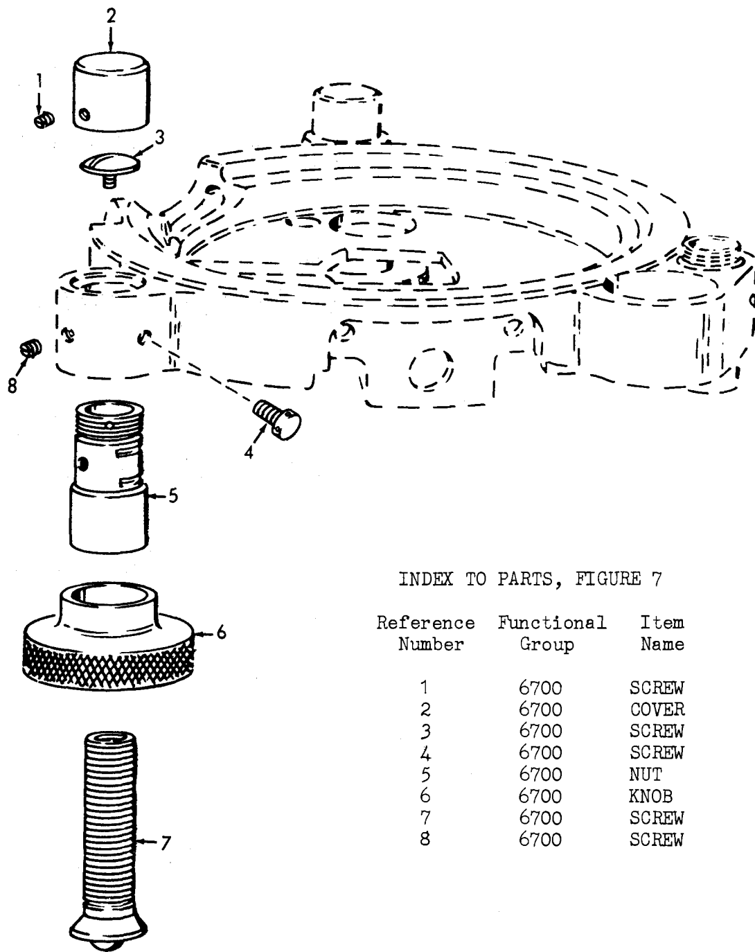
Figure 7. Leveling Screw.
