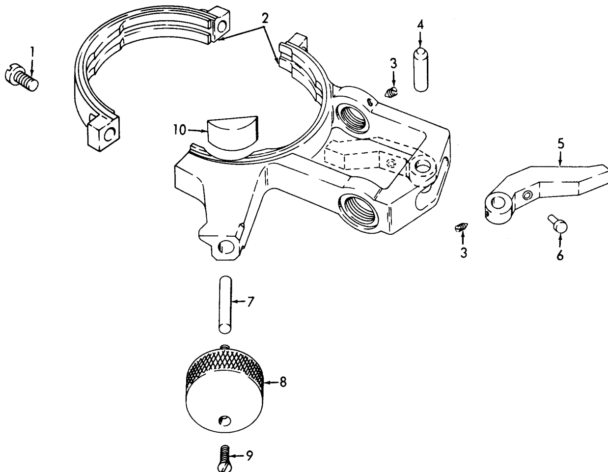
Figure 5. Horizontal Clamp.
