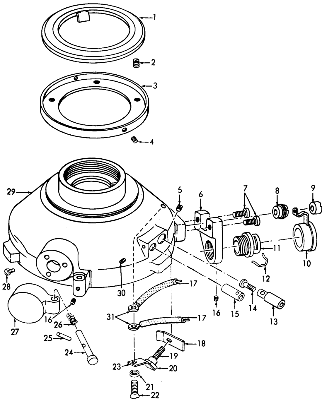
Figure 6. Horizontal Base.
