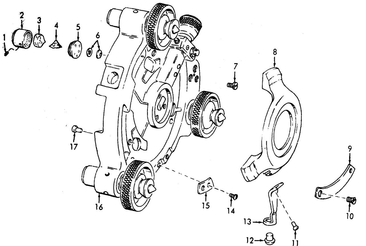
Figure 12. Tribach.
