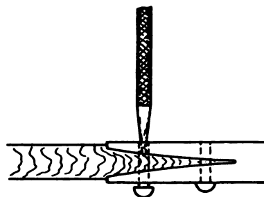
② KNOCK OUT RIVET USING A PUNCH
