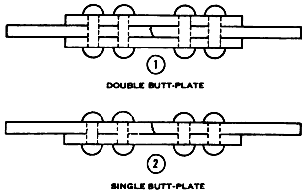
Figure 4-18. Repairing a fracture with butt straps and rivets.
