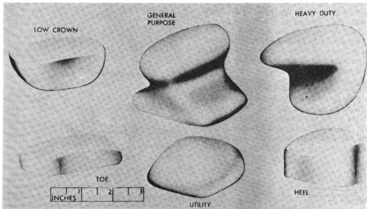
Figure 4-4. Dolly blocks.
