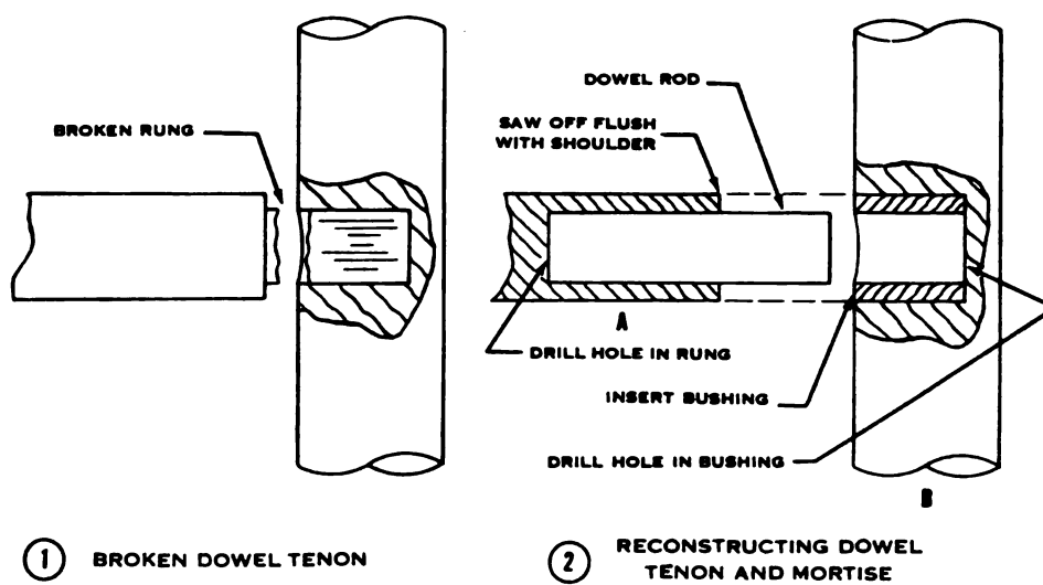
Figure 2-13. Replacing a broken dowel tenon.
