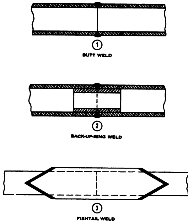
Figure 4-16. Welding tubing.
