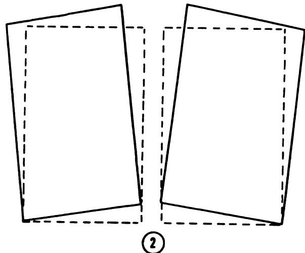
USE OF SPREAD TO BALANCE CONTRACTION
