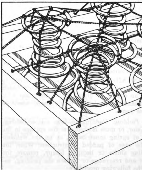
Figure 2-17. Springs tied lengthwise, crosswise, and diagonally.
