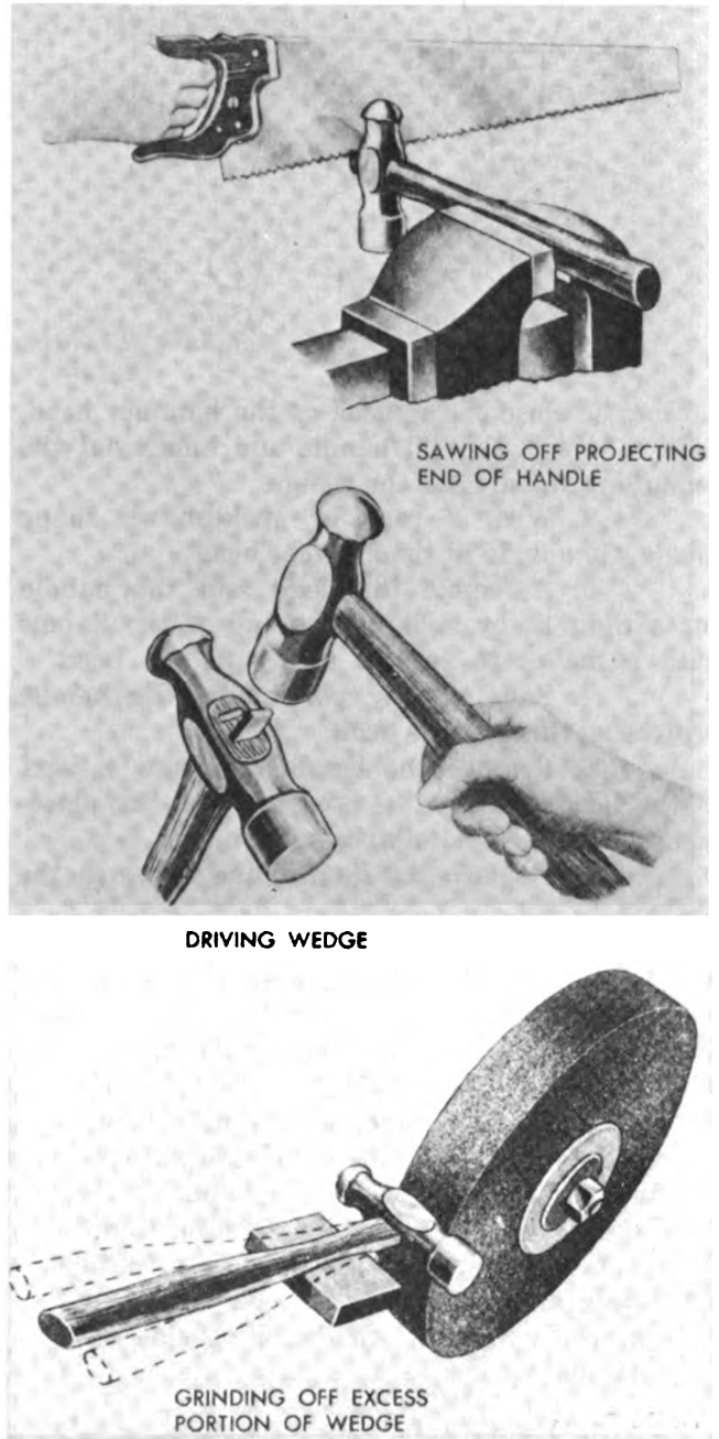
Figure 3-5. Installing wedges.
