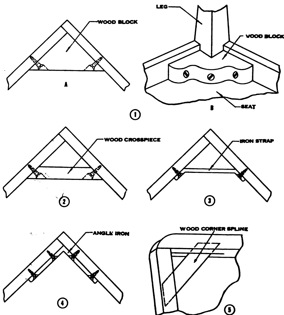
Figure 2-10. Methods of bracing.
