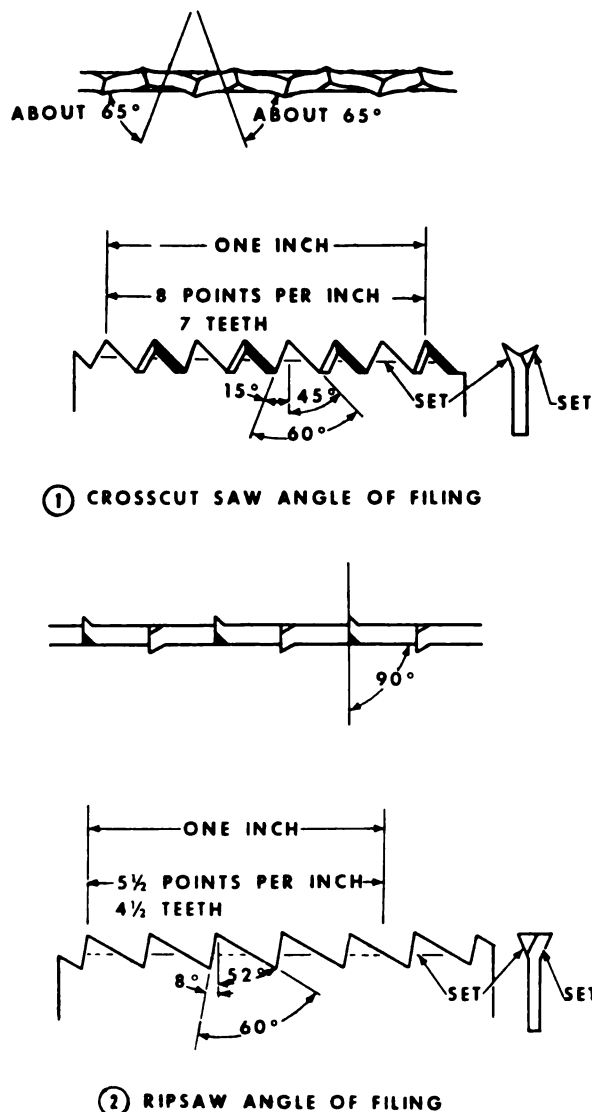
Figure 3-3. Saw setting and sharpening.
