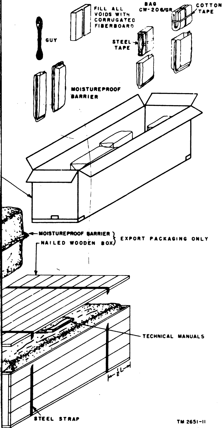
Antenna Group AN/GRA-12.
