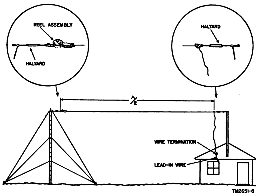
Figure 7. L-type antenna.
