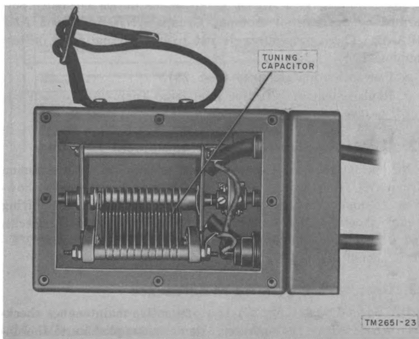
Figure 26. Tuner TN-174/GRA-4, interior view.
