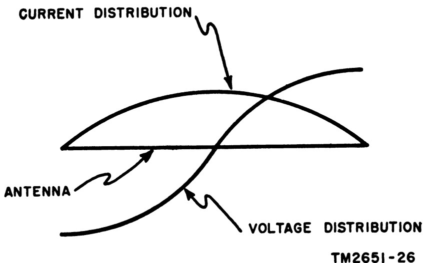
Figure 31. Current and voltage distribution in a half-wave antenna.
