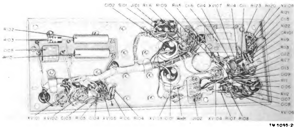
Figure 31. Frequency Meter FR-5/U, power supply, location of parts, bottom view.
