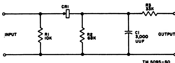
Figure 32. Recommended demodulator schematic diagram.
