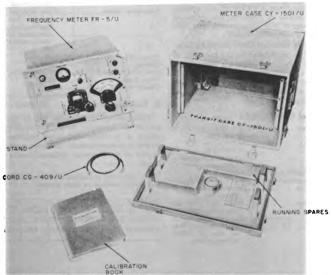
Figure 1. Frequency Meter AN/URM-80.
