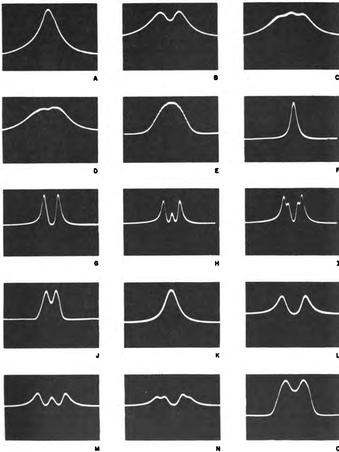
Figure 34. Frequency Meter FR-5/U, wave forms.
