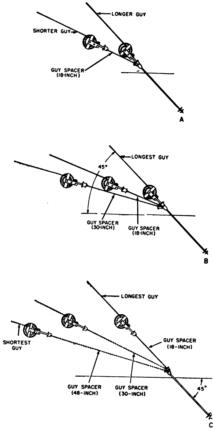
Figure 30. Installation of guy spacers.
