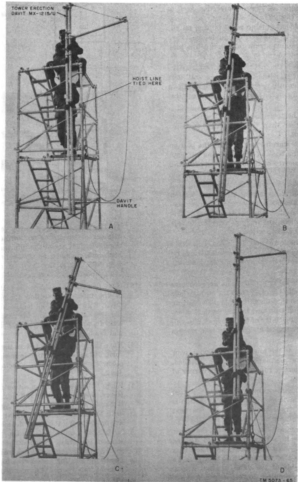
Figure 25. Transferring davit.
