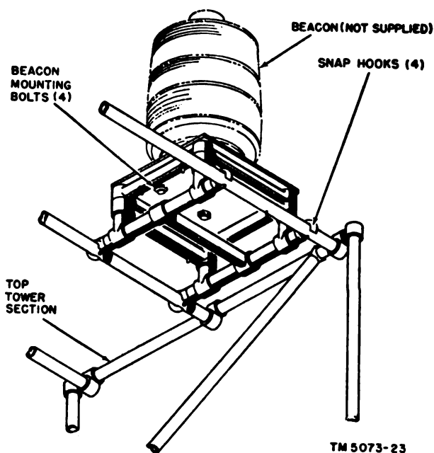
Figure 34. Tower Platform Section MT-1156/U, installed.
