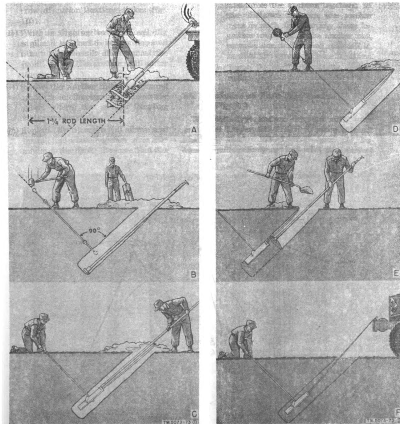
Figure 13. Installation of plate-type anchor.
