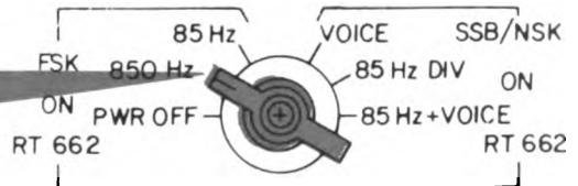
MODE SELECTOR
