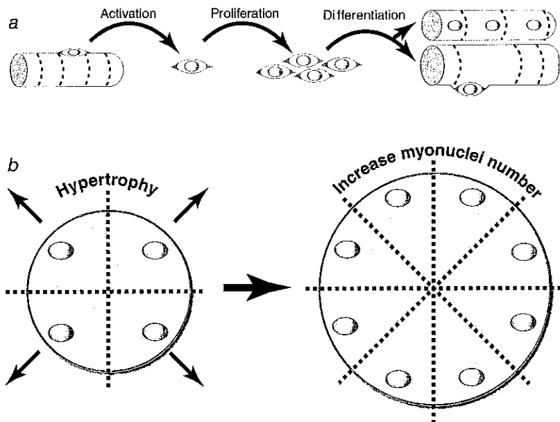
Figure 2.2 The role of satellite cells in muscle growth. (a) When a muscle fiber is damaged during resistance exercise, quiescent satellite cells are activated, causing them to proliferate and differentiate. If damage is relatively minor, as is usually the case following resistance exercise, the satellite cells will fuse to the muscle fiber and donate their nucleus (bottom fiber). This process helps to repair the muscle and allows for growth. However, if there is severe muscle damage, which is rare following resistance exercise, the satellite cells will fuse to one another and generate a new fiber (top fiber). (b) The myonuclear domain theory suggests that nuclei can only “manage” a finite amount of cytoplasm. Therefore, if a muscle is stimulated to grow, the muscle must increase its number of nuclei to “manage” the increase in cytoplasm. The increase in nuclei is donated by satellite cells. Note that each nucleus “manages” the same volume of cytoplasm before and after muscle growth.
