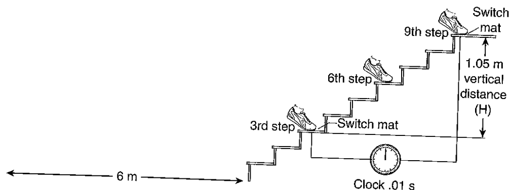
Figure 5.4 The Margaria-Kalamen stair sprint test is a simple method for assessing your level of power relative to others in your age group.
