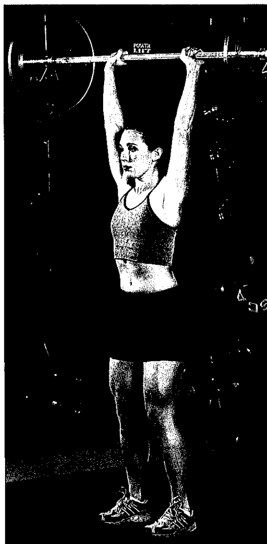
Figure 6.2 Isotonic exercises such as this barbell overhead press can condition your body to more easily perform everyday activities.
