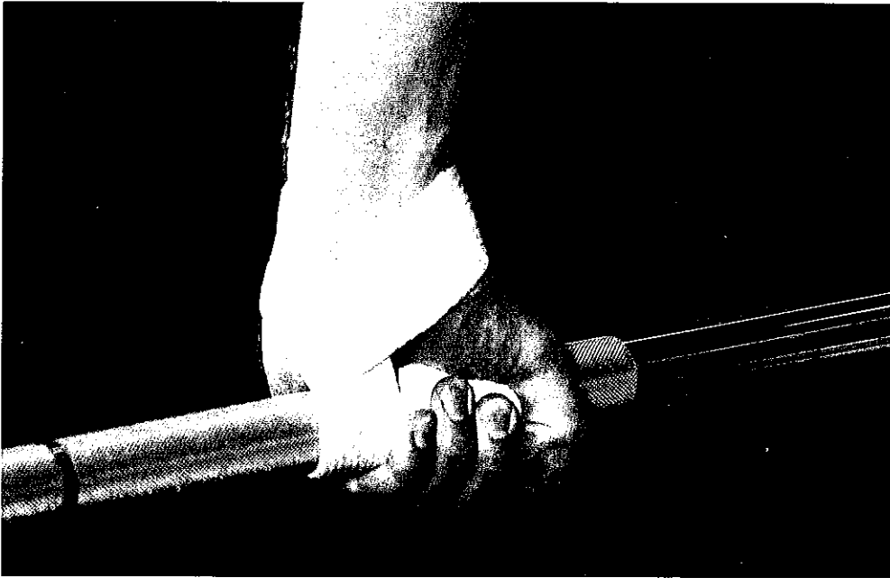
Figure 8.3 The closed grip is shown here using lifting straps. Notice that the thumb wraps around the bar to prevent slippage.
