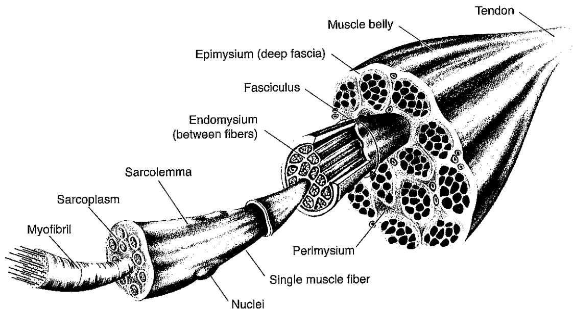
Figure 1.1 Tendons attach the muscles to the bones allowing muscles to cause movement. The intact whole muscle is made up of bundles of muscle fibers, each with a connective tissue sheath surrounding it. A muscle fiber is made up of myofibrils, which contain many different contractile proteins. The key contractile proteins in the myofibrils of the muscle are actin and myosin.
