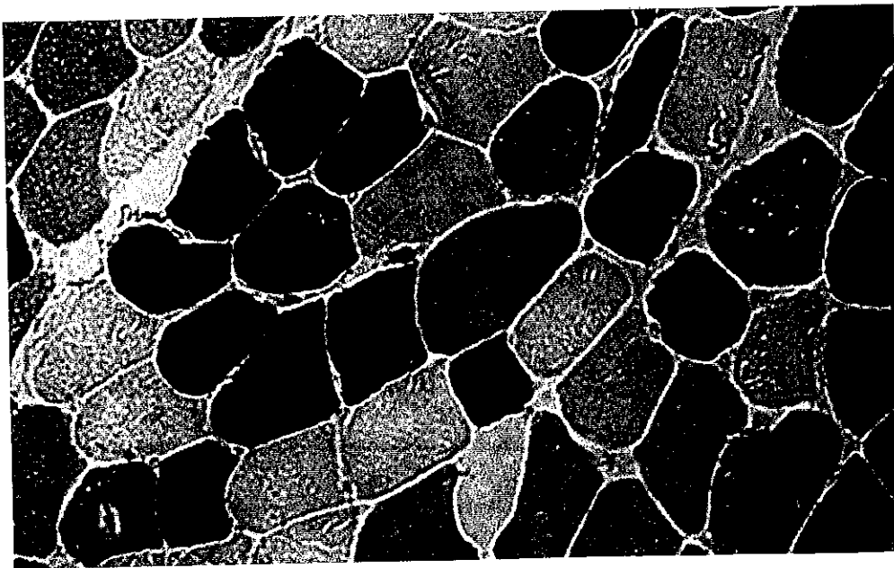
Figure 1.3 Muscles can be artificially stained in the laboratory to produce different color fibers in order to classify what percentage of Type I and Type II muscle fibers exist in the muscle. In this picture, Type I muscle fibers are black, and Type II muscle fibers are light gray (Type IIA) and dark gray (Type IIX).
