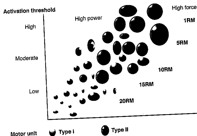
Figure 1.10 Recruitment of motor units (alpha motor neuron and the associated muscle fibers—depicted as circles) occurs based on size. Small motor units are recruited first, going up to larger motor units that produce high force and power. Some people do not have many fast-twitch, or Type II, motor units; also, if not stimulated with resistance exercise, these motor units can be lost with age. The force requirement needed to stimulate motor units varies.
