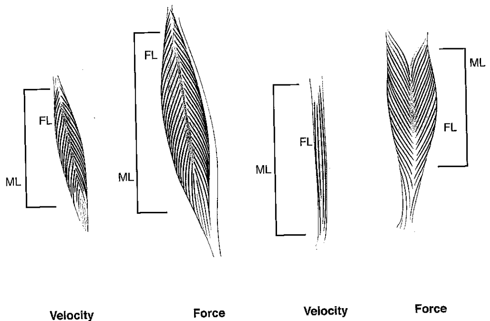
Figure 1.9 Pennation angle, muscle fiber length (FL), and muscle length (ML) for muscles with either high-force or high-velocity functions. Relatively long muscle fibers make the muscle well suited for high-velocity movements; relatively short fibers arranged in parallel make the muscle well suited for high-force movements.
