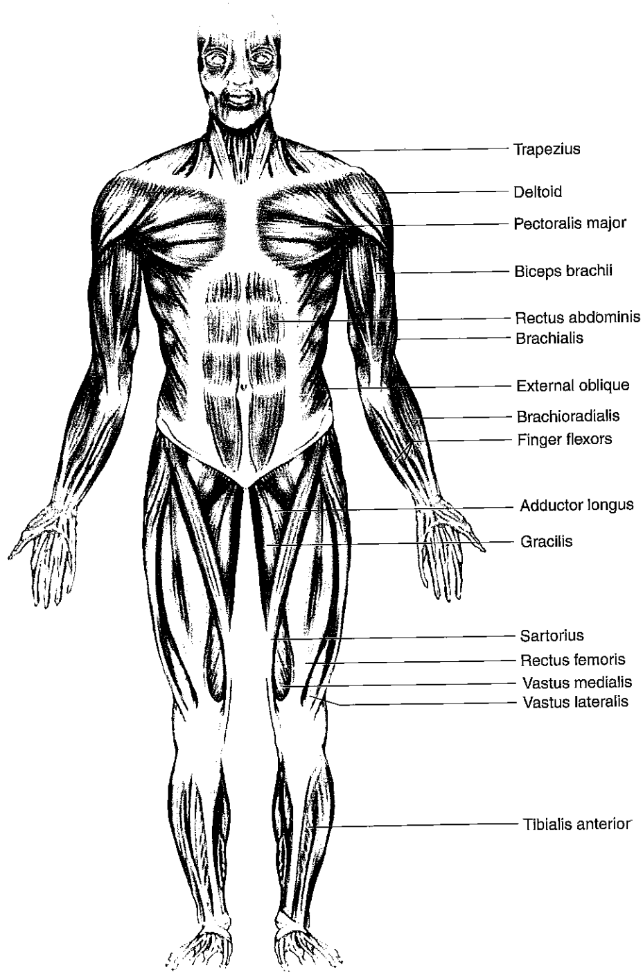
Figure 1.4a Major muscles of the body; front view.
