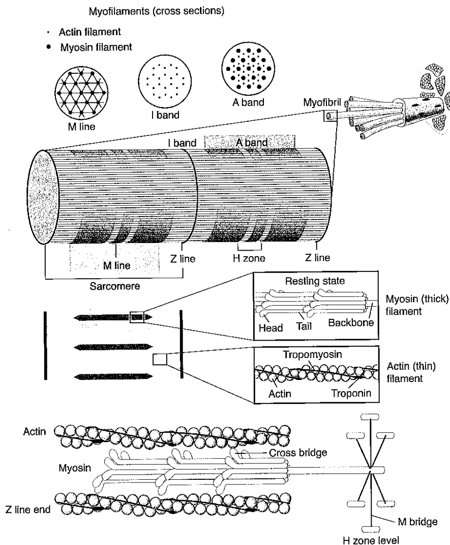
Figure 1.2 The sarcomere runs from Z line to Z line and is the basic contractile unit of the muscle. The interactions of the actin and myosin create force production that causes the muscle to contract.
