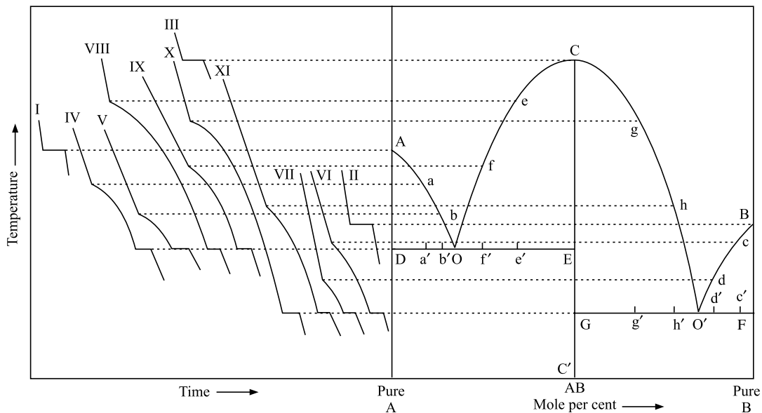
Fig. 6.6.1 Phase diagram of a system exhibiting a congruent melting point
