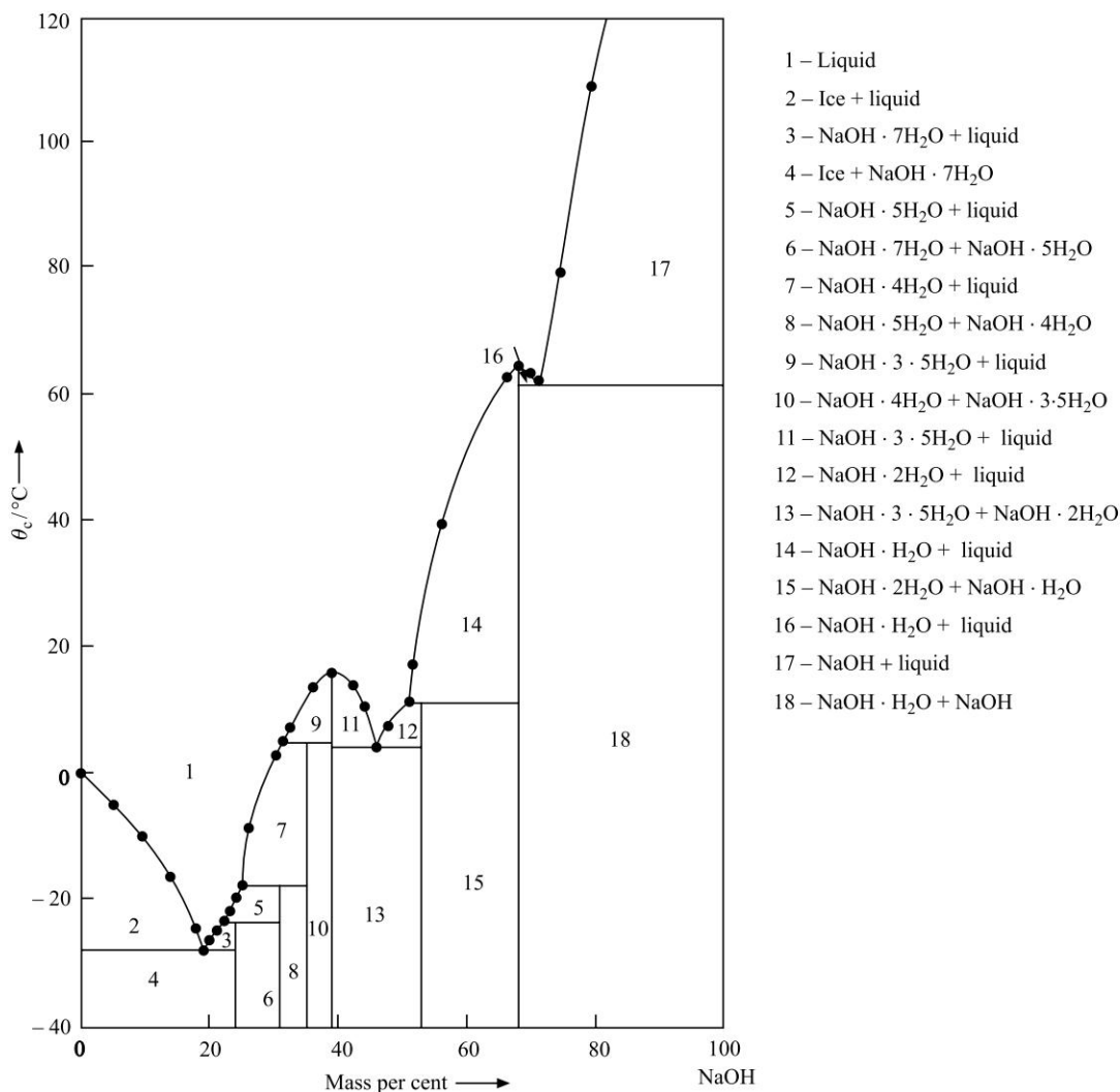
Fig. 6.12.6 Required phase diagram of \text{NaOH} - \text{H}_2\text{O} system
