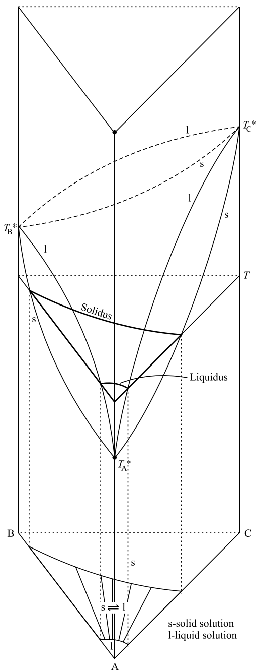
Fig. 7.10.2 Triangular plot for a system exhibiting three pairs A-B, B-C and C-A of solid solutions with T_C^* > T_B^* > T > T_A^*
