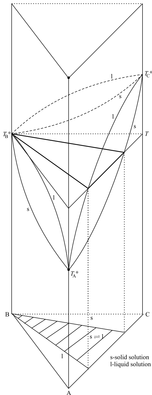
Fig. 7.10.3 Triangular plot for a system exhibiting three pairs A-B, B-C and A-C of solid solutions with T_C^* > T_B^* = T > T_A^*
