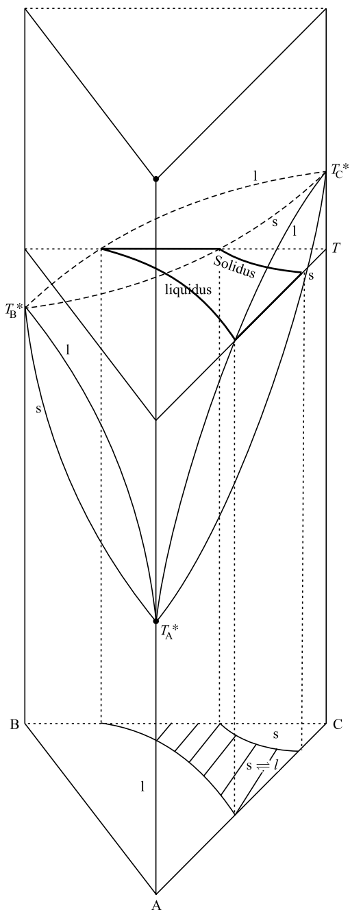
Fig. 7.10.4 Triangular plot for a system exhibiting three pairs A-B, B-C and A-C of solid solutions with T_C^* > T > T_B^* > T_A^*
