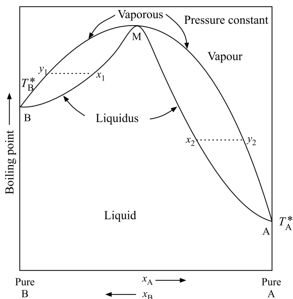
Fig. 4.16.2 Temperature-composition diagram for a system exhibiting a maximum in boiling point
