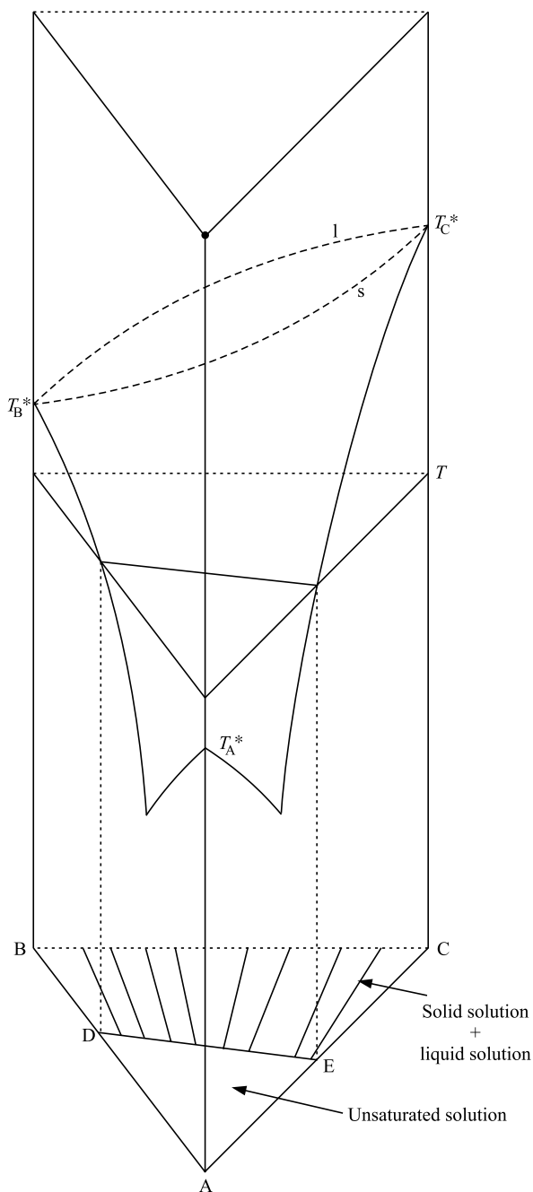
Fig. 7.10.1 Triangular plot for a system exhibiting only one pair B-C of solid solution
