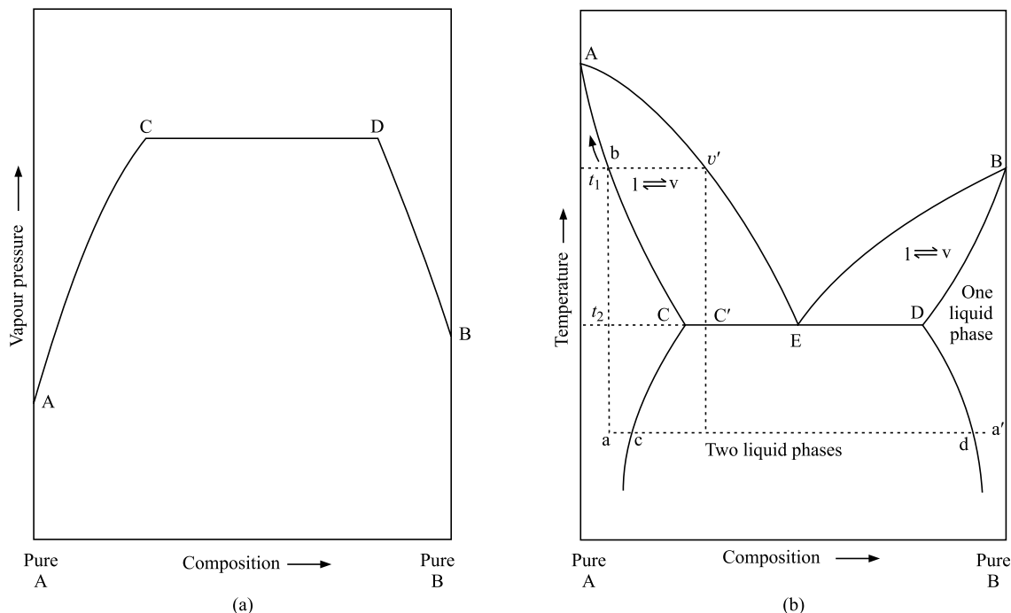
Fig. 4.18.8 (a) Vapour pressure-composition and (b) temperature-composition diagrams for partial miscible liquids with no azeotropic mixture
