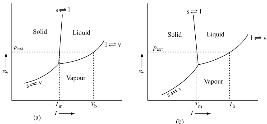
Fig. 1.5.2 Phase diagrams (a) carbon dioxide where V_{m,1} > V_{m,s} and (b) water where V_{m,1} < V_{m,s}
