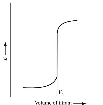
Fig. 8.18.4 A typical potentiometric titration curve
