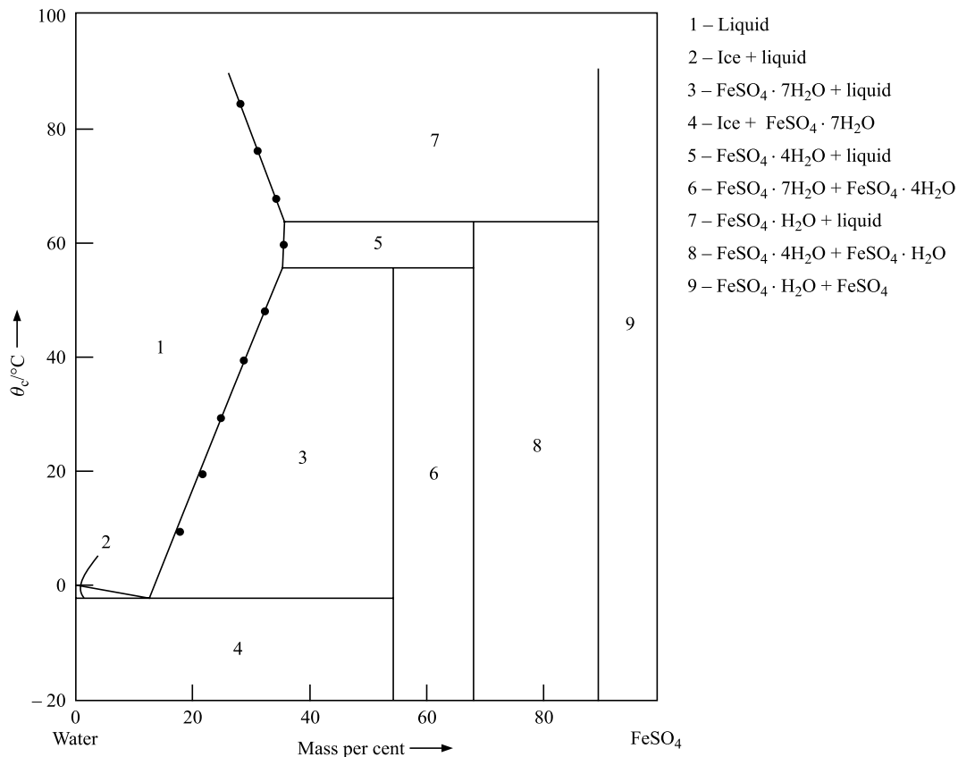
Fig. 6.12.5 Required phase diagram of \text{FeSO}_4\text{-H}_2\text{O} system
