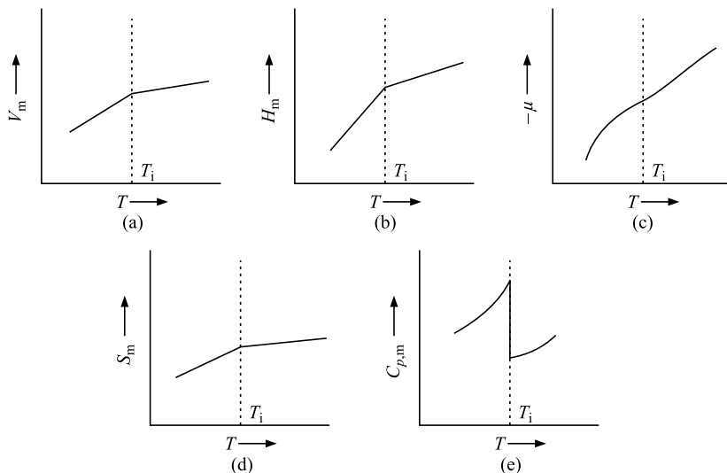
Fig. 1.6.2 Typical variations of (a) V_m versus T , (b) H_m versus T , (c) -\mu versus T , (d) S_m versus T , and (e) C_{p,m} versus T of second-order transition
