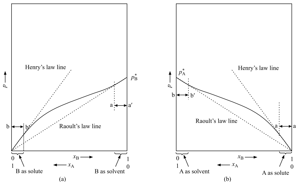
Fig. 4.4.1 Schematic graphs indicating applicability of Henry's law to the solute and Raoult's law to the solvent. (a) For liquid B and (b) for liquid A.
