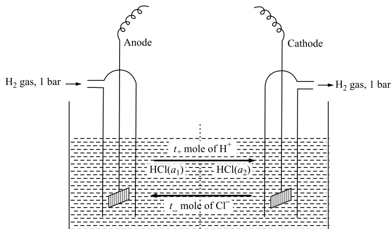
Fig. 8.21.1 Cell in which electrodes are reversible with respect to cations
