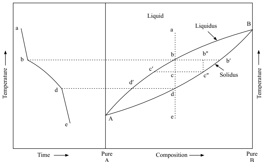
Fig. 6.8.1 Phase diagram for a system exhibiting continuous series of solid solutions with no maximum or minimum
