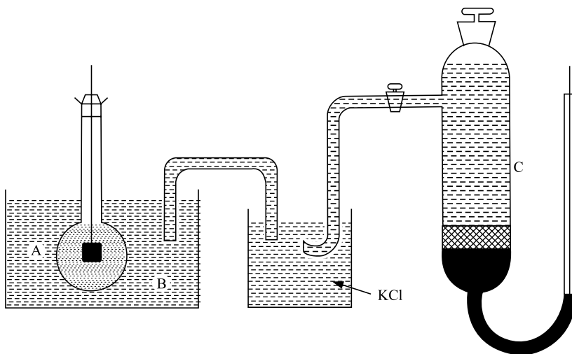
Fig. 8.18.3 Determination of pH of the solution with the cell containing glass electrode
