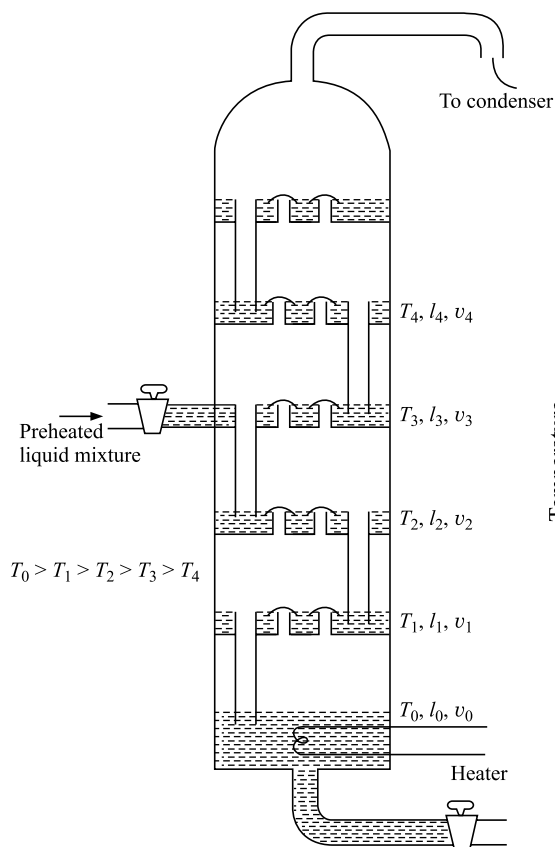
Fig. 4.13.3 Bubble-cap distilling column
