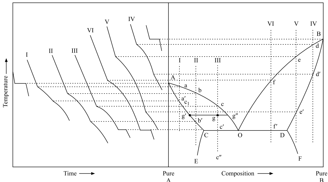
Fig. 6.9.1 Phase diagram exhibiting partial miscibility in the solid state with the eutectic point
