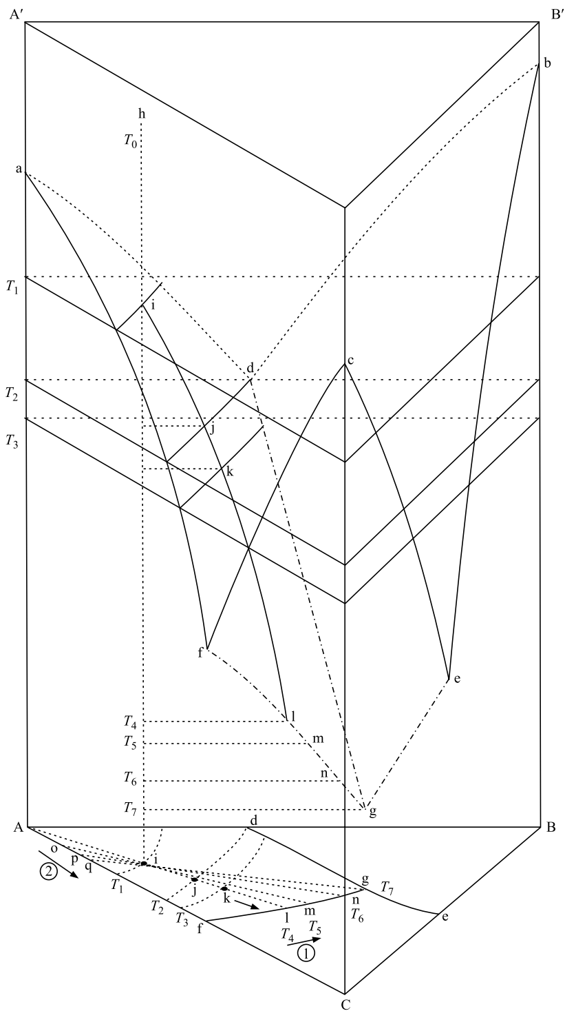
Fig. 7.4.10 The sequence of effects produced on cooling a ternary system. The tie-lines are as follows. Ai at T_1 , Aij at T_2 , Aik at T_3 , Ail at T_4 , oim at T_5 , pin at T_6 , and qig at T_7 . The arrows 1 and 2 indicate the directions of change in compositions of liquid and solid phases, respectively.
