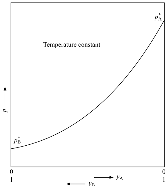
Fig. 4.9.2 Plot of p against y_A , the composition of A in vapour phase
