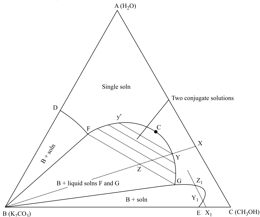
Fig. 7.12.1 Triangle plot for the system \text{H}_2\text{O} – \text{K}_2\text{CO}_3 – \text{CH}_3\text{OH}
