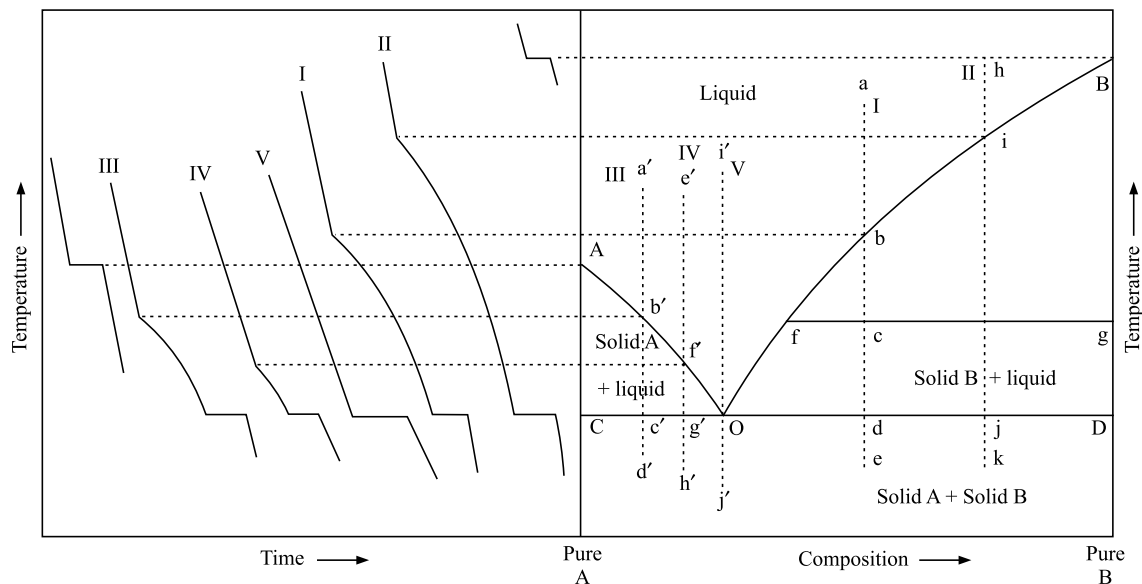
Fig. 6.4.1 Phase diagram of a system exhibiting crystallization of pure components
