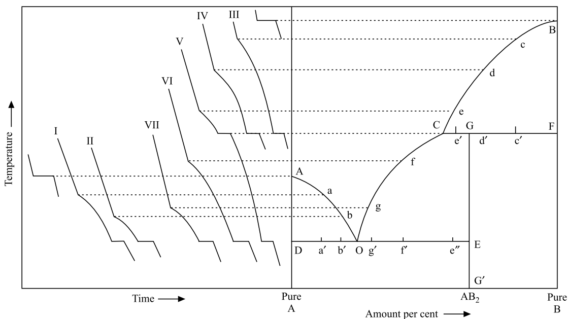
Fig. 6.7.1 Phase diagram of a system exhibiting the formation of an incongruent compound AB_2
