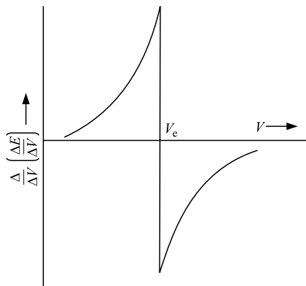
Fig. 8.18.6 A typical second derivative graph
