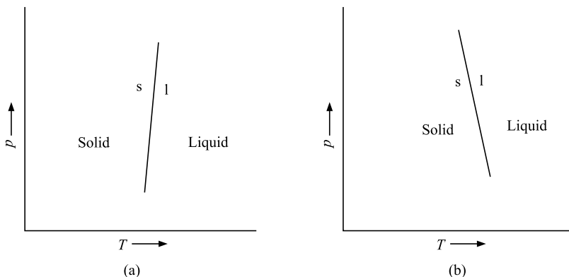
Fig. 1.5.1 Plot of p versus T for solid-liquid equilibrium, when
