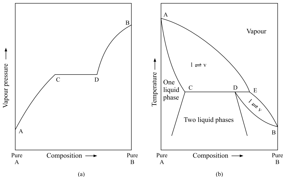
Fig. 4.18.10 (a) Vapour pressure-composition and (b) temperature-composition diagrams for partially miscible liquids exhibiting complete separation of its constituents
