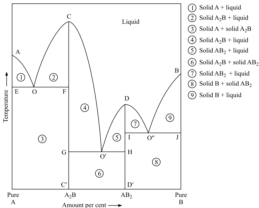
Fig. 6.6.2 Formation of two congruent compounds
