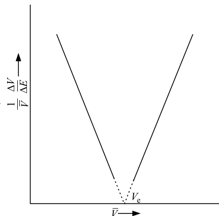
Fig. 8.18.7 A typical graph between (\Delta V/\Delta E)/\bar{V} and \bar{V} (Gran's method)
