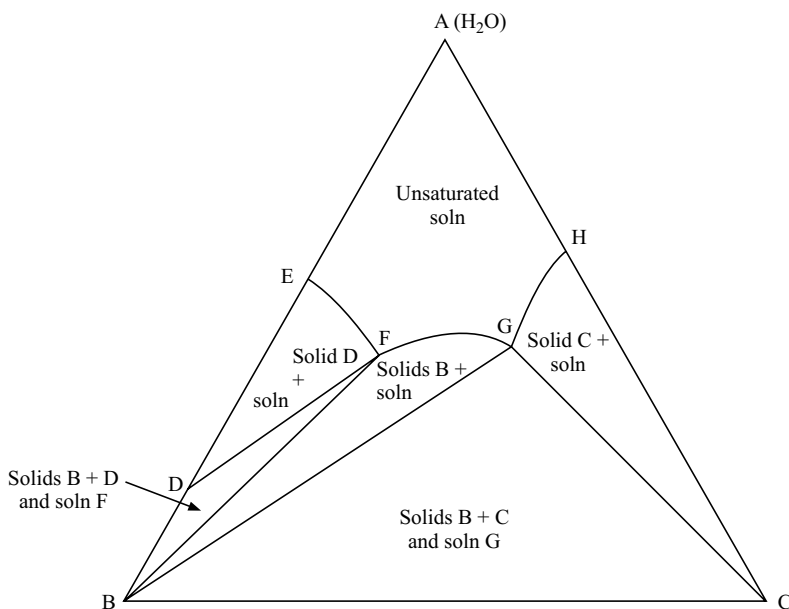
Fig. 7.7.3 Triangular plot where both stable hydrate and the anhydrous salt crystallize together
