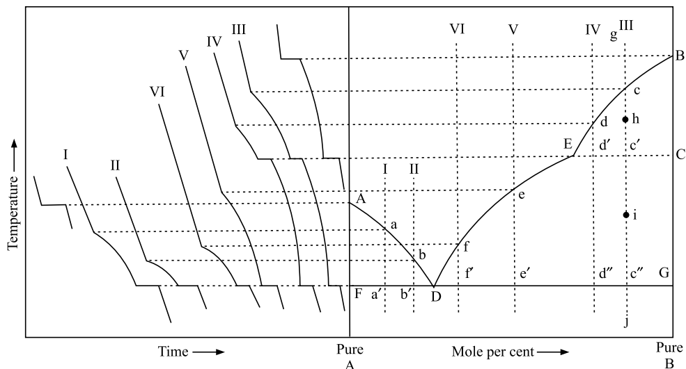
Fig. 6.5.1 Simple eutectic phase diagram for a system exhibiting crystalline modification of one of the components
