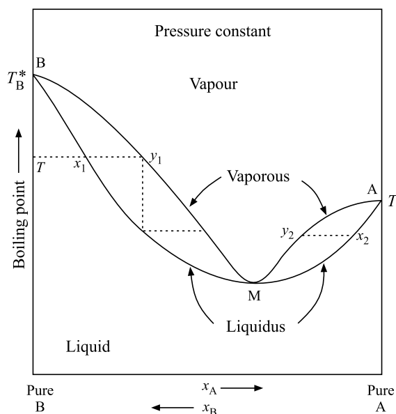
Fig. 4.16.1 Temperature-composition diagram for a system exhibiting a minimum in boiling point
