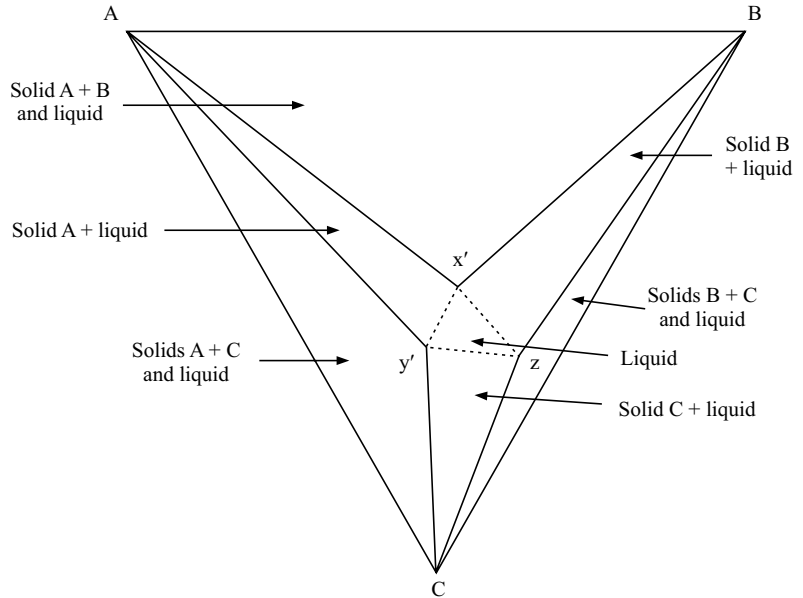
Fig. 7.4.8 Triangular plot at temperature T_7 which lies below the eutectic temperatures of A–B, A–C and B–C systems
