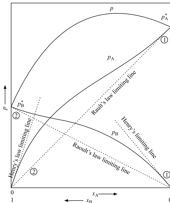
Fig. 4.14.1 Pressure-composition curves of a typical nonideal solution exhibiting positive deviation from ideality
