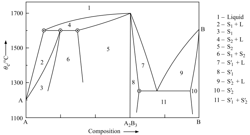
Fig. 6.10.3 Required phase diagram
