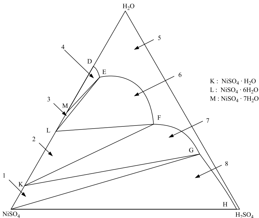
Fig. 7.8.2 The required phase diagram:
