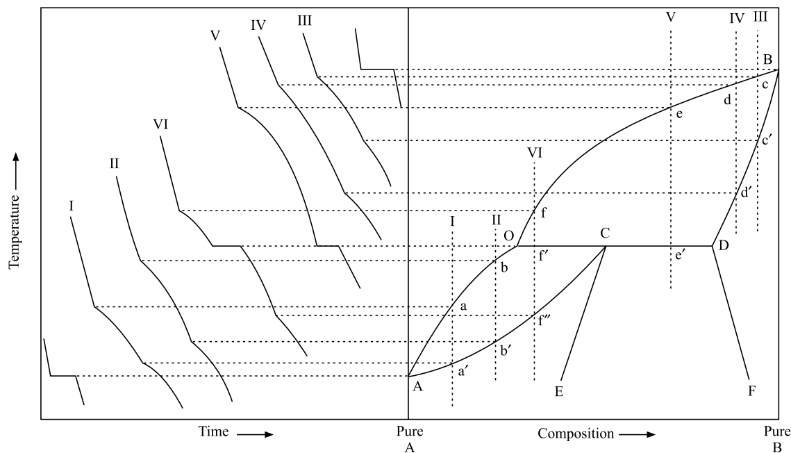
Fig. 6.10.1 Phase diagram exhibiting partial miscibility in the solid state with a peritectic transition
