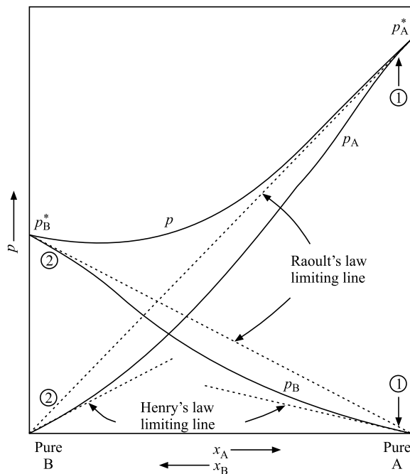
Fig. 4.14.2 Pressure-composition diagram of a typical system exhibiting negative deviation
