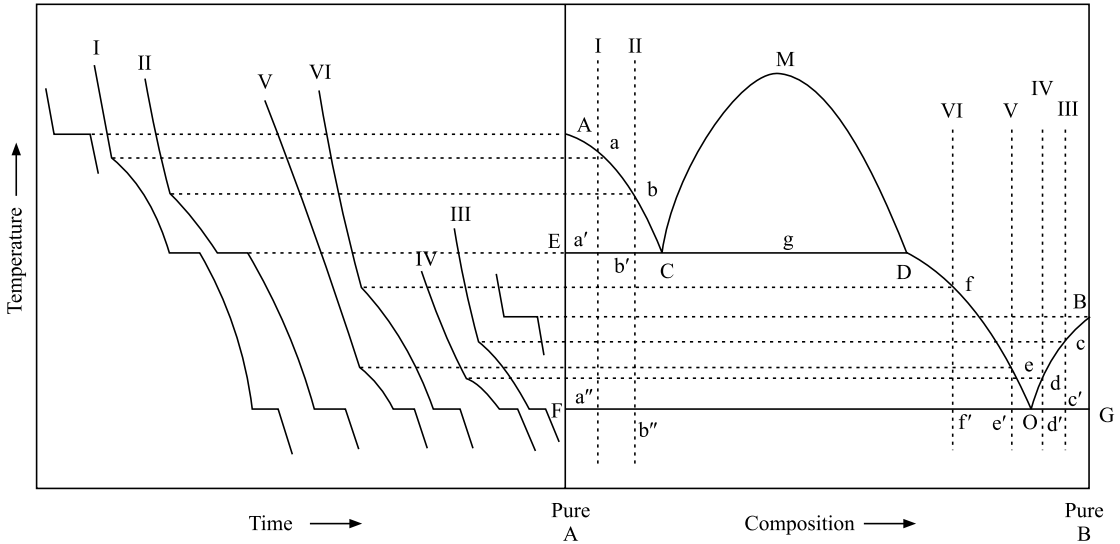
Fig. 6.11.1 Phase diagram exhibiting partial miscibility in the liquid phase
