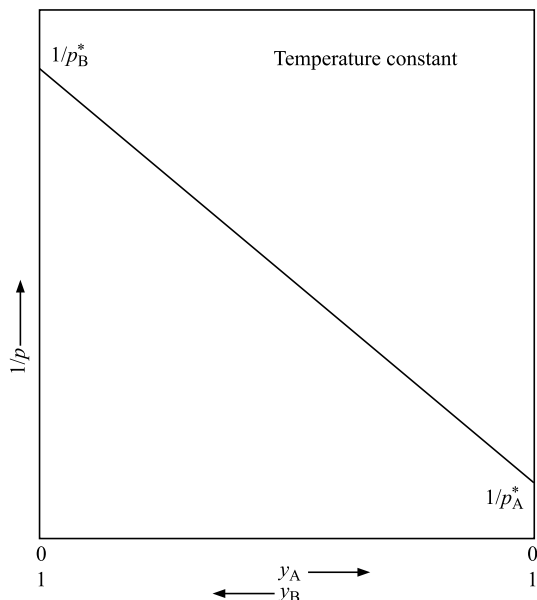
Fig. 4.9.3 Plot of 1/p versus y_A , the composition of A in vapour phase
