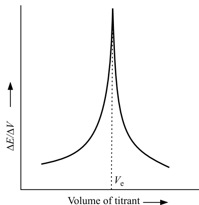
Fig. 8.18.5 A typical first derivative graph
