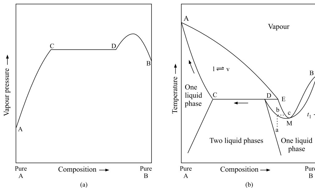
Fig. 4.18.9 (a) Vapour pressure-composition and (b) temperature-composition diagrams for partial miscible liquids exhibiting azeotropic mixture
