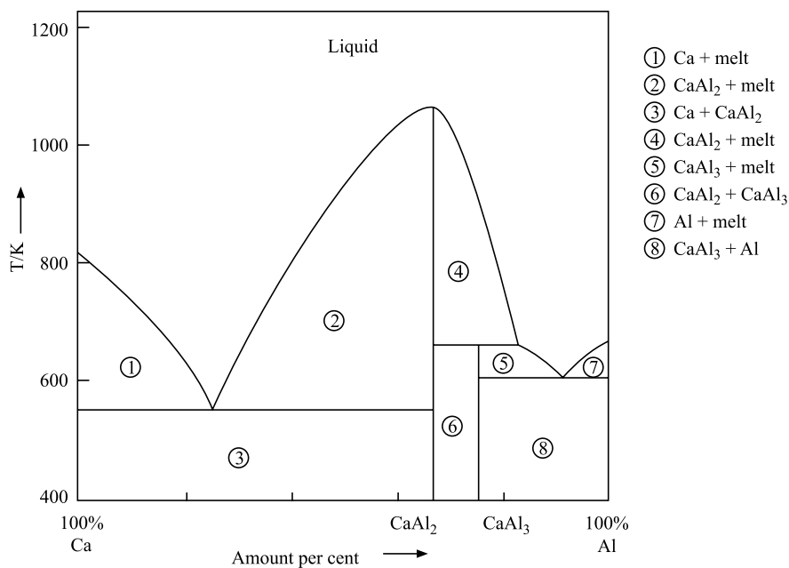
Fig. 6.7.5 Phase diagram of Ca-Al system
