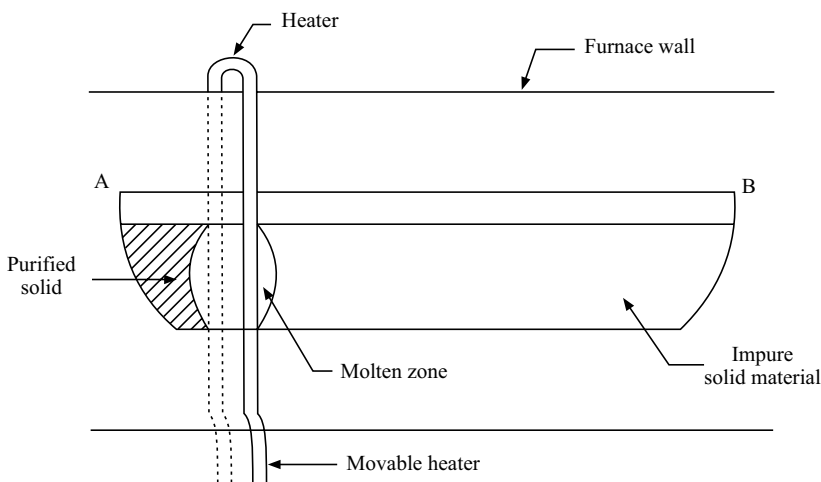
Fig. 6.8.2 Schematic representation of a zone refining apparatus
