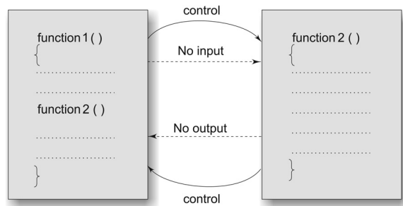
Fig. 5.3 No data communication between functions
