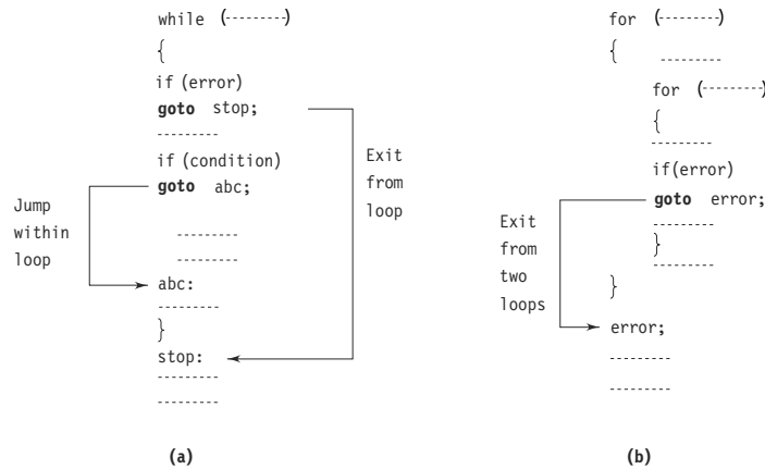
Fig. 4.17 Jumping within and exiting from the loops with goto statement
