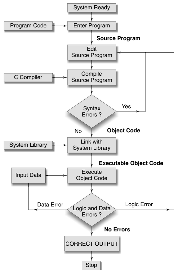
Fig. 1.64 Process of compiling and running a C program
