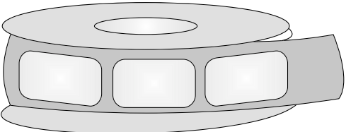
Fig. 1.14 Magnetic tape
