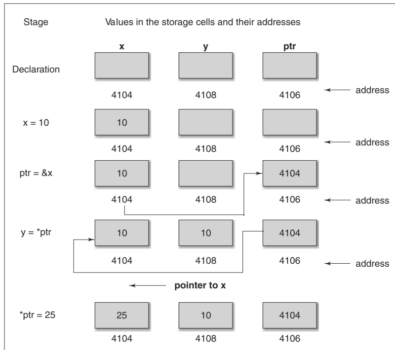
Fig. 6.6 Illustration of pointer assignments
