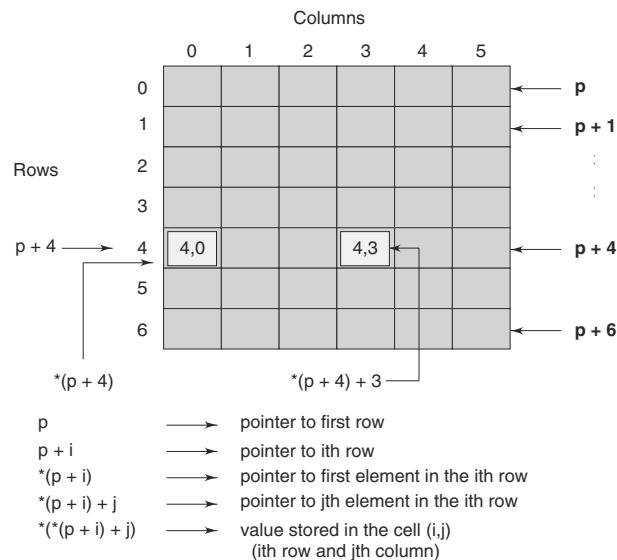
Fig. 6.9 Pointers to two-dimensional arrays
