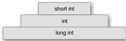
Fig. 1.70 Integer types
