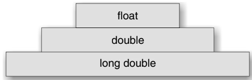
Fig. 1.71 Floating-point types
