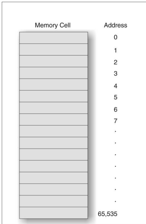
Fig. 6.1 Memory organisation
