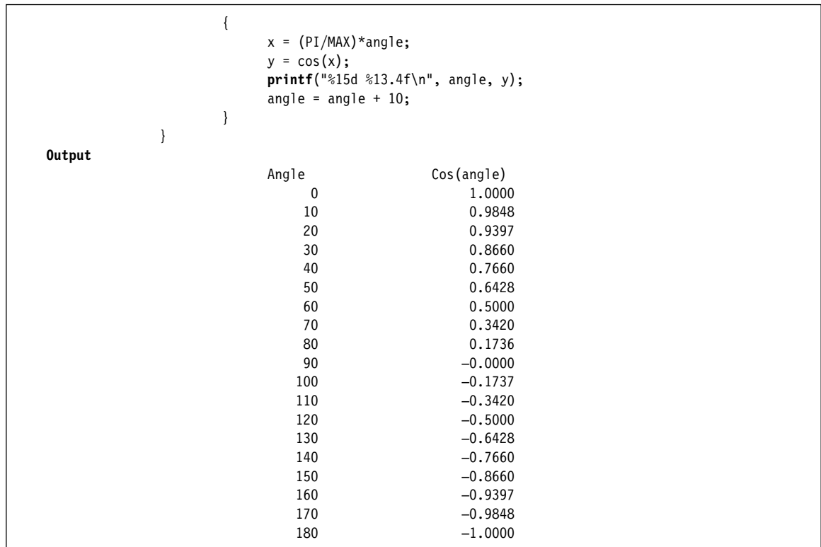
Fig. 1.62 Program using a math function
