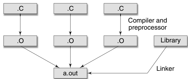
Fig. 1.65 Compilation of multiple files
