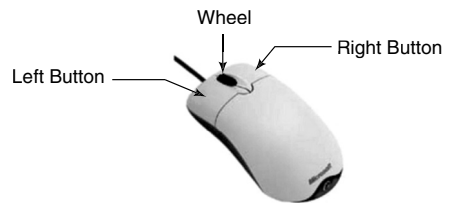
Fig. 1.5 Mouse
