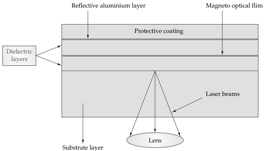
Fig. 1.17 Magneto-optical disk
