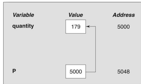
Fig. 6.3 Pointer variable
