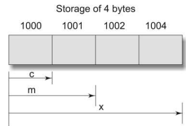
Fig. 7.7 Sharing of a storage locating by union members
