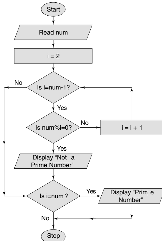
Fig. 1.39 Flowchart to find out whether a given number is prime or not
