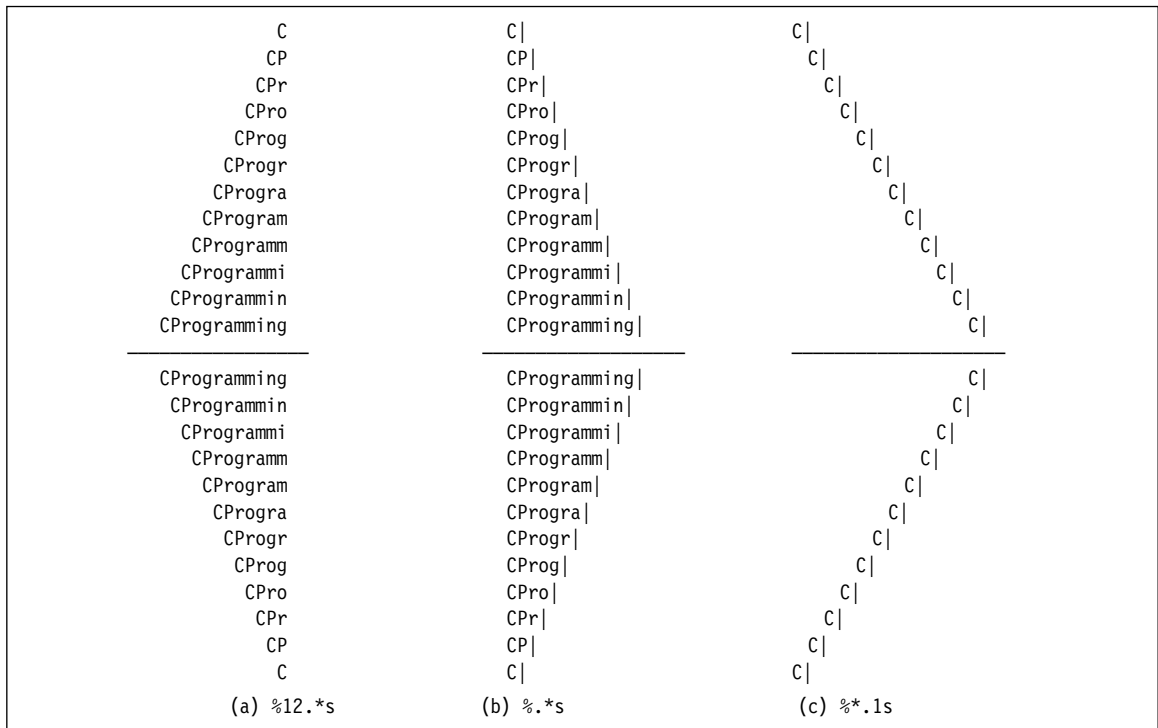
Fig. 4.6 Further illustrations of variable specifications
