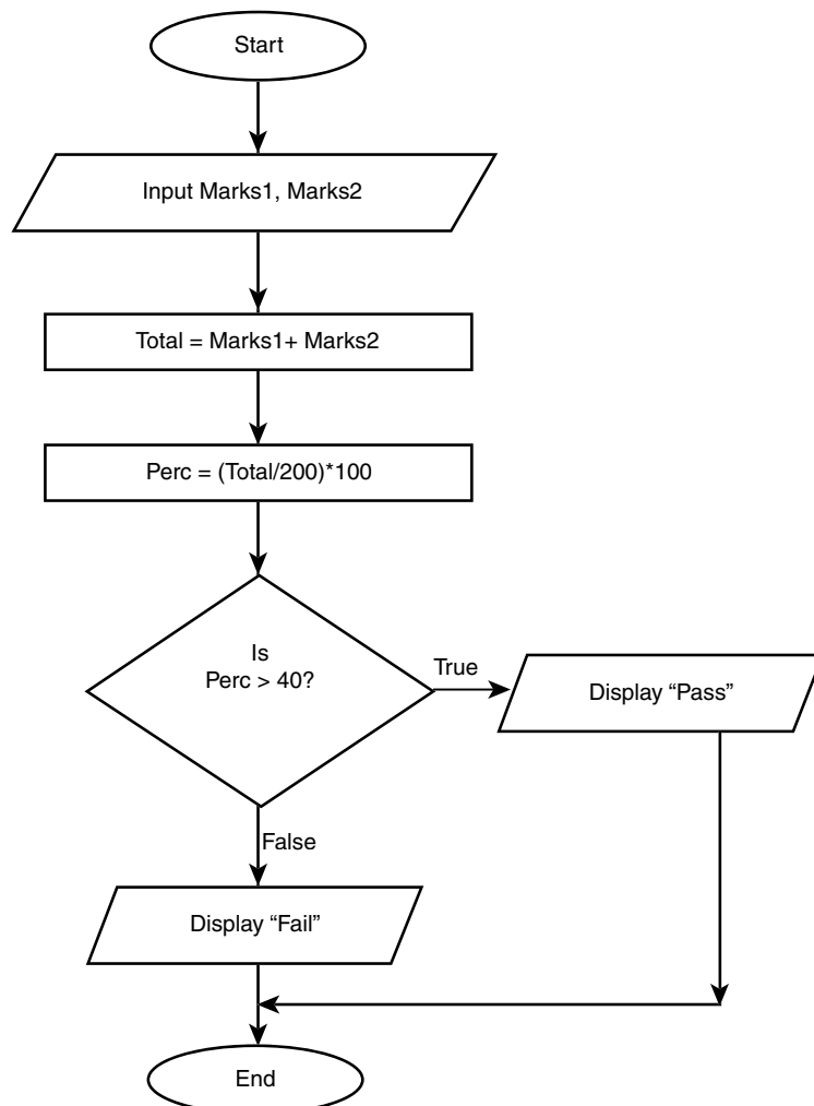
Fig. 1.21. Flowchart for calculating the percentage of marks and displaying the result.
