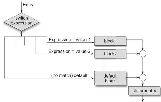
Fig. 2.11 Selection process of the switch statement
