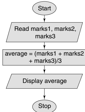
Fig. 1.40 Flowchart to find the average of marks obtained by a student
