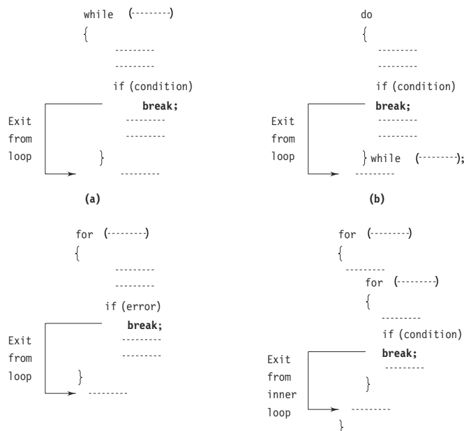
Fig. 4.16 Exiting a loop with break statement
