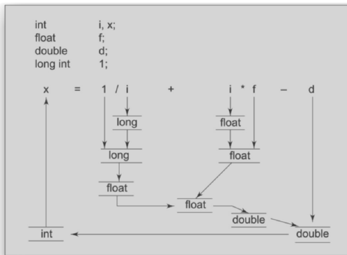
Fig. 1.93 Process of implicit type conversion
