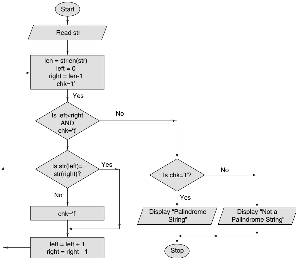
Fig. 1.43 Flowchart to determine whether a given string is a palindrome or not
