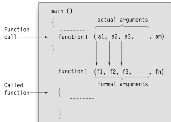
Fig. 5.6 Arguments matching between the function call and the called function
