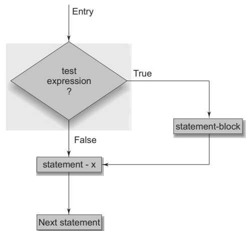
Fig. 2.2 Flow chart of simple if control
