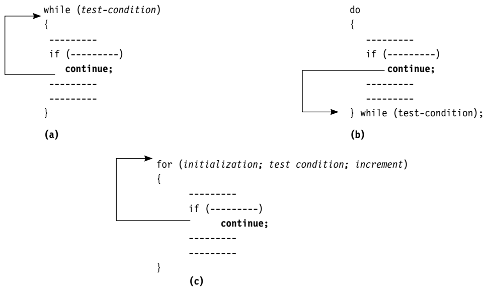
Fig. 4.20 Bypassing and continuing in loops
