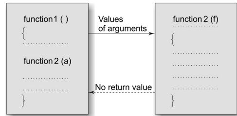
Fig. 5.5 One-way data communication
