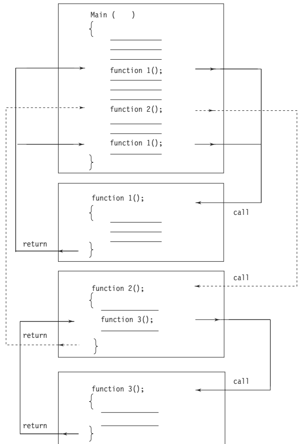
Fig. 5.2 Flow of control in a multi-function program
