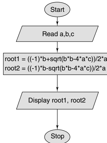
Fig. 1.51 Flowchart for finding the roots of a quadratic equation
