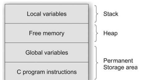
Fig. 6.14 Storage of a C program
