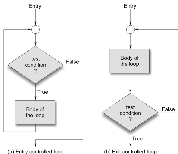
Fig. 4.11 Loop control structures
