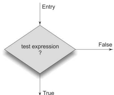
Fig. 2.1 Two-way branching
