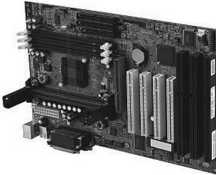
Fig. 1.7 A motherboard
