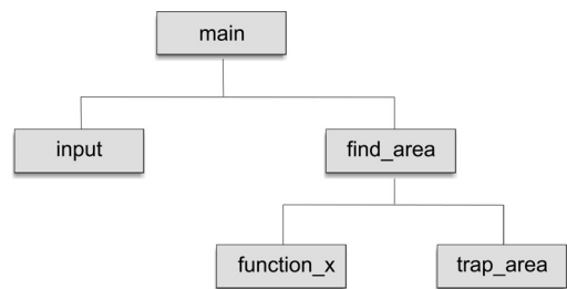
Fig. 5.20 Modular chart
