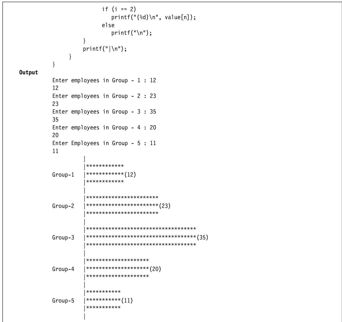
Fig. 4.26 Program to draw a histogram
