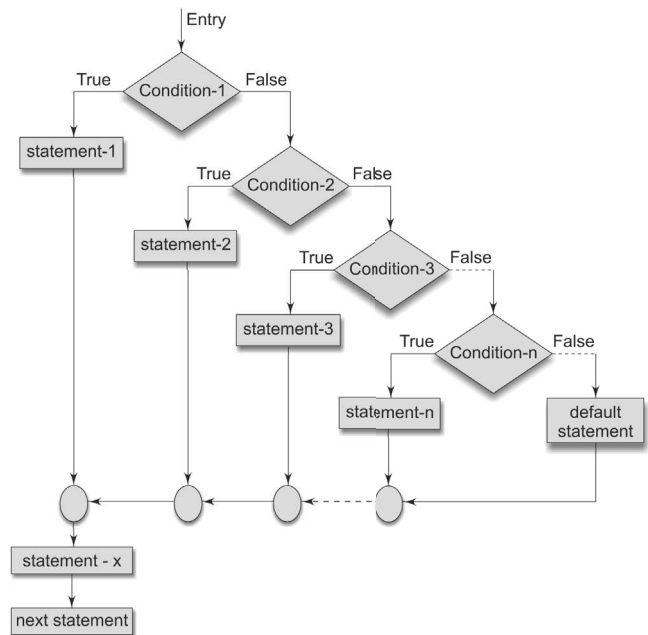
Fig. 2.9 Flow chart of else..if ladder
