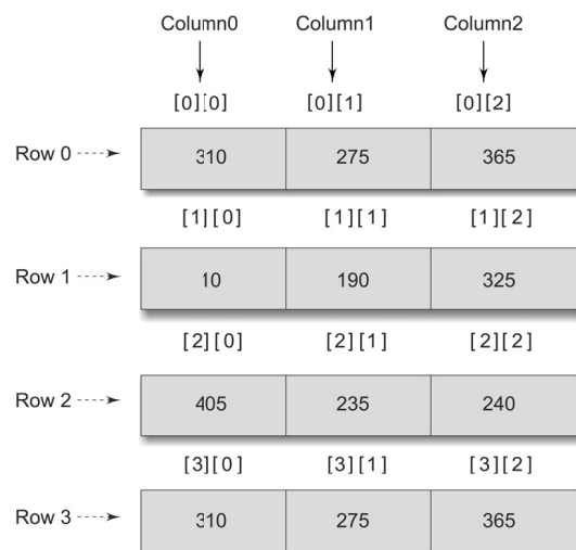
Fig. 3.7 Representation of a two-dimensional array in memory
