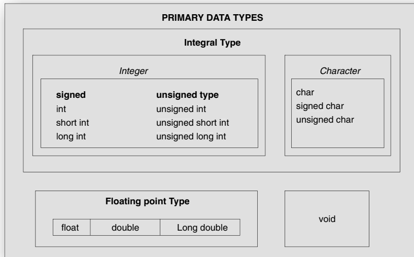
Fig. 1.69 Primary data types in C
