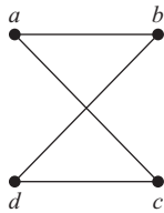
FIGURE 4 A Graph with the Given Adjacency Matrix.
