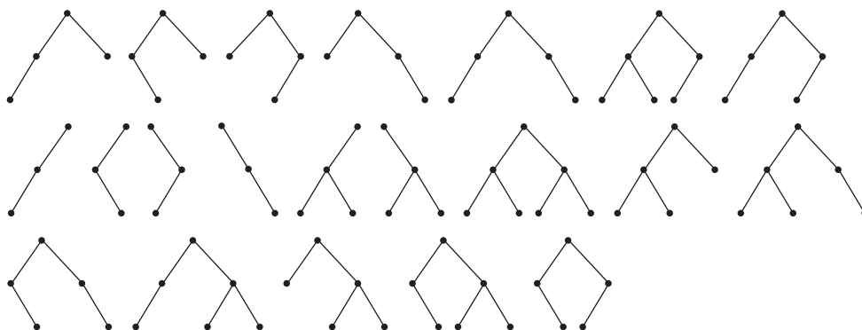
FIGURE 3 Building Up Extended Binary Trees.
