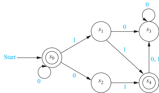
FIGURE 7 A Nondeterministic Finite-State Automaton.
