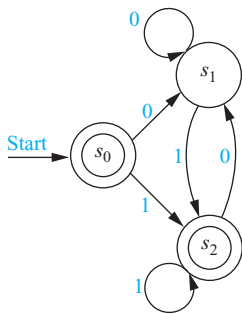
FIGURE 5 A Finite-State Automaton.
