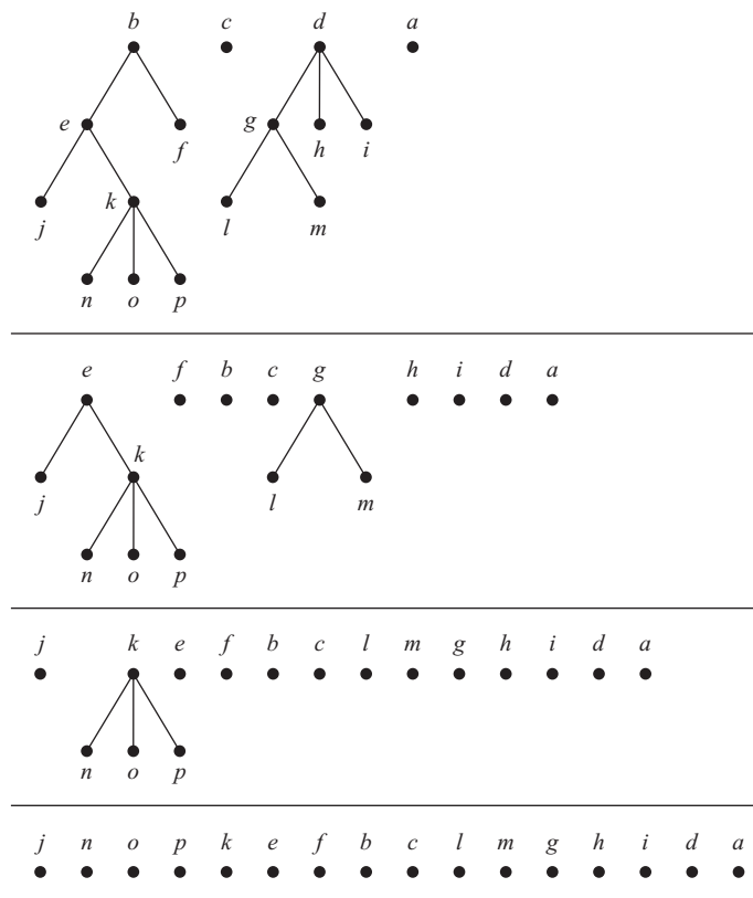
FIGURE 8 The Postorder Traversal of T .
