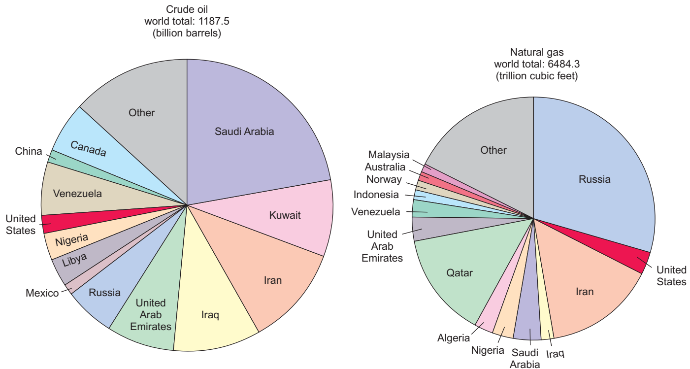
Figure 14.5 Estimated proven world reserves of crude oil and natural gas, January 2006. Note that inclusion of the fuel in Canada's tar sands (discussed later in the chapter) would increase world oil reserves by more than 150 billion barrels, and make Canada's oil reserves second only to those of Saudi Arabia. Source: Averages of estimates of BP Statistical Review, Oil and Gas Journal and World Oil, as summarized in International Energy Annual 2006, U.S. Energy Information Administration.
