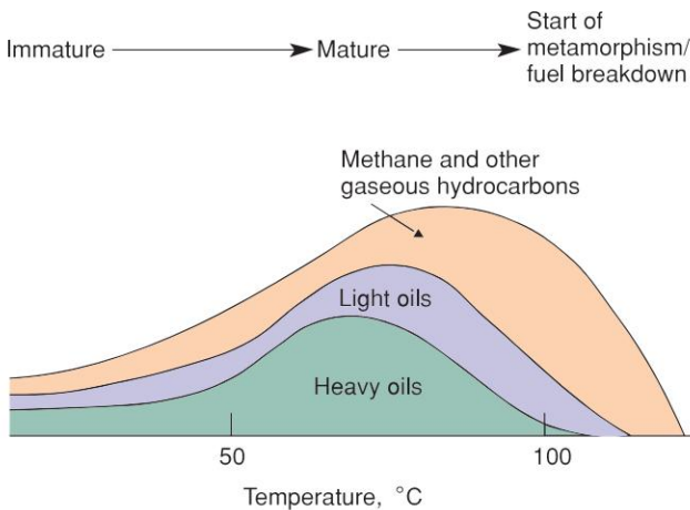
Figure 14.3 The process of petroleum maturation in a marine deposit, in simplified form. Source: After J. Watson, Geology and Man, 1983, Allen and Unwin, Inc.
