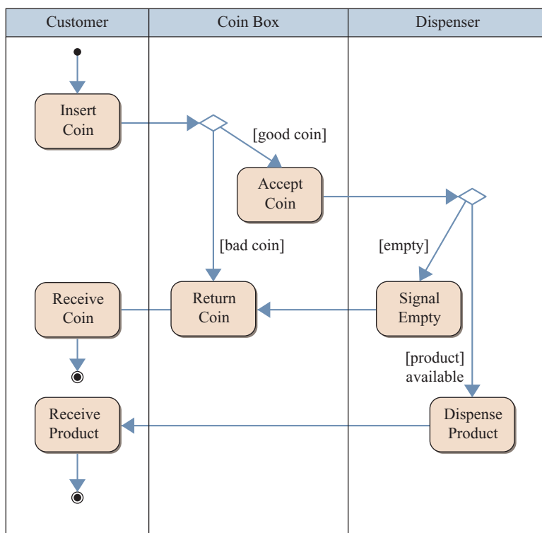
Figure 7 Activity diagram.
