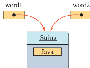
Figure 5.6 Difference between using and not using the new operator for String .
