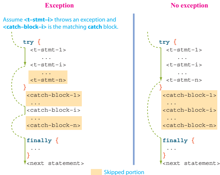
Figure 8.3 Two possible control flows of the try-catch statement with multiple catch blocks and the finally block. The finally block is always executed.
