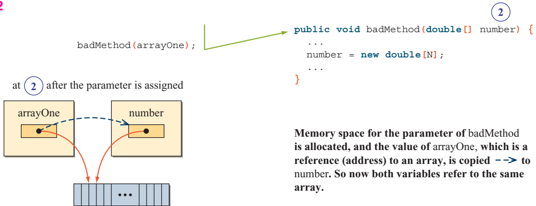
Figure 10.11 Effect of creating a local array and not returning it.
