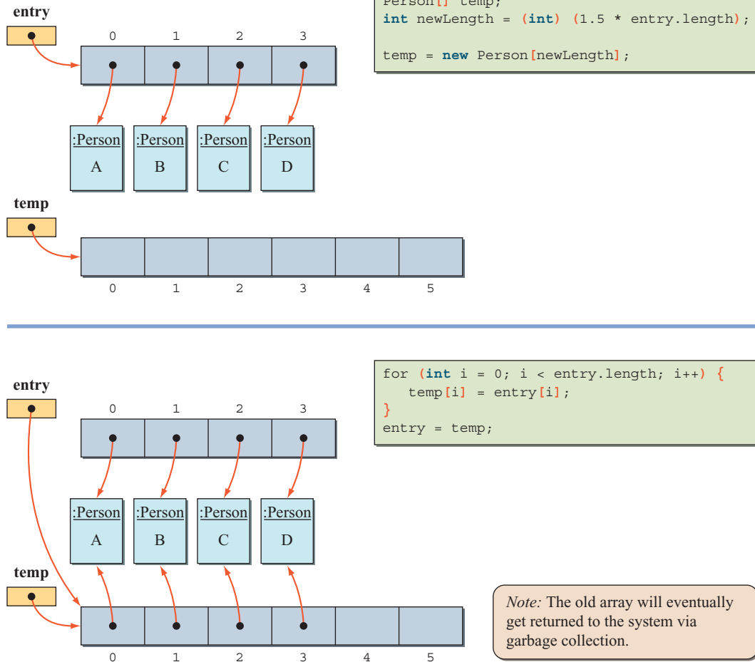
Figure 10.16 How a new array that is 150 percent of the original array is created. The size of the original array is 4.
