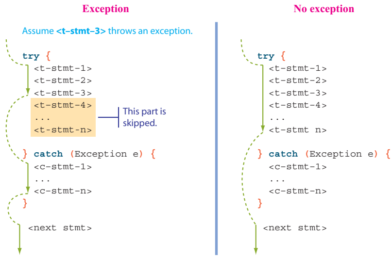
Figure 8.1 Two possible control flows of the try-catch statement with one catch block. Assume <t-stmt-3> throws an exception.
