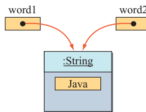
Figure 9.3 Difference between using and not using the new operator for String .
