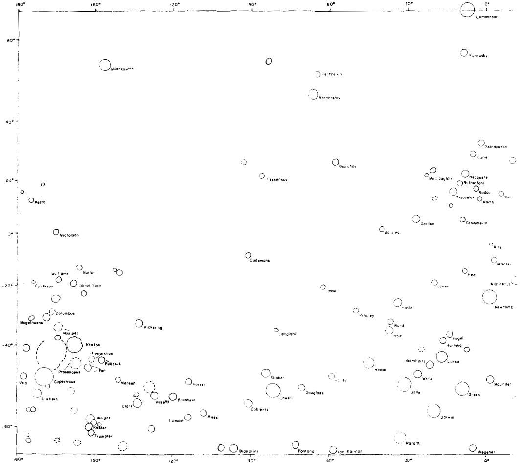
FIG. 3a. Named craters at equatorial and middle latitudes; IAU Commission 16—working group
