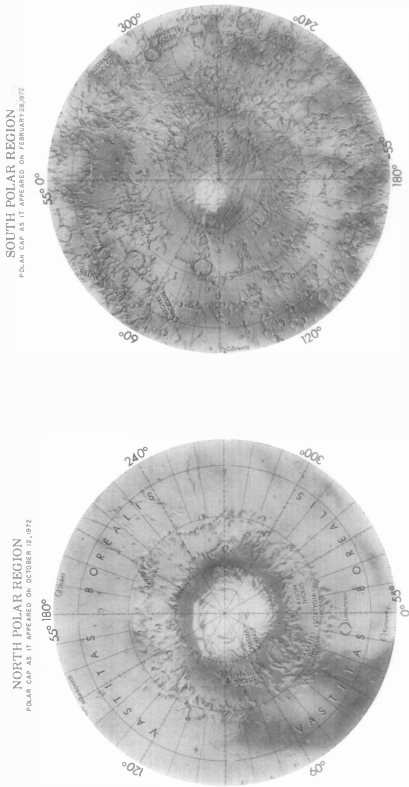
FIG. 4b. Same but "polar latitudes."
