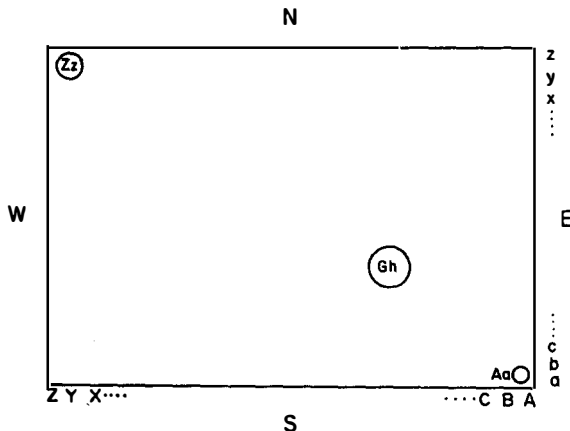
FIG. 2. Double letter crater designation scheme within each 1:5 000 000 map quadrangle.
