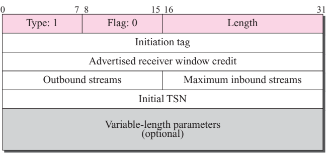
Figure 16.10 INIT chunk
