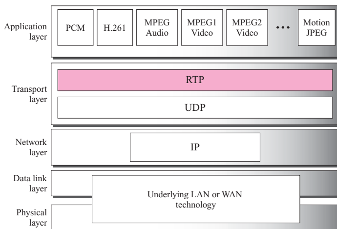
Figure 25.18 RTP
