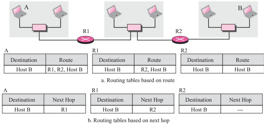
Figure 6.3 Next-hop method
