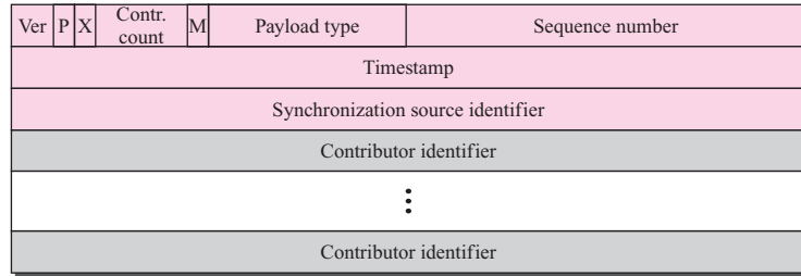
Figure 25.19 RTP packet header format
