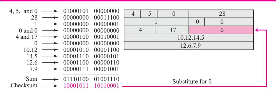
Figure 7.24 Example of checksum calculation at the sender
