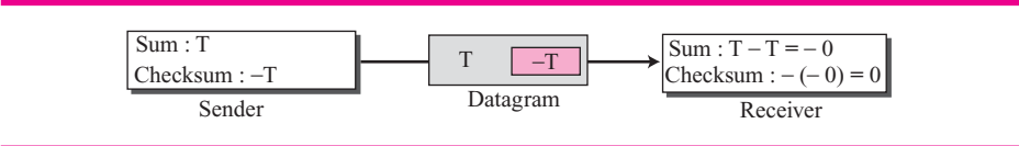
Figure 7.23 Checksum in one's complement arithmetic
