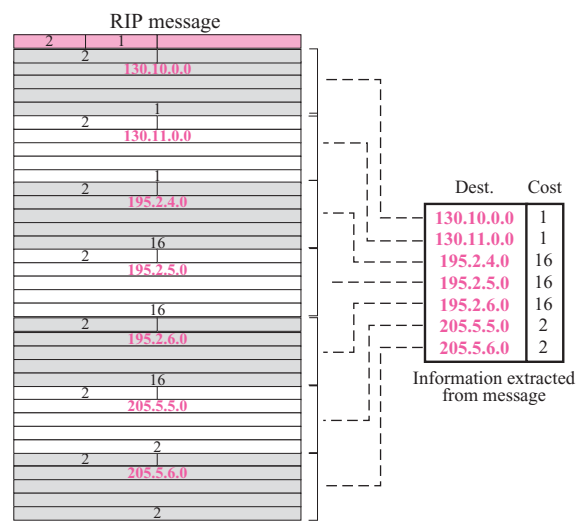
Figure 11.13 Solution to Example 11.4
