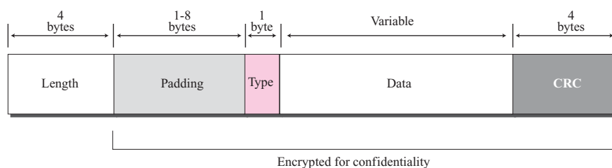
Figure 20.19 SSH Packet Format
