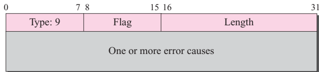
Figure 16.17 ERROR chunk
