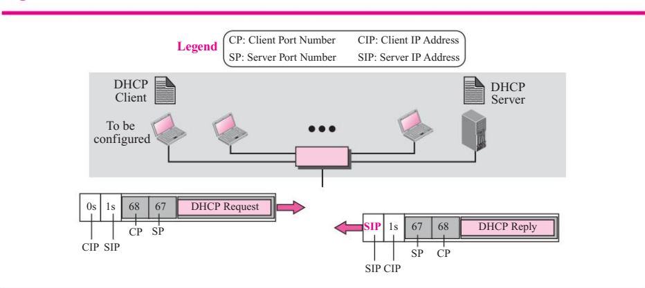
Figure 18.1 Client and server on the same network
