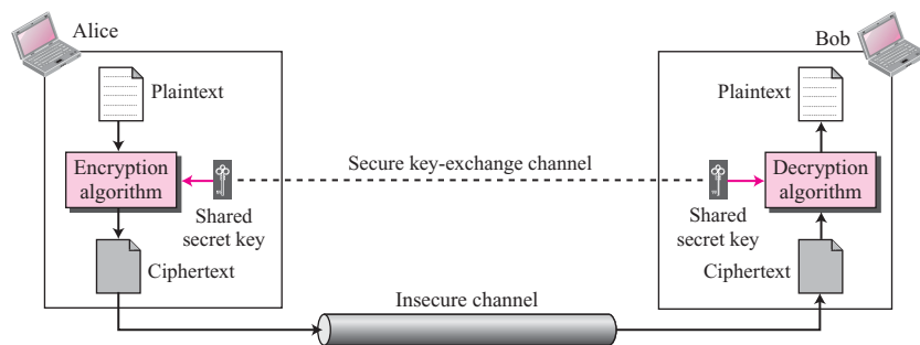
Figure 29.2 General idea of a traditional cipher
