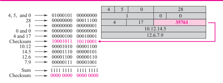
Figure 7.25 Example of checksum calculation at the receiver
