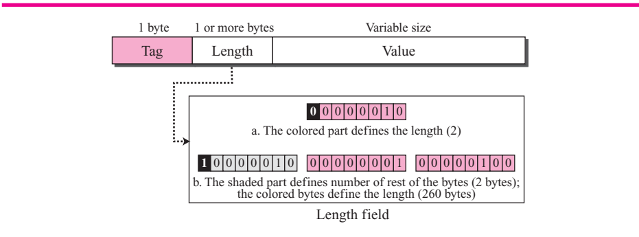
Figure 24.7 Encoding format
