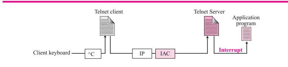
Figure 20.12 Example of interrupting an application program
