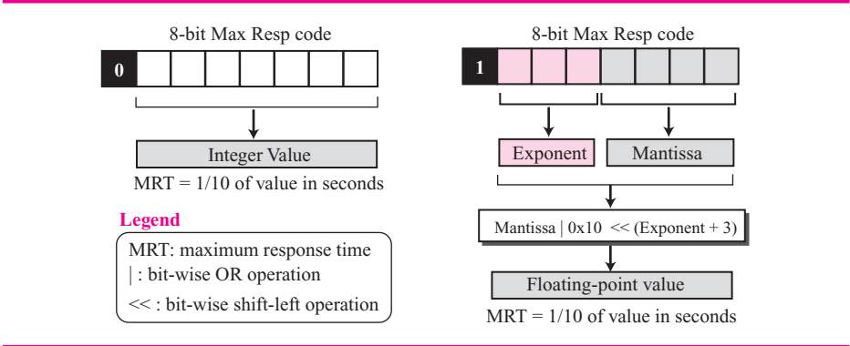
Figure 12.17 Calculation of maximum response time
