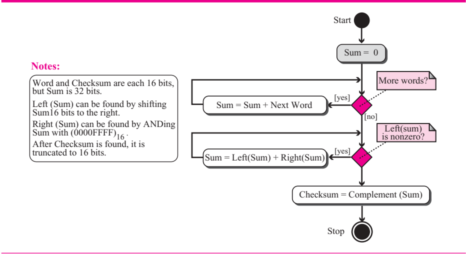
Figure D.2 Algorithm to calculate traditional checksum
