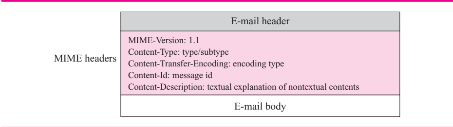
Figure 23.16 MIME header
