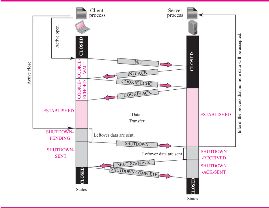
Figure 16.24 A common scenario of states
