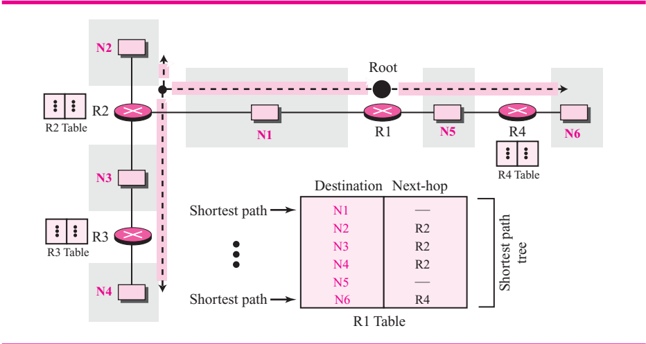
Figure 12.18 Shortest path tree in unicast routing
