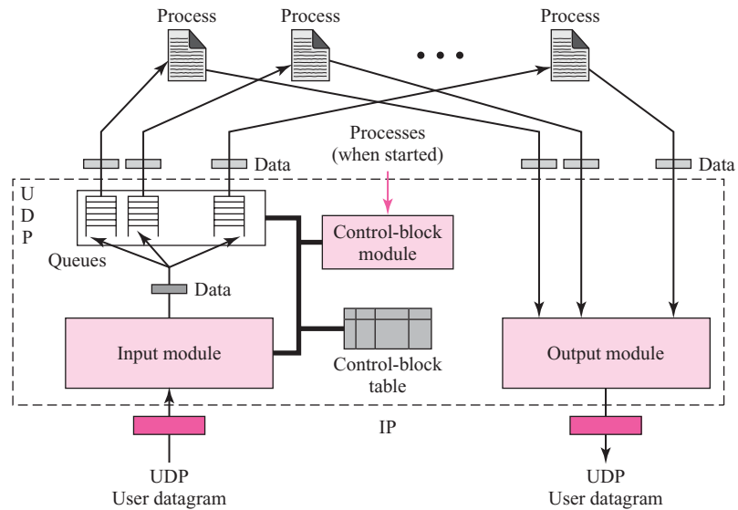
Figure 14.8 UDP design
