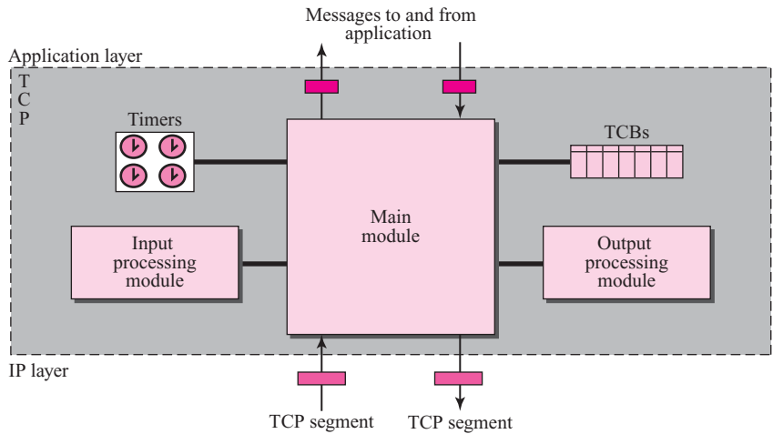
Figure 15.52 TCP package
