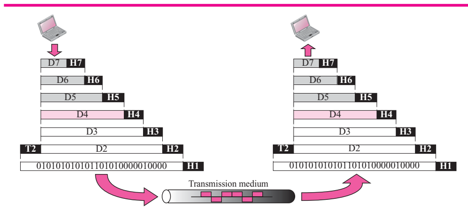
Figure 2.5 An exchange using the OSI model
