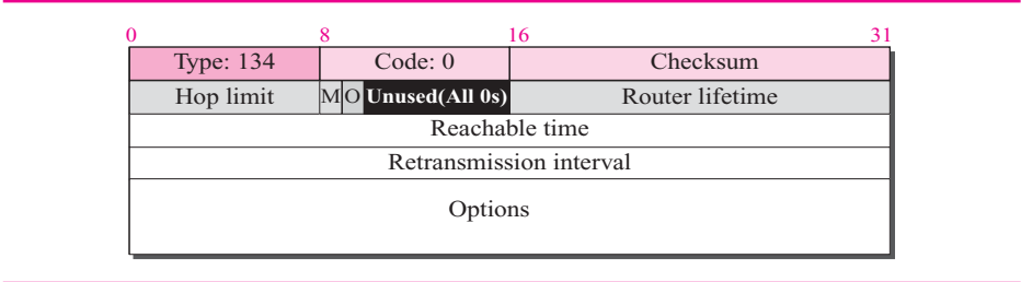
Figure 28.11 Router-advertisement message
