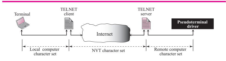
Figure 20.3 Concept of NVT
