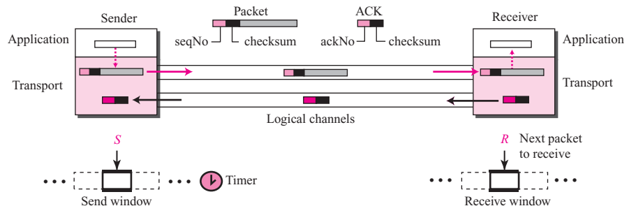
Figure 13.19 Stop-and-Wait protocol
