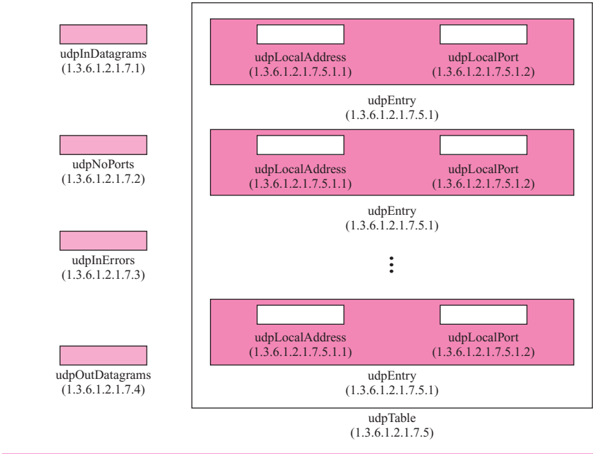
Figure 24.14 udp variables and tables
