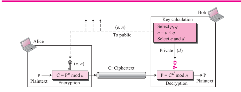
Figure 29.15 Encryption, decryption, and key generation in RSA
