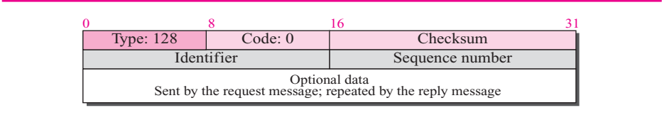
Figure 28.8 Echo-request message
