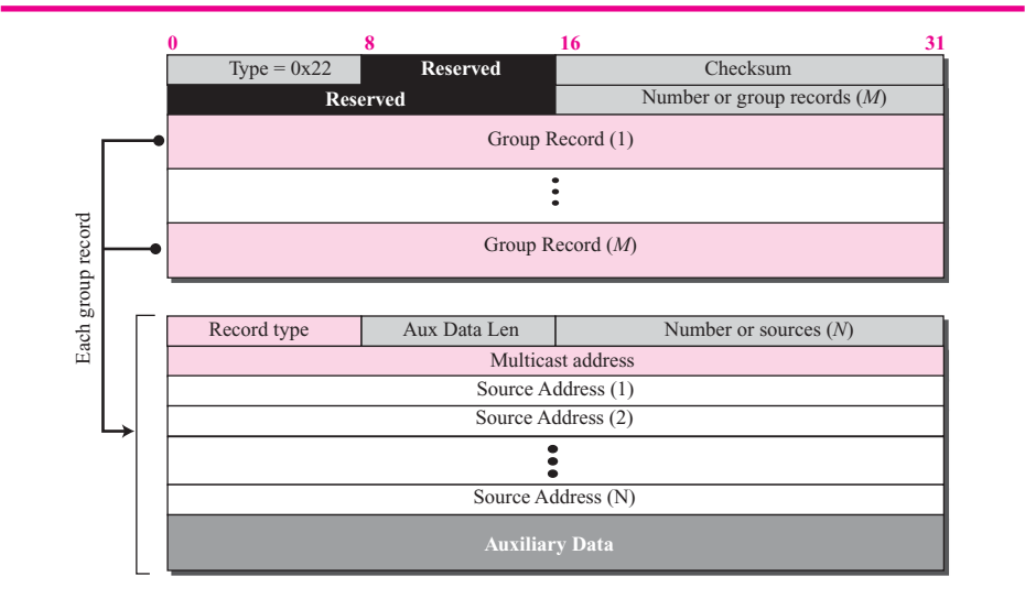
Figure 12.10 Membership report message format
