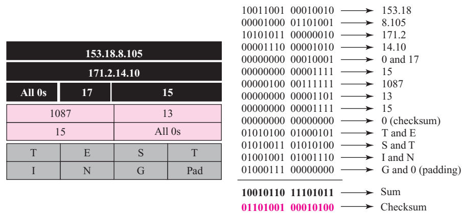
Figure 14.4 Checksum calculation of a simple UDP user datagram
