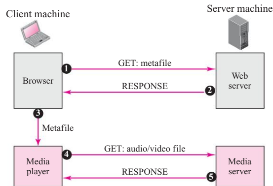
Figure 25.12 Using a media server
