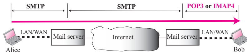
Figure 23.13 POP3 and IMAP4
