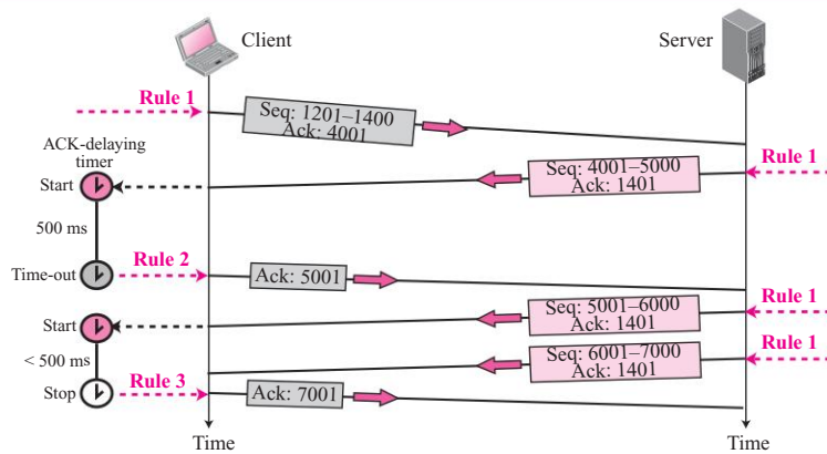
Figure 15.29 Normal operation
