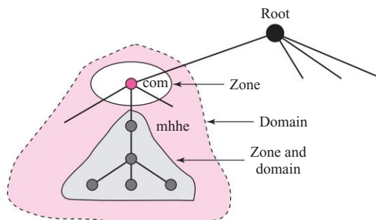
Figure 19.7 Zones and domains
