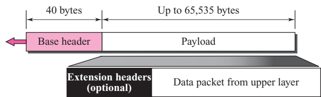
Figure 27.1 IPv6 datagram
