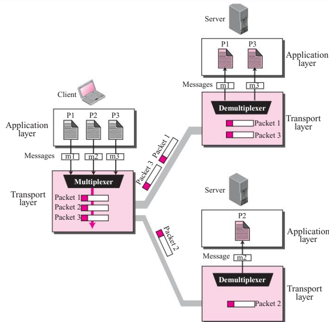
Figure 13.7 Multiplexing and demultiplexing
