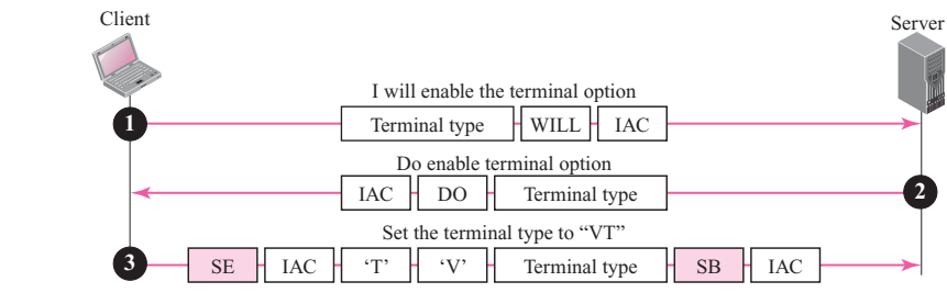
Figure 20.11 Example of sub-option negotiation
