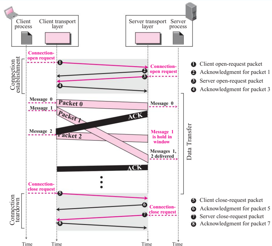
Figure 13.14 Connection-oriented service
