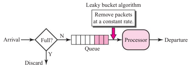
Figure 25.33 Leaky bucket implementation
