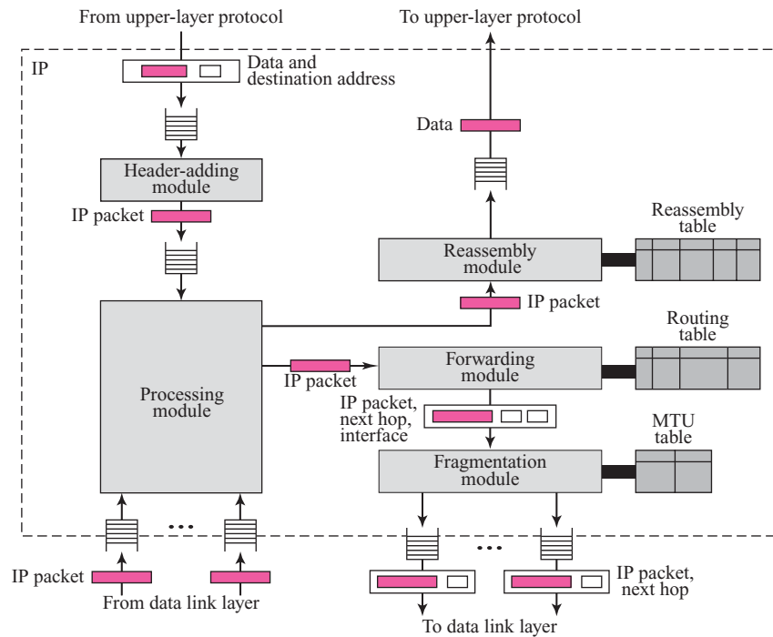
Figure 7.29 IP components
