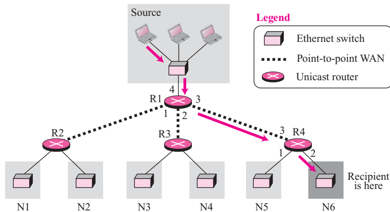
Figure 12.1 Unicasting
