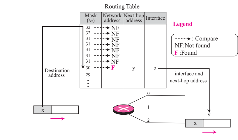
Figure 6.18 Example 6.13: Forwarding based on destination address
