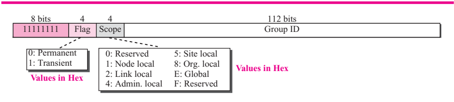
Figure 26.13 Multicast address
