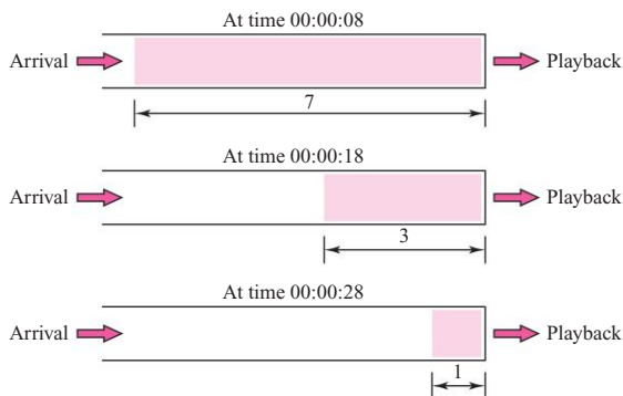
Figure 25.17 Playback buffer
