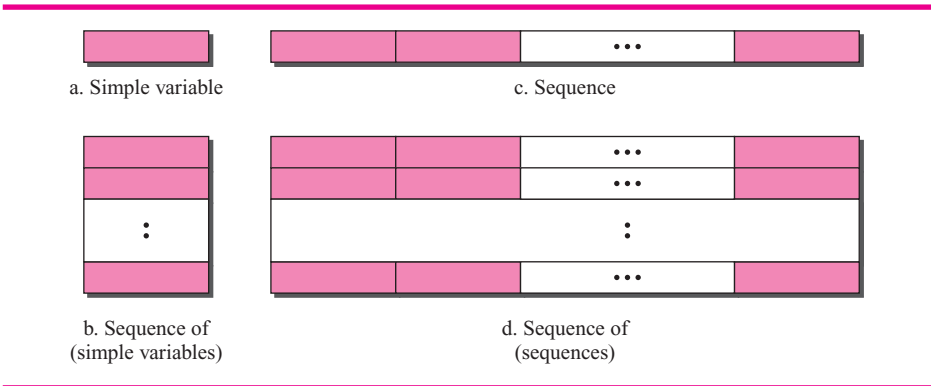
Figure 24.6 Conceptual data types
