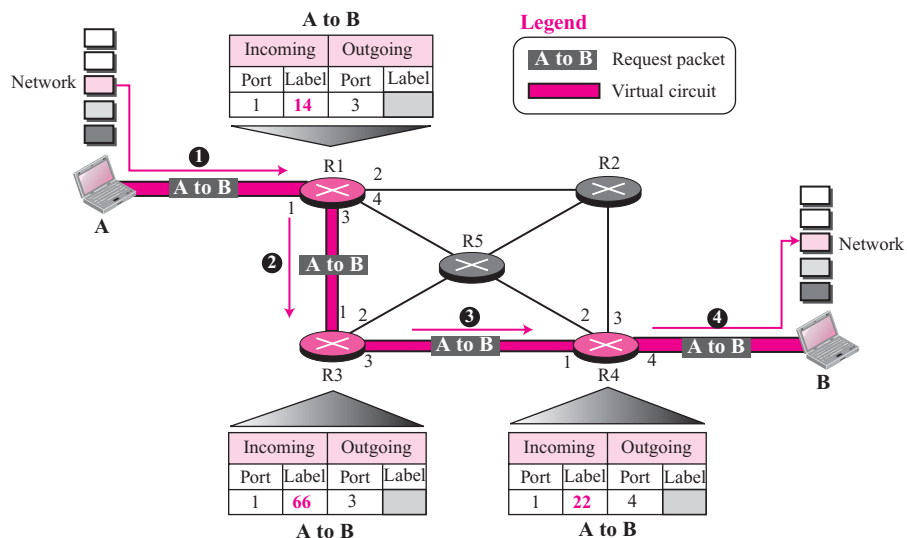
Figure 4.8 Sending request packet in a virtual-circuit network
