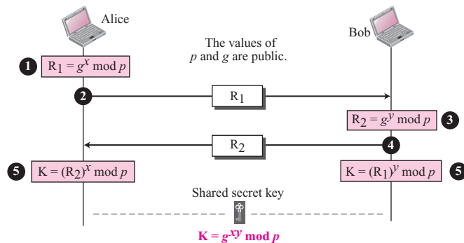
Figure 29.27 Diffie-Hellman method
