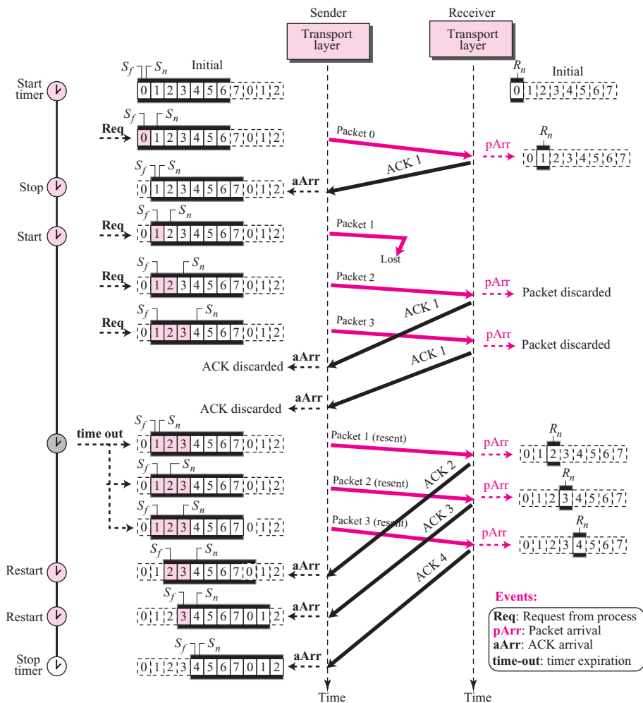
Figure 13.29 Flow diagram for Example 3.8
