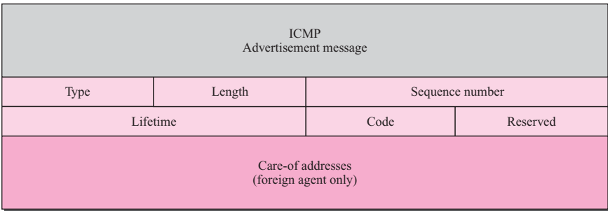
Figure 10.4 Agent advertisement
