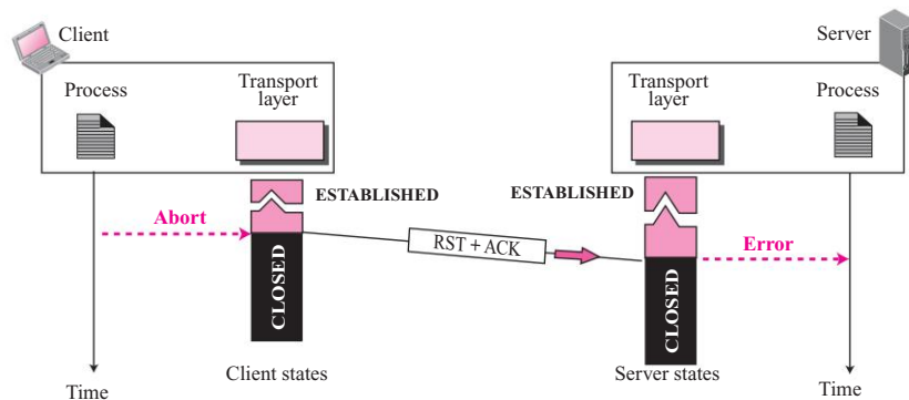
Figure 15.21 Aborting a connection
