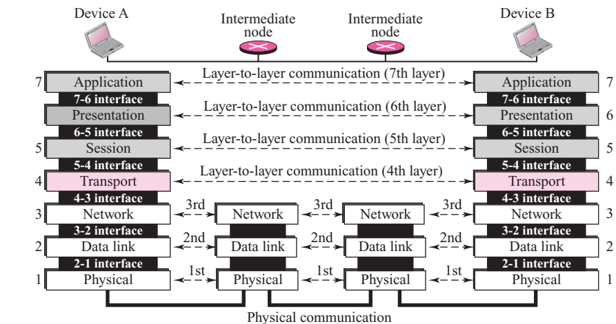
Figure 2.4 OSI layers
