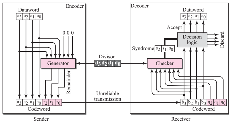
Figure C.6 CRC encoder and decoder
