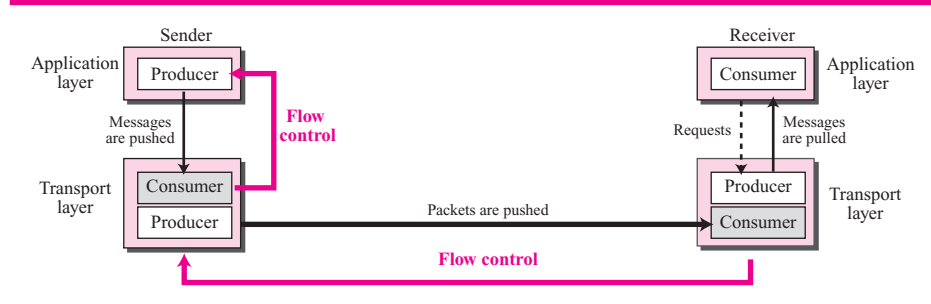
Figure 13.9 Flow control at the transport layer
