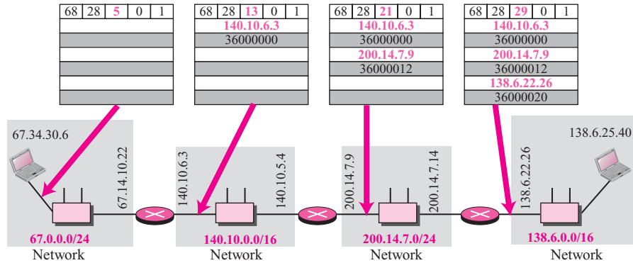
Figure 7.21 Timestamp concept
