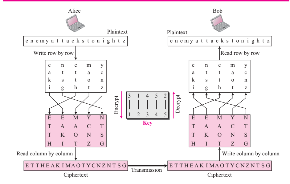
Figure 29.6 Transposition cipher
