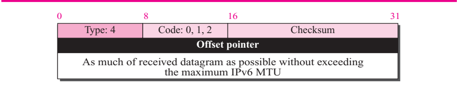
Figure 28.7 Parameter-problem message
