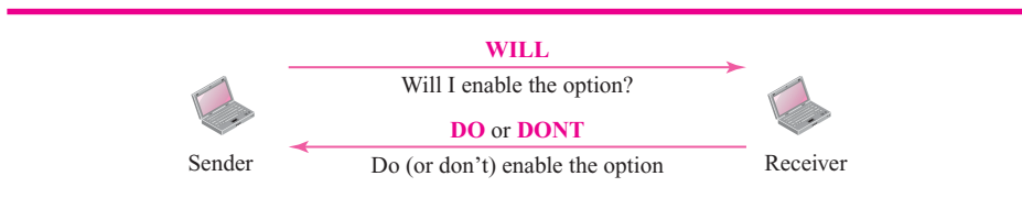
Figure 20.6 Offer to enable an option
