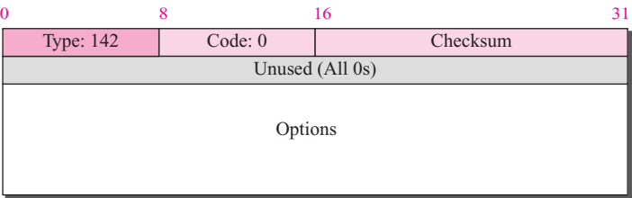
Figure 28.16 Inverse-neighbor-advertisement message
