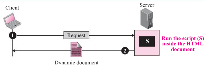
Figure 22.7 Dynamic document using server-site script
