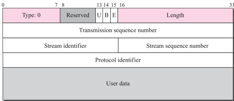
Figure 16.9 DATA chunk
