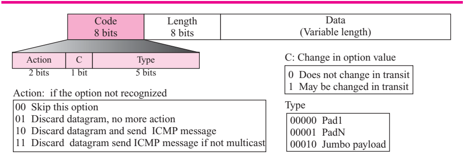
Figure 27.6 The format of options in a hop-by-hop option header
