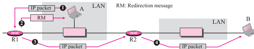
Figure 9.10 Redirection concept
