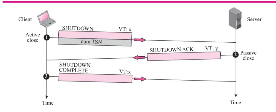
Figure 16.21 Association termination
