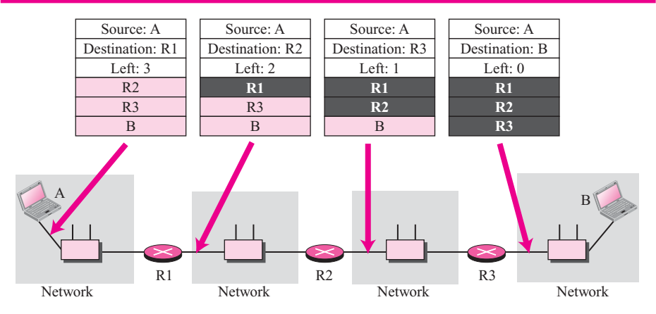
Figure 27.11 Source routing example
