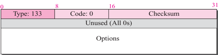
Figure 28.10 Router-solicitation message
