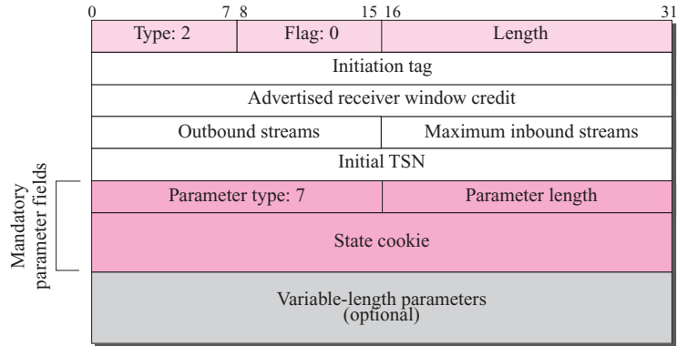
Figure 16.11 INIT ACK chunk
