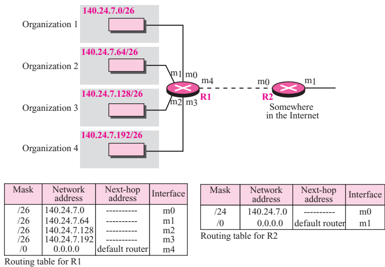
Figure 6.15 Address aggregation
