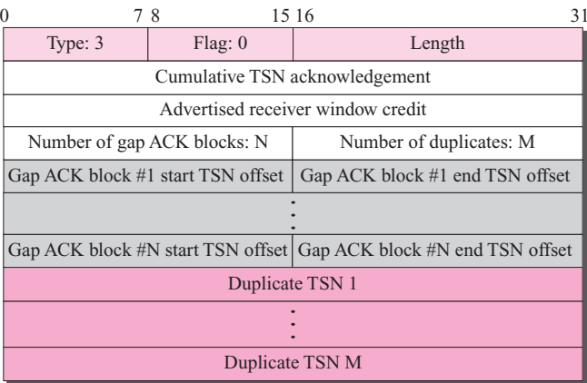
Figure 16.14 SACK chunk
