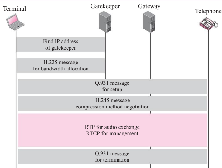
Figure 25.27 H.323 example
