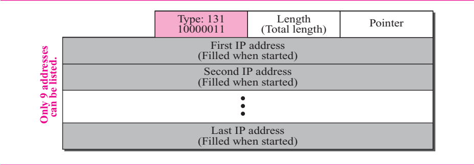
Figure 7.18 Loose-source-route option
