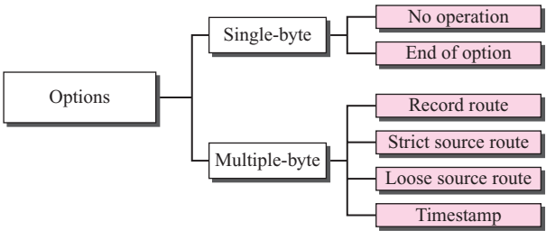
Figure 7.11 Categories of options
