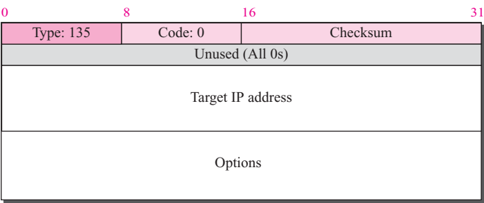
Figure 28.12 Neighbor-solicitation message
