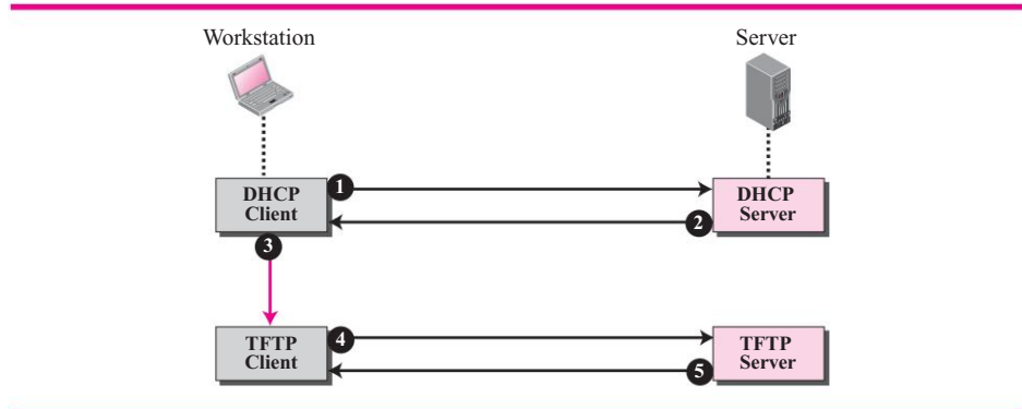
Figure 21.20 Use of TFTP with DHCP
