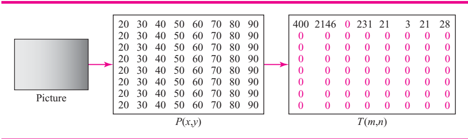
Figure 25.6 Case 3: gradient gray scale
