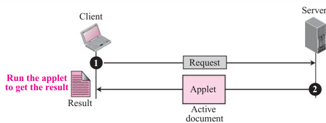
Figure 22.8 Active document using Java applet
