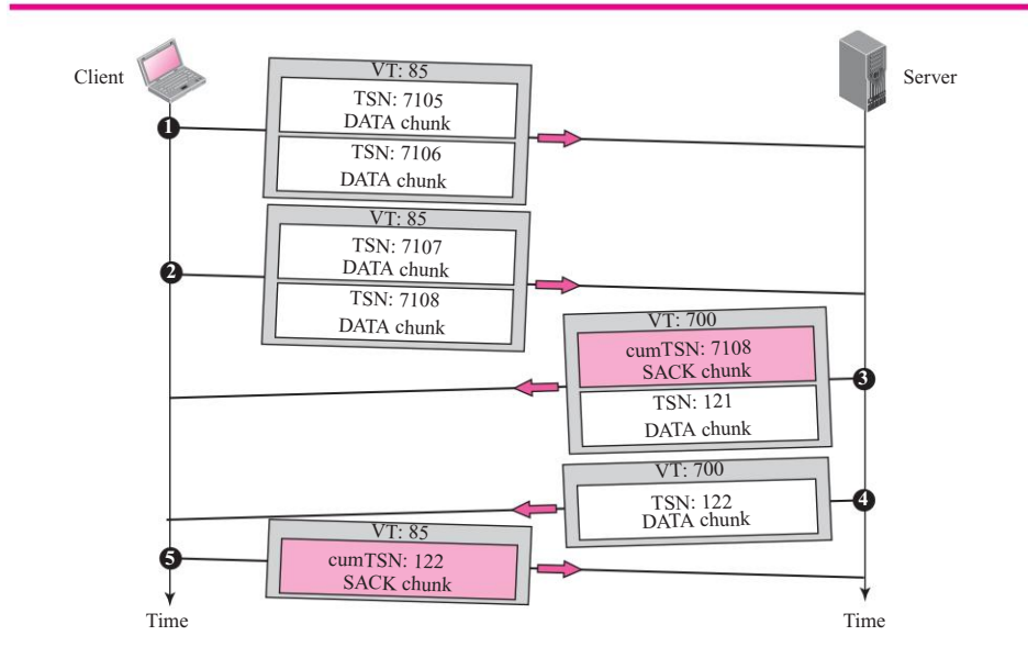
Figure 16.20 Simple data transfer
