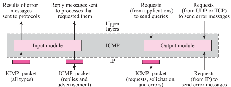
Figure 9.16 ICMP package
