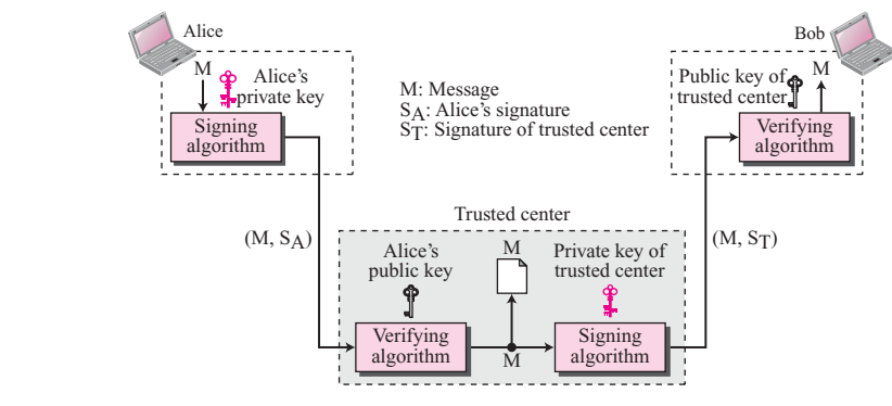
Figure 29.20 Using a trusted center for nonrepudiation
