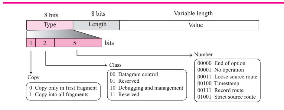
Figure 7.10 Option format
