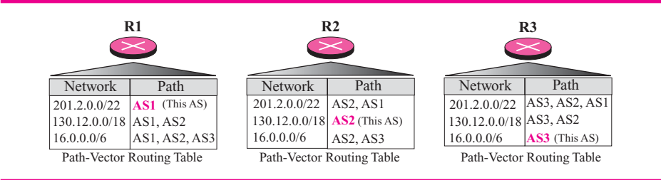
Figure 11.52 Routing table after aggregation
