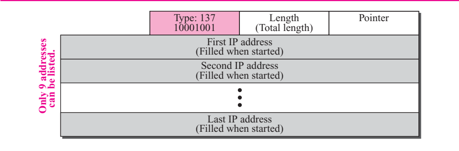
Figure 7.16 Strict-source-route option
