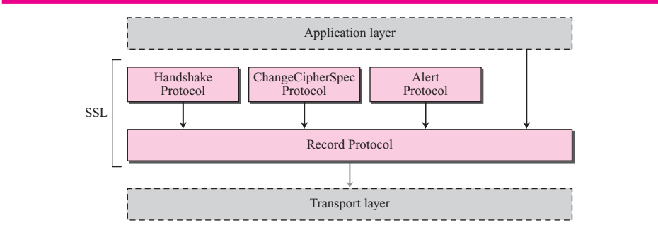
Figure 30.19 Four SSL protocols
