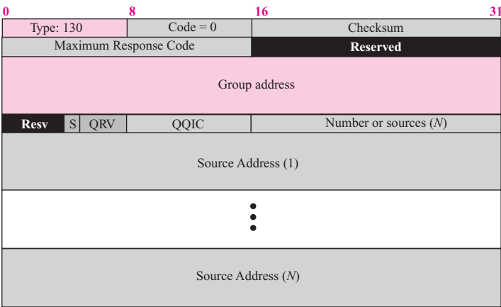
Figure 28.17 Membership-query message format
