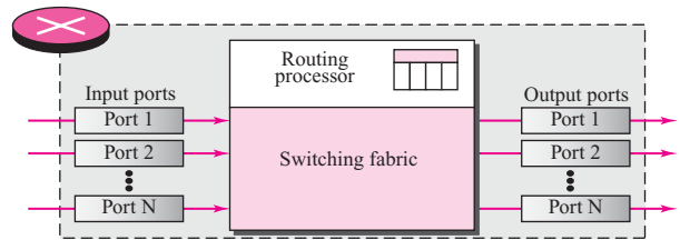
Figure 6.22 Router components
