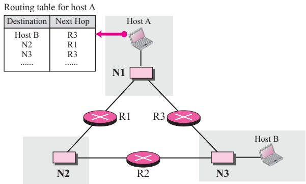
Figure 6.5 Host-specific routing
