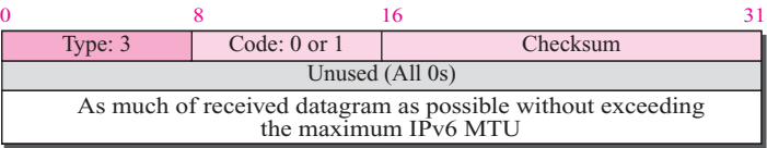
Figure 28.6 Time-exceeded message
