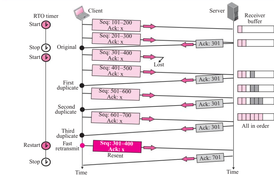
Figure 15.31 Fast retransmission
