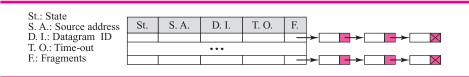
Figure 7.30 Reassembly table
