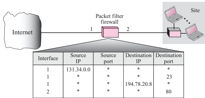
Figure 30.33 Packet-filter firewall
