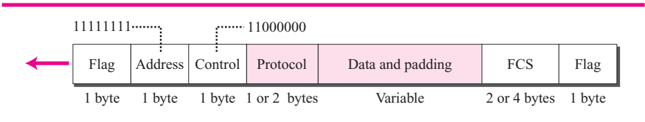
Figure 3.31 PPP frame
