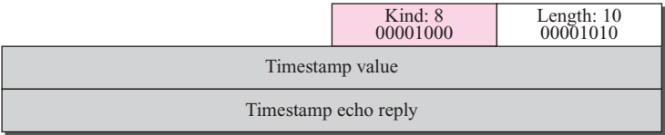
Figure 15.46 Timestamp option
