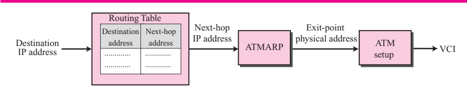
Figure 7.28 Address binding in IP over ATM
