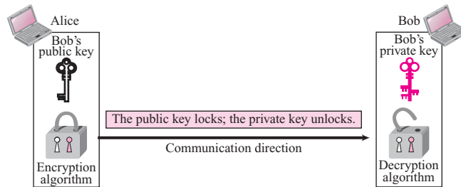
Figure 29.13 Locking and unlocking in asymmetric-key cryptosystem
