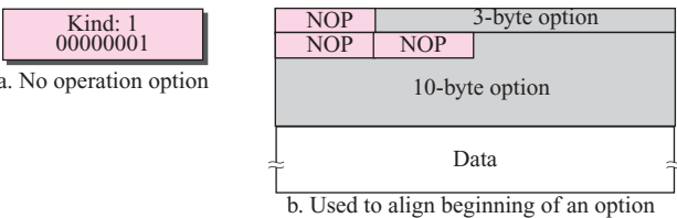
Figure 15.43 No-operation option
