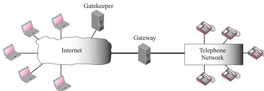
Figure 25.25 H.323 architecture
