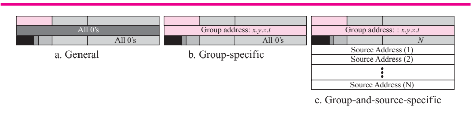
Figure 12.9 Three formats of query messages
