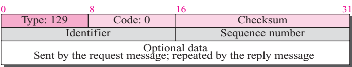
Figure 28.9 Echo-reply messages
