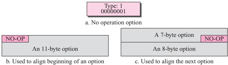
Figure 7.12 No operation option
