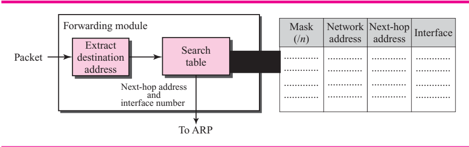
Figure 6.12 Simplified forwarding module in classless address
