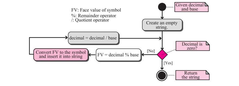
Figure B.6 Conversion from decimal to any base
