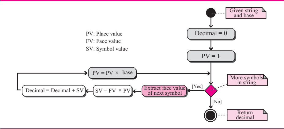
Figure B.5 Algorithm to convert from any base to decimal.
