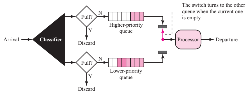
Figure 25.30 Priority queuing
