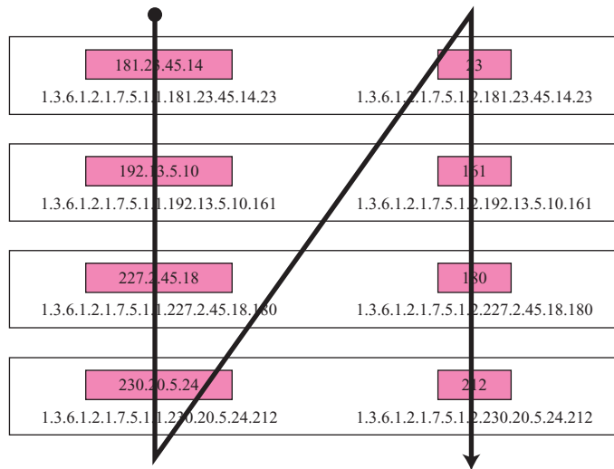
Figure 24.16 Lexicographic ordering
