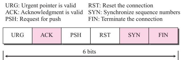
Figure 15.6 Control field
