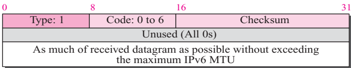
Figure 28.4 Destination-unreachable message
