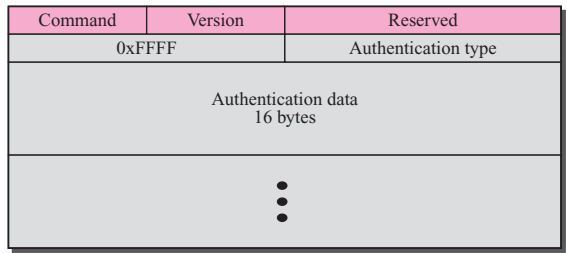
Figure 11.16 Authentication
