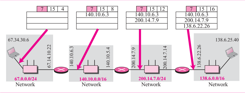
Figure 7.15 Record-route concept
