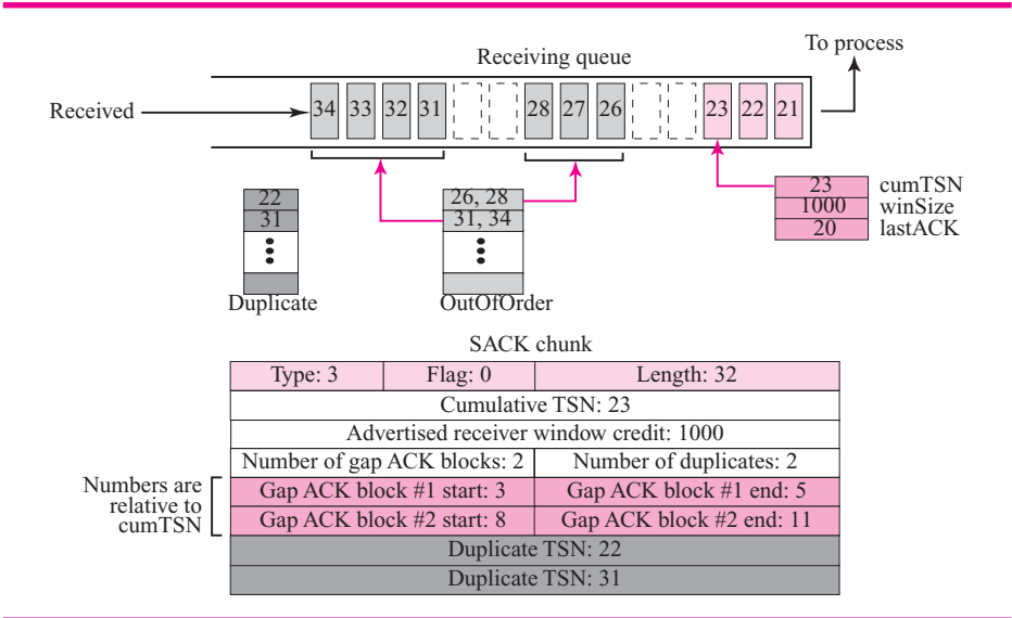
Figure 16.30 Error control, receiver site
