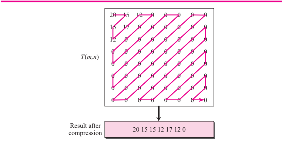
Figure 25.7 Reading the table
