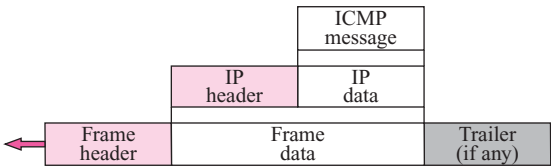
Figure 9.2 ICMP encapsulation
