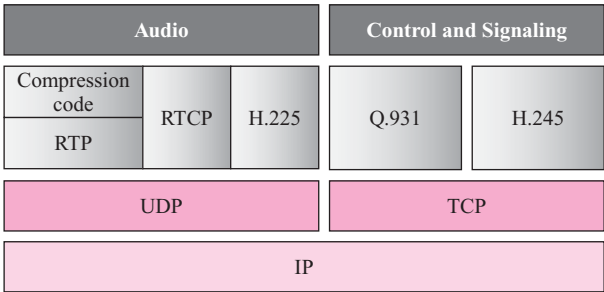
Figure 25.26 H.323 protocols
