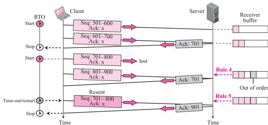
Figure 15.30 Lost segment
