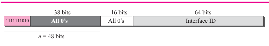
Figure 26.12 Link local address
