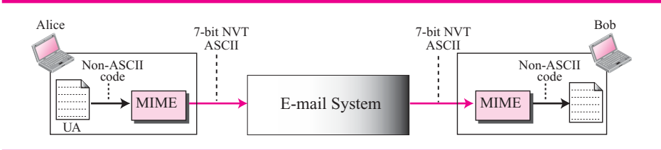
Figure 23.15 MIME
