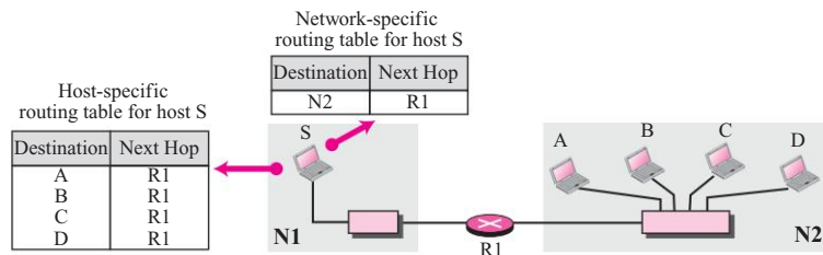
Figure 6.4 Network-specific method
