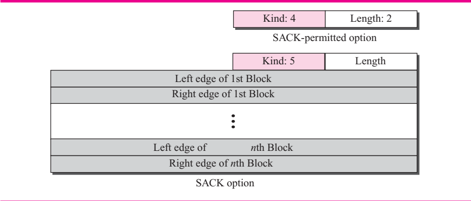
Figure 15.48 SACK
