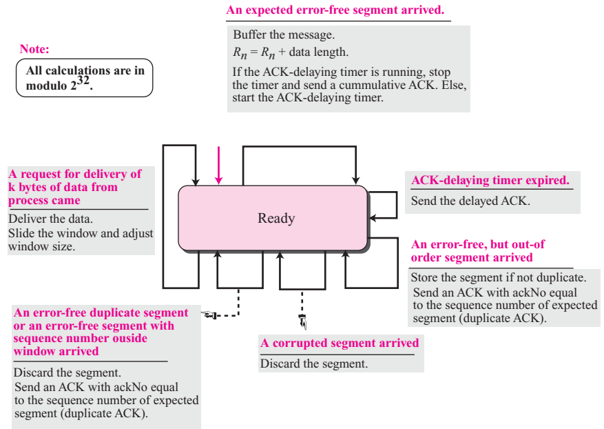
Figure 15.28 Simplified FSM for the TCP receiver side
