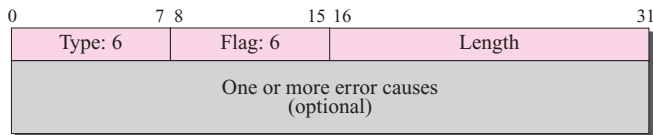
Figure 16.18 ABORT chunk
