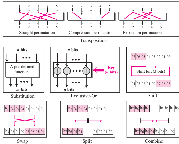
Figure 29.8 Components of a modern block cipher
