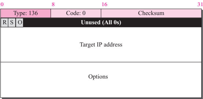
Figure 28.13 Neighbor-advertisement message
