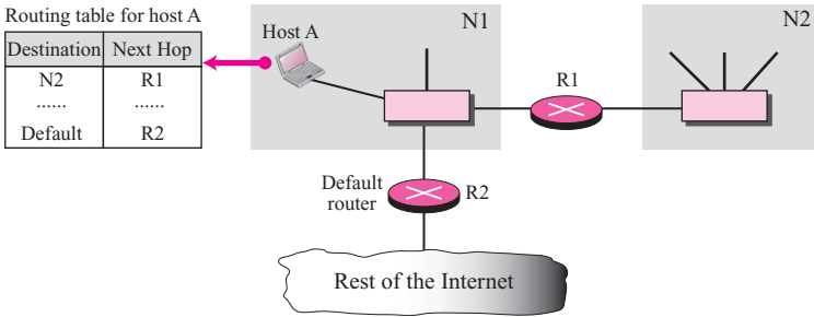
Figure 6.6 Default routing
