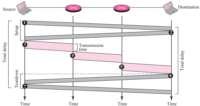
Figure 4.11 Delay in a connection-oriented network
