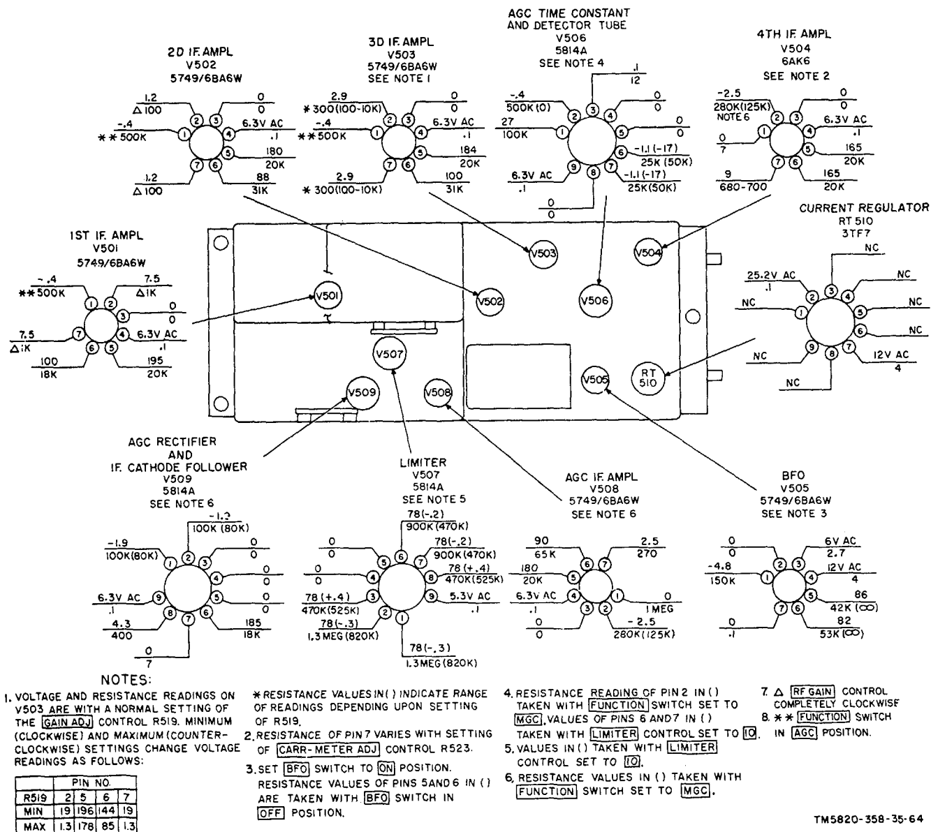
Figure 60. If. subchassis, voltage and resistance diagram.
