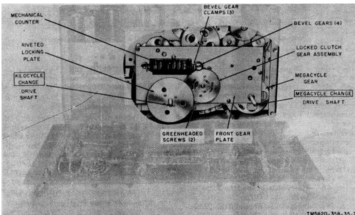
Figure 67. Rf gear train assembly, location of parts.
