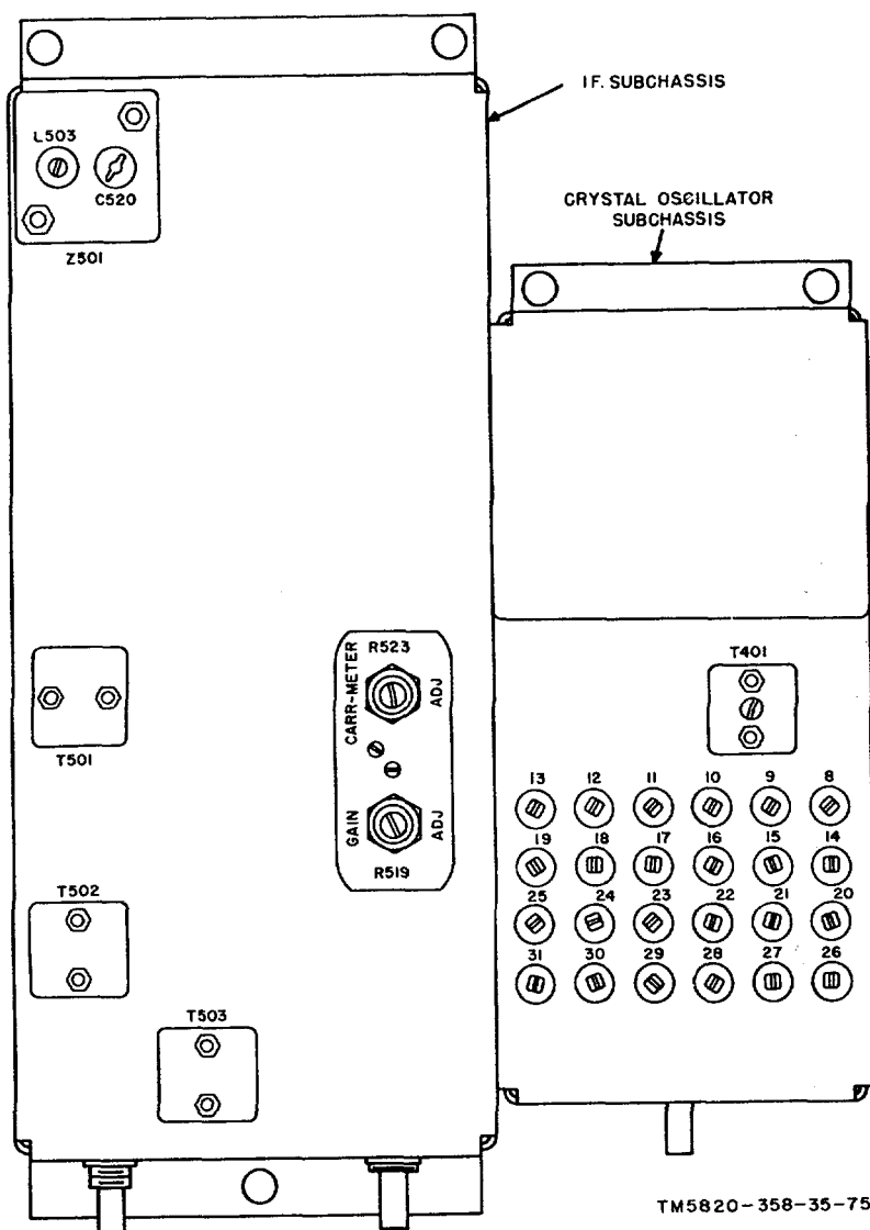
Figure 71. Crystal-oscillator and if. subchassis alignment points.
