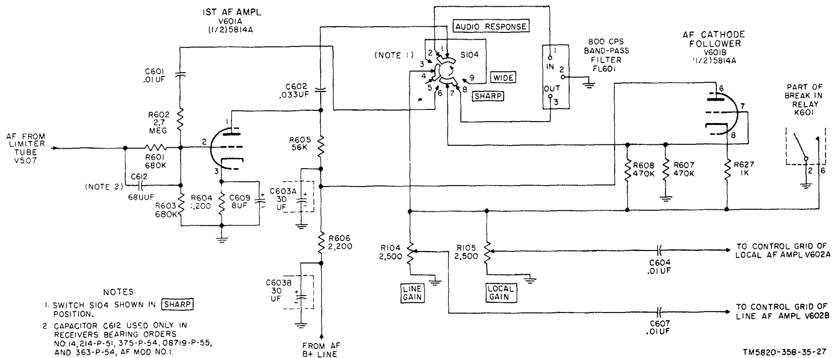
Figure 23. First af amplifier V601A and af cathode follower V601B, simplified schematic diagram.
