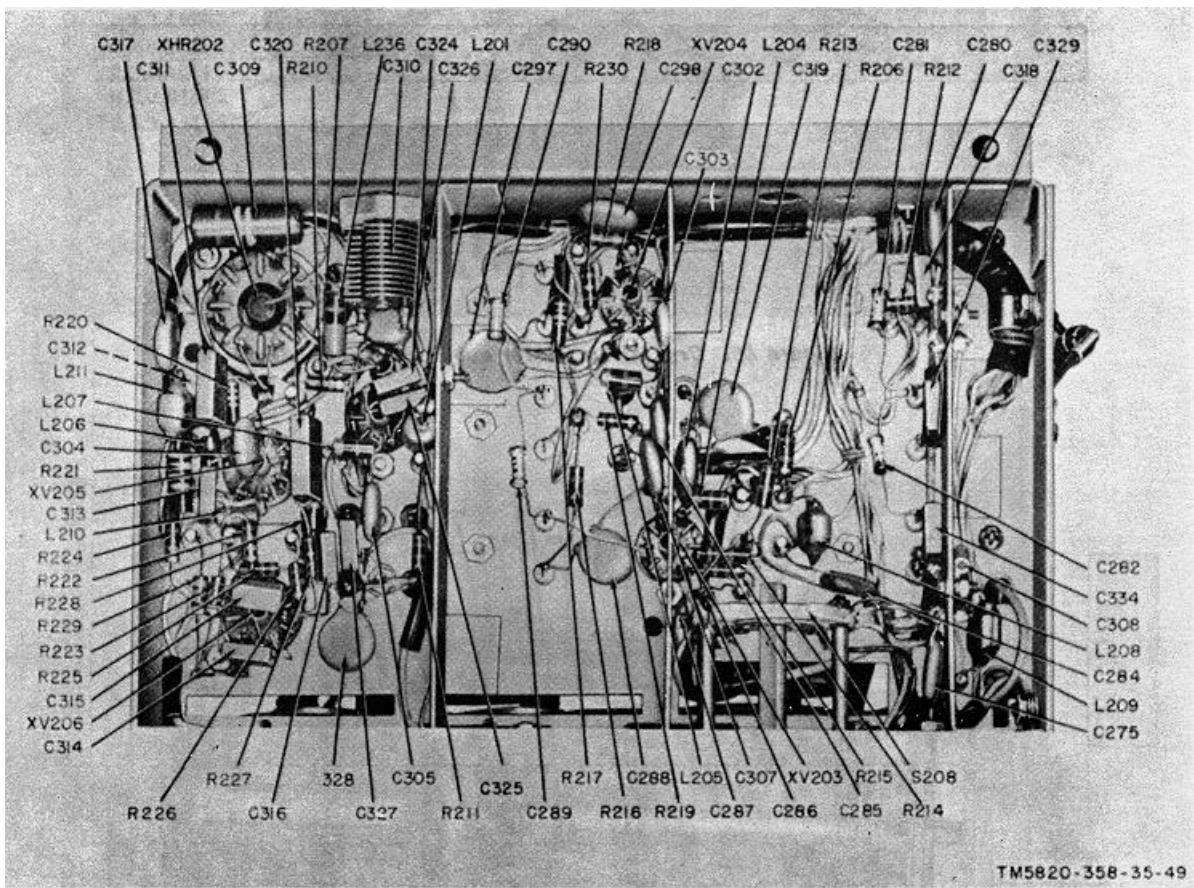
Figure 45. Rf subchassis, bottom view, rear section.
