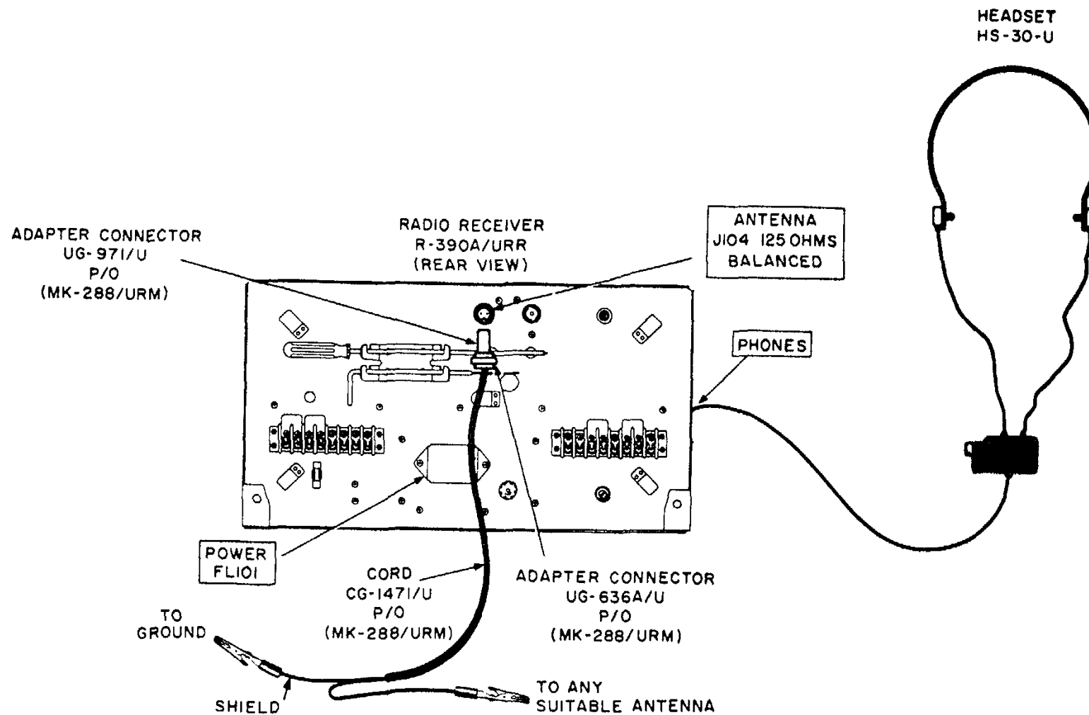
Figure 81. Operating tests setup.
