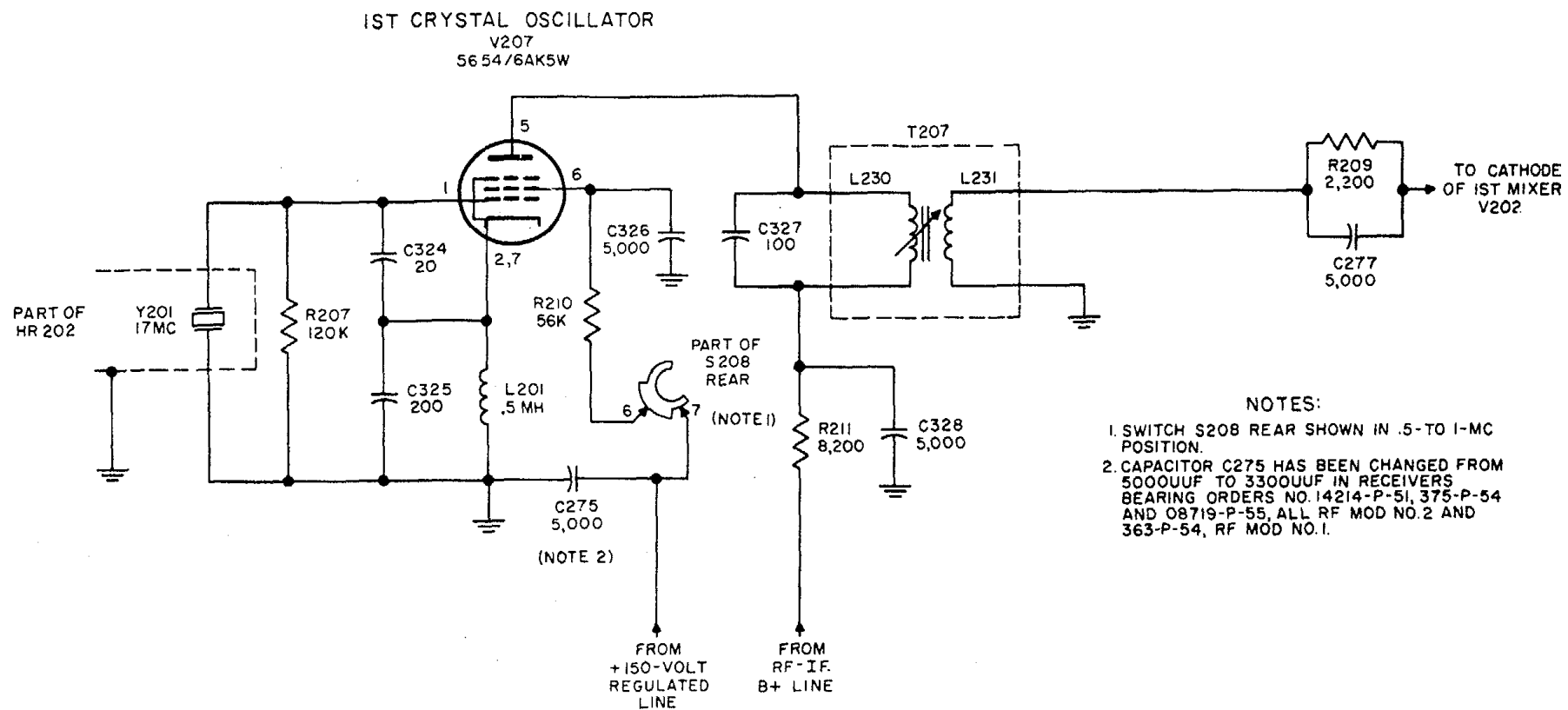
Figure 5. First crystal oscillator V207, simplified schematic diagram.
