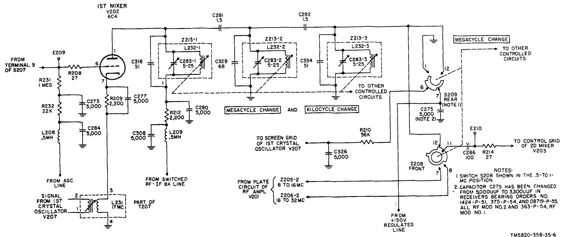
Figure 4. First mixer V202, simplified schematic diagram.
