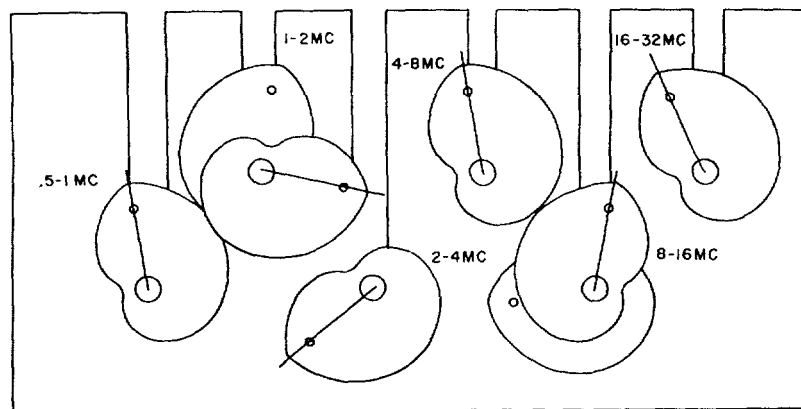
CAM POSITIONS VIEWED FROM REAR WITH 2 REAR PLATES REMOVED AND FREQUENCY INDICATOR SET AT 07 +000
