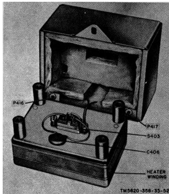
Figure 48. Crystal-oscillator subchassis, internal view of crystal oven.
