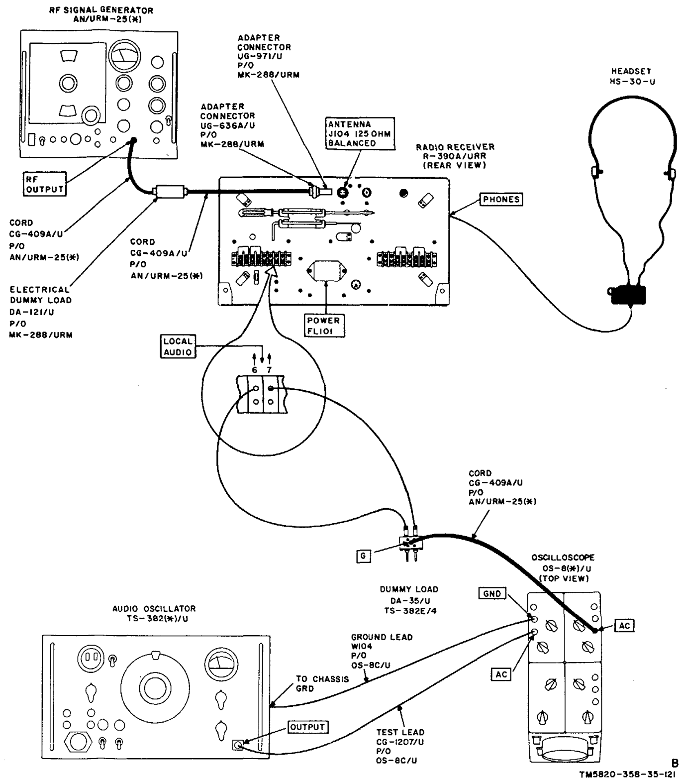
Figure 76. If. Output and bfo calibration test setup.
