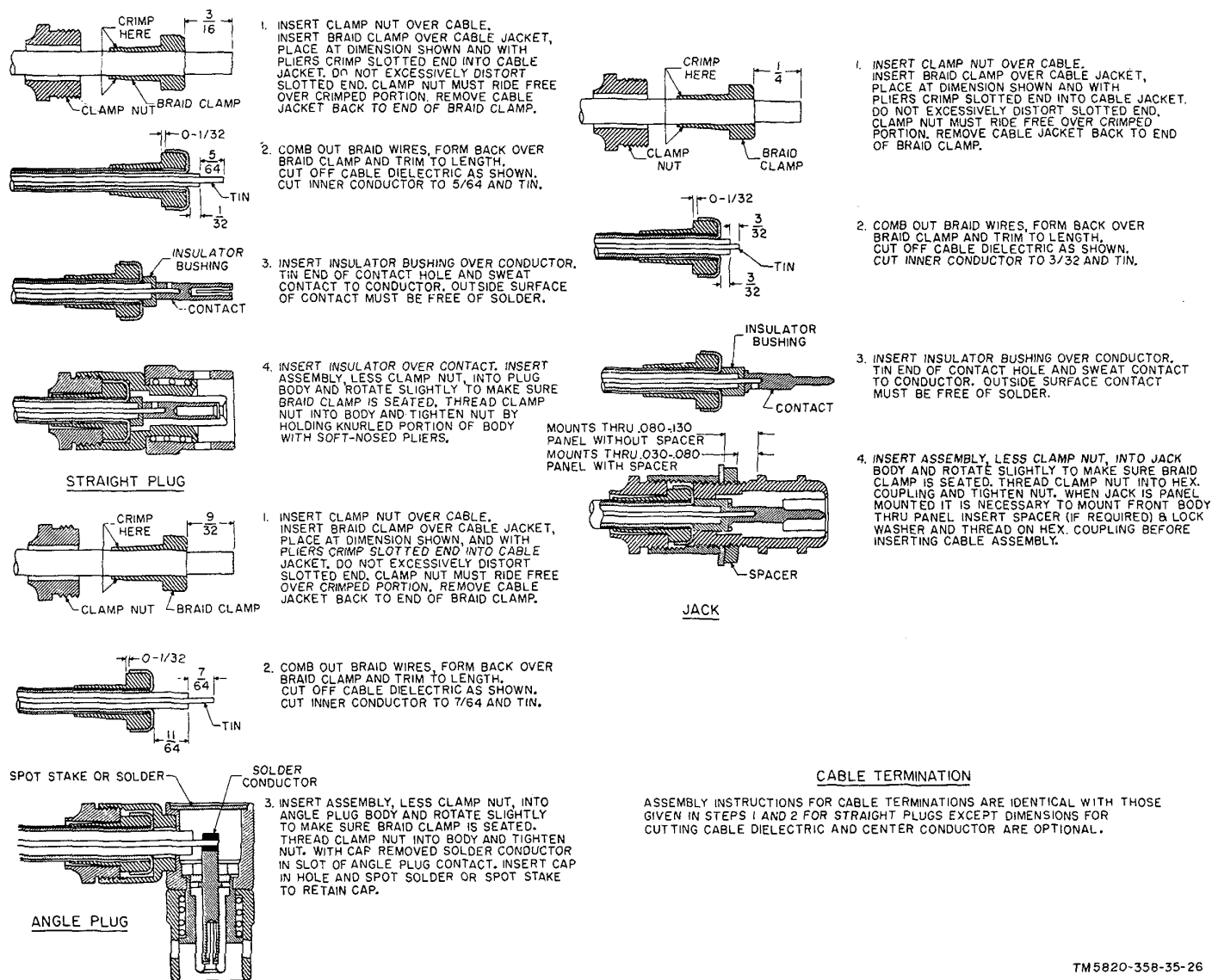
Figure 32. Fabrication of coaxial test cables.
