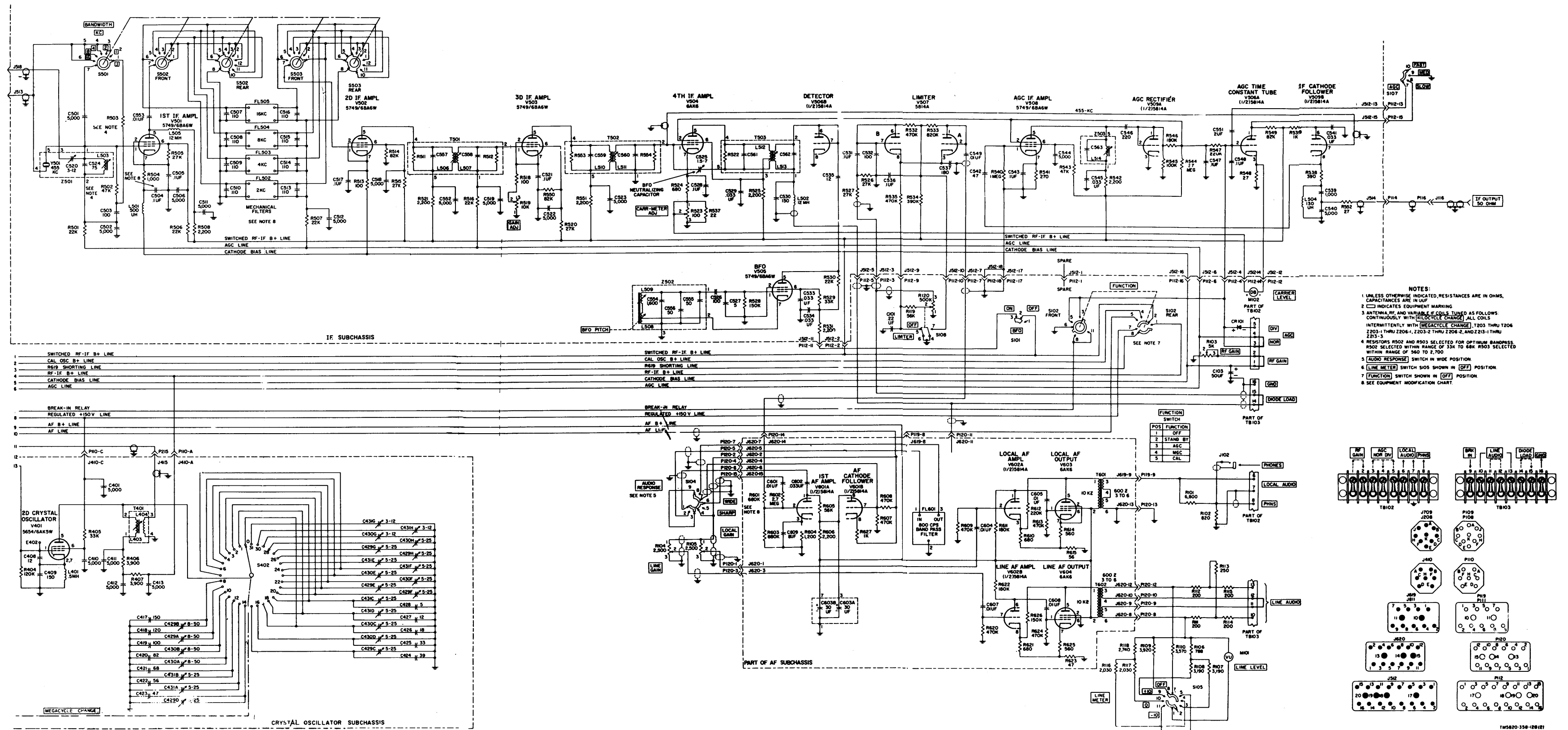
Figure 89 2. Radio Receiver R-390A/URR, main schematic diagram (part 2 of 2)
