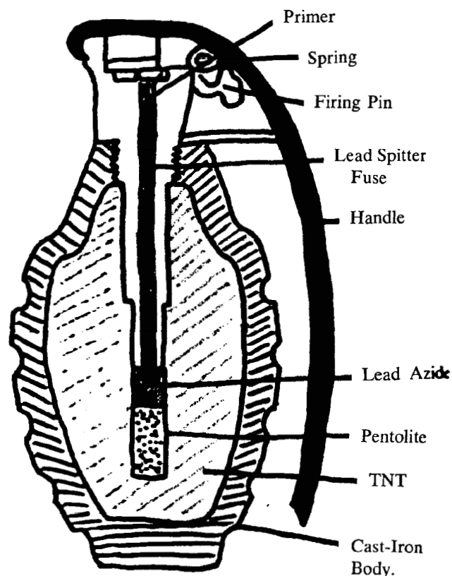
Figure 90. Military grenade.
