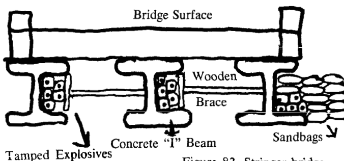
Figure 83. Stringer bridge.
