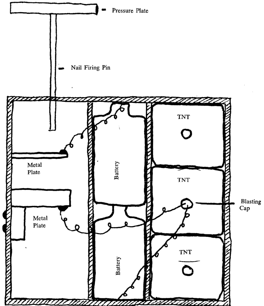
Figure 93. Pressure-plate detonator.
