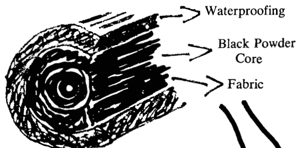
Figure 73. Safety fuse.
