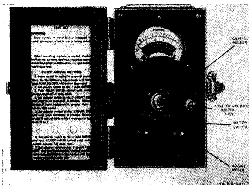
Figure 9. Crystal Rectifier Test Set TS-268D/U, front panel.
