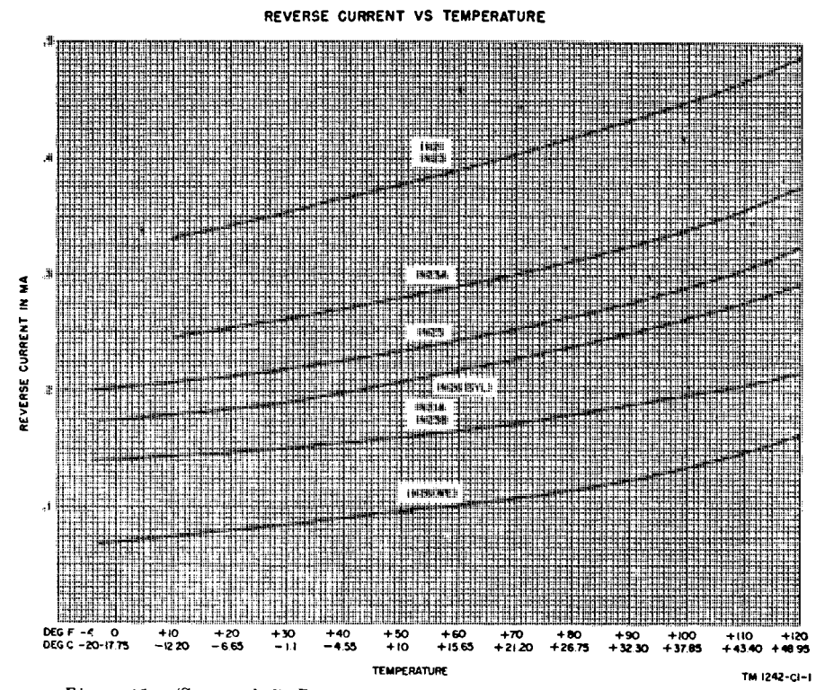
Figure 13. (Superseded) Reverse current versus temperature chart, showing allowable crystal limits of reverse current through the crystal
