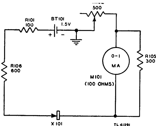
Figure 16. Circuit for forward resistance measurements, schematic diagram.
