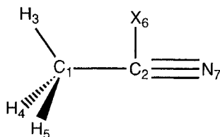
Figure D.3 Atom numbering for methyl cyanide including a dummy atom
