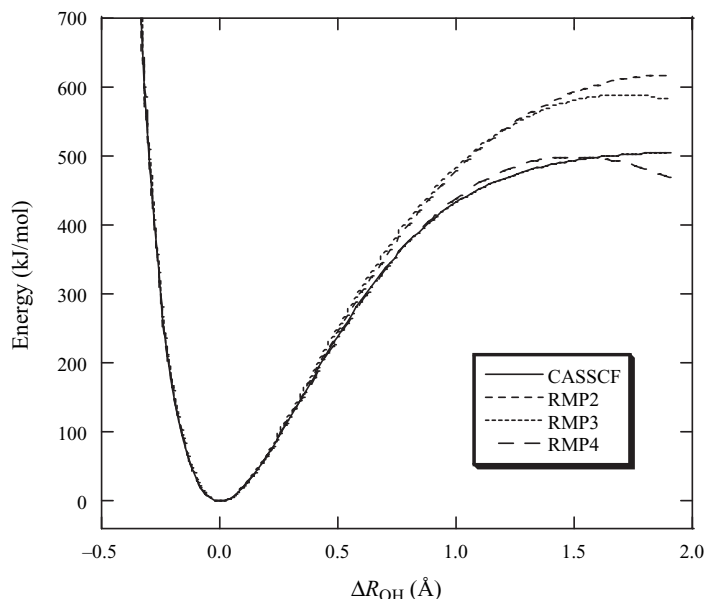
Figure 11.7 RMP2, RMP3 and RMP4 dissociation curves for \text{H}_2\text{O}
