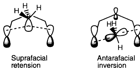
Figure 15.26 FMO interactions for allowed modes of the [1,5]-methyl shift in 1,3-hexadiene
