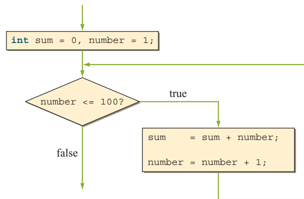
Figure 6.2 A diagram showing the control flow of a while statement.
