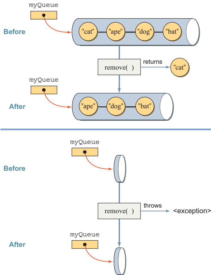
Figure 20.3 Sample remove operations on the myQueue queue.
