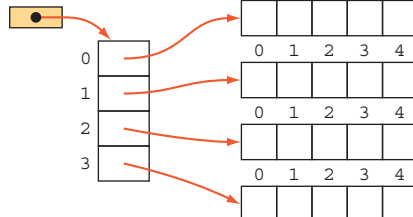
Figure 10.15 Executing the statements on the left in sequence will create the array of arrays shown on the right.
