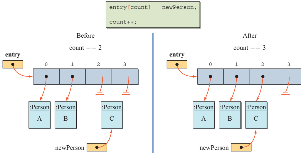
Figure 10.17 Adding a new Person object to the next available location. The array length is 4.
