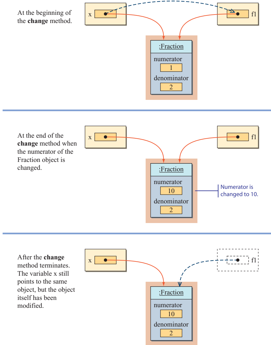
Figure 7.8 This illustration shows the effect of calling the change method.
