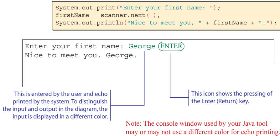
Figure 2.16 Sample interaction using System.in with Scanner and System.out . Keyboard input is echo-printed in the console window.
