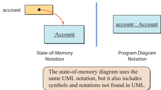
Figure 2.5 Relationship between the state-of-memory diagram and the program diagram notation.
