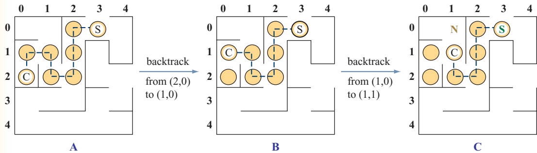
Figure 19.12 This illustrates how the backtracking works. Visited cells are marked with a red circle.
