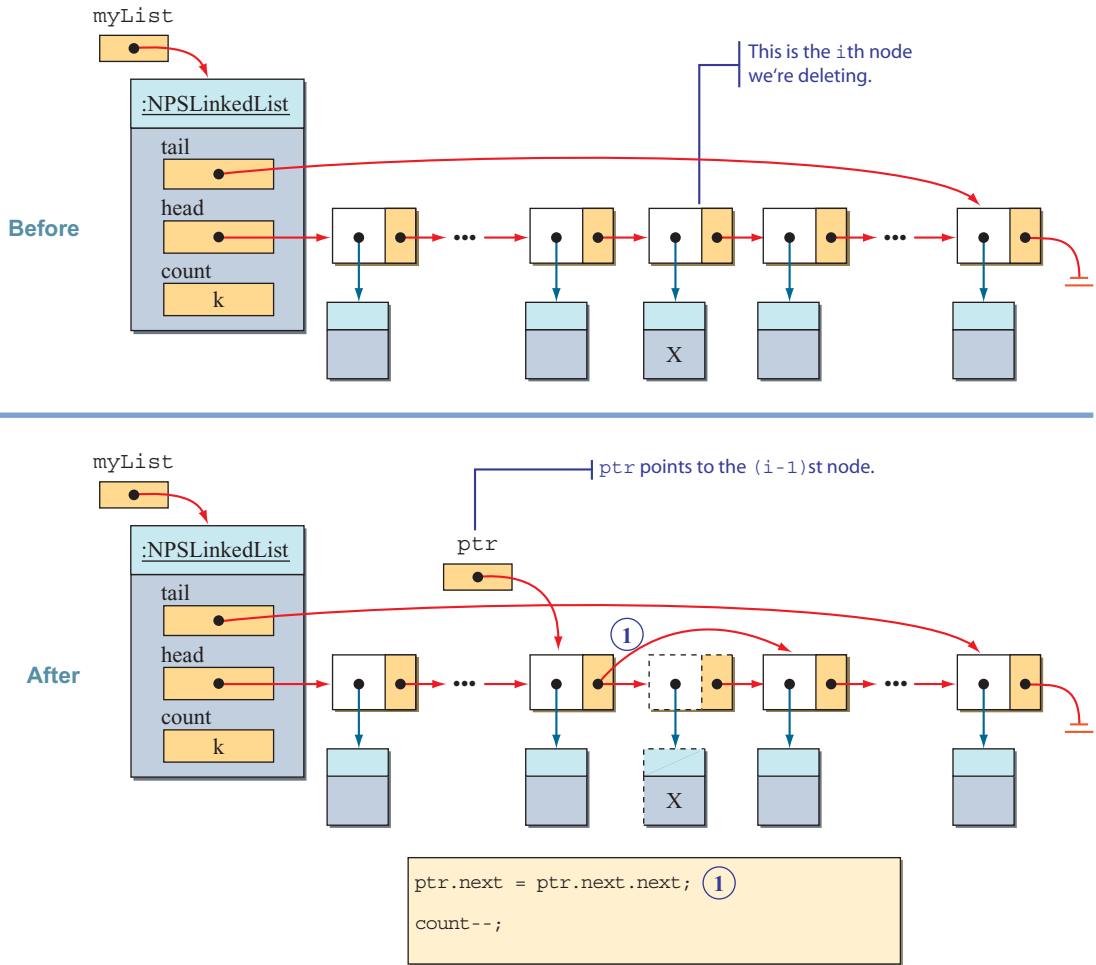
Figure 18.18 The first version of the remove operation. Remove the i th node given the value i .
