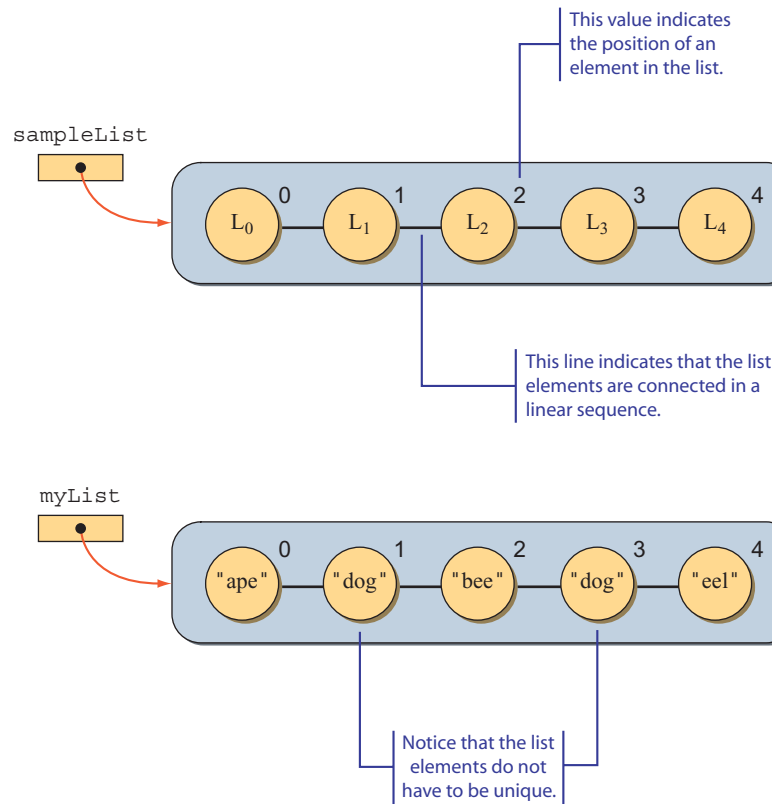
Figure 18.1 A generic list named sampleList with five elements and a list of three-letter animals, named myList .
