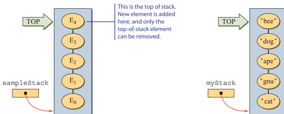
Figure 19.1 A generic stack sampleStack with five elements and a stack myStack with three-letter animal names.
