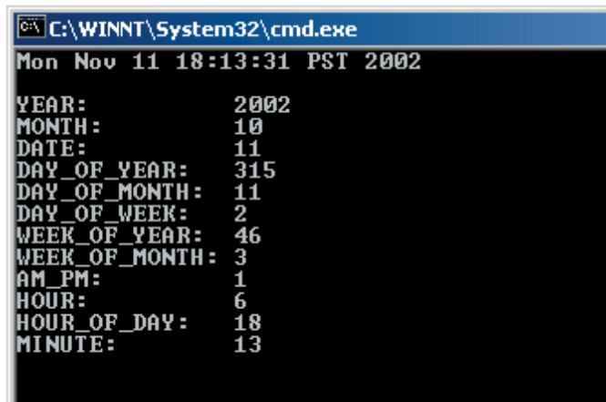
Figure 3.4 Result of running the Ch3TestCalendar program at November 11, 2002, 6:13 p.m.
