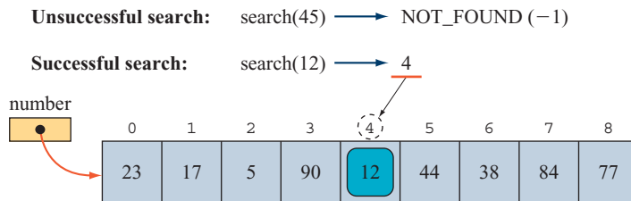
Figure 11.1 Successful and unsuccessful searches.
